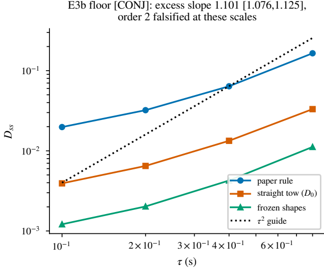
Fig. 9. Numerical evidence for the conjectured stochastic steady-state floor ([ES §10(ii)]); Theorem 7.2 is leading-order and deterministic and is tested in Fig. 6. Fitted excess exponent 1.101 [1.076, 1.125]: the conjectured order 2 is excluded (and so is 1); the frozen+noise-off regression reproduces the executed null ( D_{ss} \sim 10^{-30} ).
