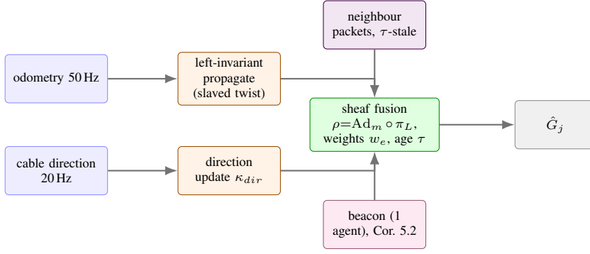
LOCAL sensing (odometry, cable direction) · \tau -stale SHARED neighbour estimates on the graph · one ABSOLUTE beacon at one agent (nothing else touches truth — linted).
