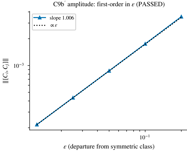
Fig. 14. Symmetry, the amplitude object (C9b'): the departure from the symmetric class is first-order in \epsilon (slope 1.006), the base commutator exactly zero — PASSED.
