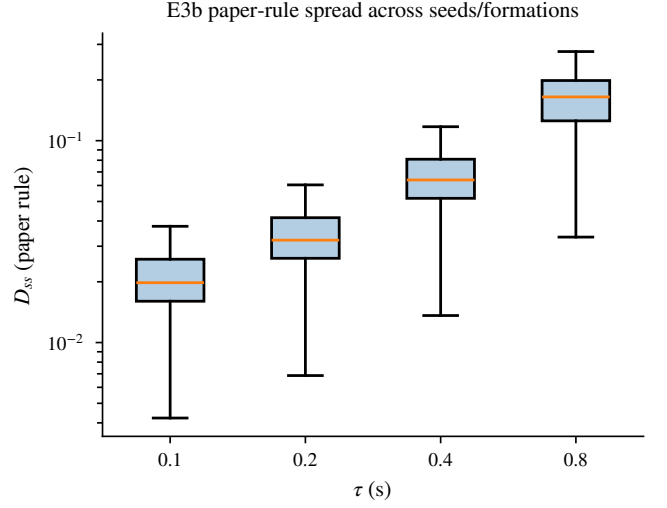
Fig. 11. Paper-rule D_{ss} spread across seeds and formations per \tau ([[CONJECTURAL] regime]).
