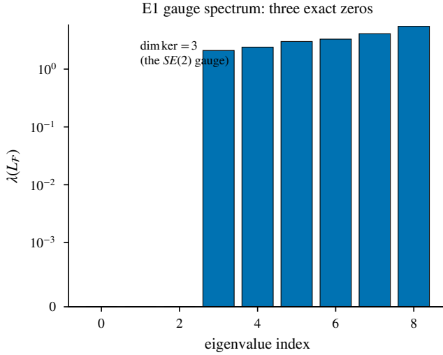
Fig. 3. Gauge spectrum: \dim \ker L_F = 3 without an anchor, collapsing to zero with one anchor whose \lambda_{\min} becomes the rate. (The harmonic-section identity — kernel = body-framed images of one common load-frame perturbation — is the 1.3 \times 10^{-15} annihilation check reported in the text.)
