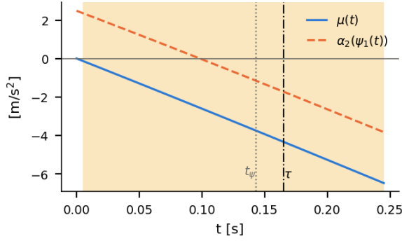
Fig. 4. HOCBF feasibility margin in a perfect-actuator trial. The feasible-to-infeasible transition occurs before a cable can enter the braking half-space.
