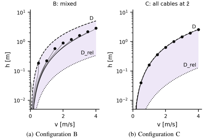
Fig. 10. Viability bands for (a) mixed cable directions and (b) cables already behind the payload; curves and dots as in Fig. 9.
