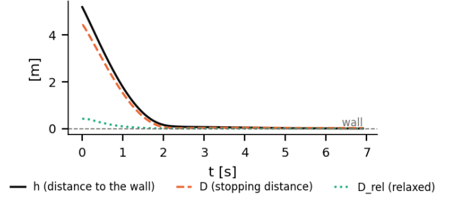
Fig. 6. Wall distance h (solid), predicted stopping distance D (dashed), and optimistic stopping distance D^{\text{rel}} (dotted) in a perfect-actuator trial under an adversarial nominal command. The trial illustrates the continuous-time maneuver but does not prove sampled safety.
