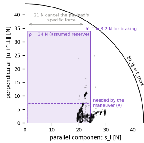
Fig. 11. Thrust budget of one vehicle: the reserved rectangle lies in the available thrust ball.
