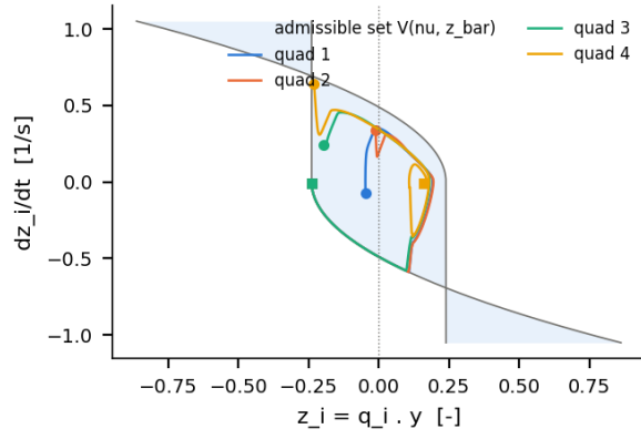
Fig. 8. Swing states (z_i, \dot{z}_i) in the trial of Fig. 6 (circle: start; square: end); the shaded region is the admissible swing set \mathcal{V} .
