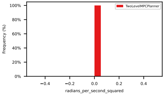
abs_ego_yaw_acceleration_within_bounds
