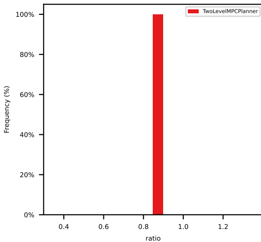
ego_expert_progress_along_route_ratio
