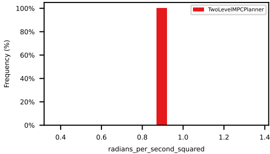
avg_ego_yaw_acceleration
