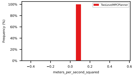
abs_ego_lon_acceleration_within_bounds
