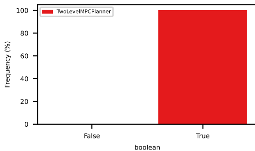
abs_ego_lon_acceleration_within_bounds
