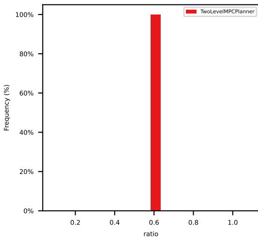
ego_expert_progress_along_route_ratio
