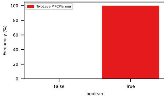
abs_ego_lat_acceleration_within_bounds
