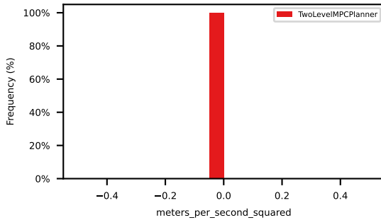
abs_ego_lat_acceleration_within_bounds
