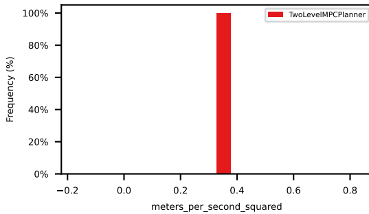
abs_ego_lon_acceleration_within_bounds
