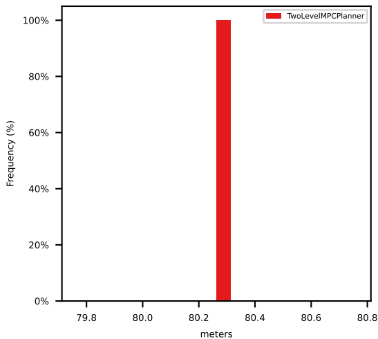
ego_total_progress_along_route
