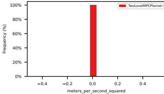
avg_ego_lat_acceleration
