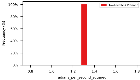
avg_ego_yaw_acceleration
