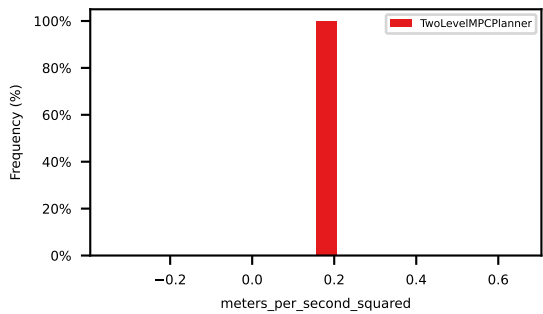
abs_ego_lon_acceleration_within_bounds
