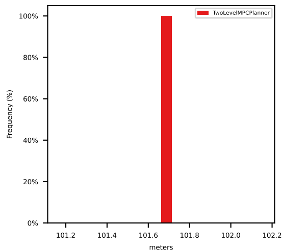
ego_total_progress_along_route
