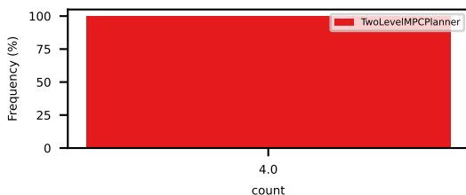
min_collision_energy_with_objects
