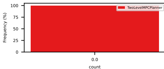
max_collision_energy_with_objects
