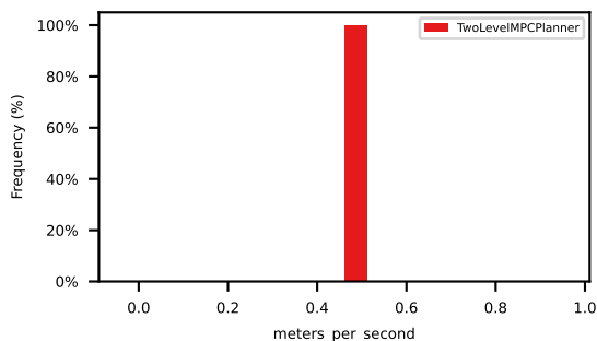
mean_violation_of_speed_limit_compliance
