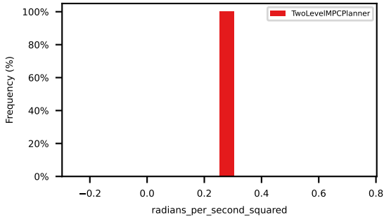
avg_ego_yaw_acceleration
