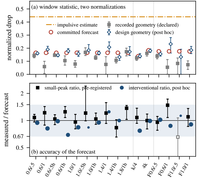
Fig. 4. Transmission in sixteen cells, labeled by T_0 in kN and weather intensity (h: doubled heading gain; F: fan; k/4 , 4k : stiffness cells). (a) Declared recorded-geometry statistic (squares) and post hoc design-geometry reading (diamonds), with seed intervals, against the committed forecast (circles). (b) Measured over forecast: pre-registered small-peak ratio (squares, seed intervals; open: unscored cell) and post hoc interventional ratio (circles, area growing with observation count); the band is the declared factor 1.5.
