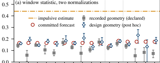
(a) window statistic, two normalizations
