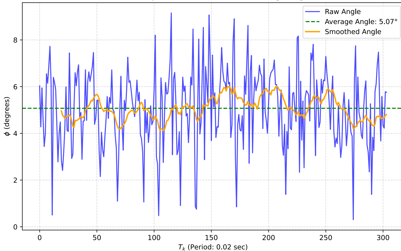
Line Plot of "Exp 1: LQR with fork" with Average Angle 5.07°
