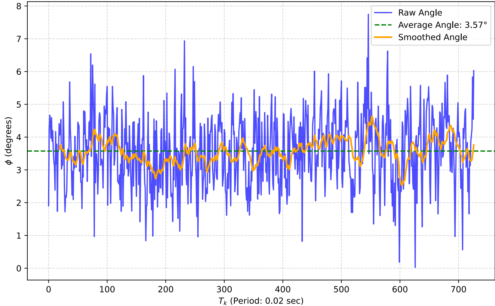
Line Plot of "Exp 2: LQR without fork" with Average Angle 3.57°
