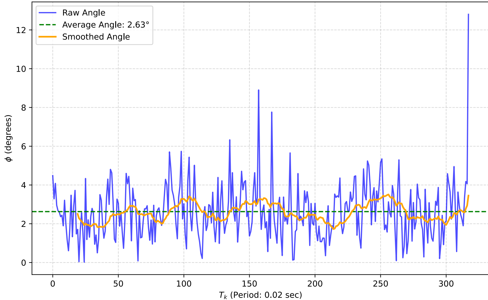
Line Plot of "Exp 4: DDFB without fork angle target_angle=2.0" with Average Angle 2.63°
