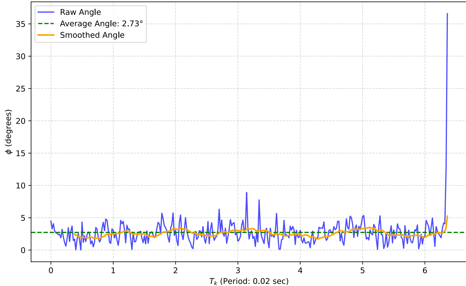
Line Plot of "Exp 4: DDFB without fork angle target_angle=2.0" with Average Angle 2.73°
