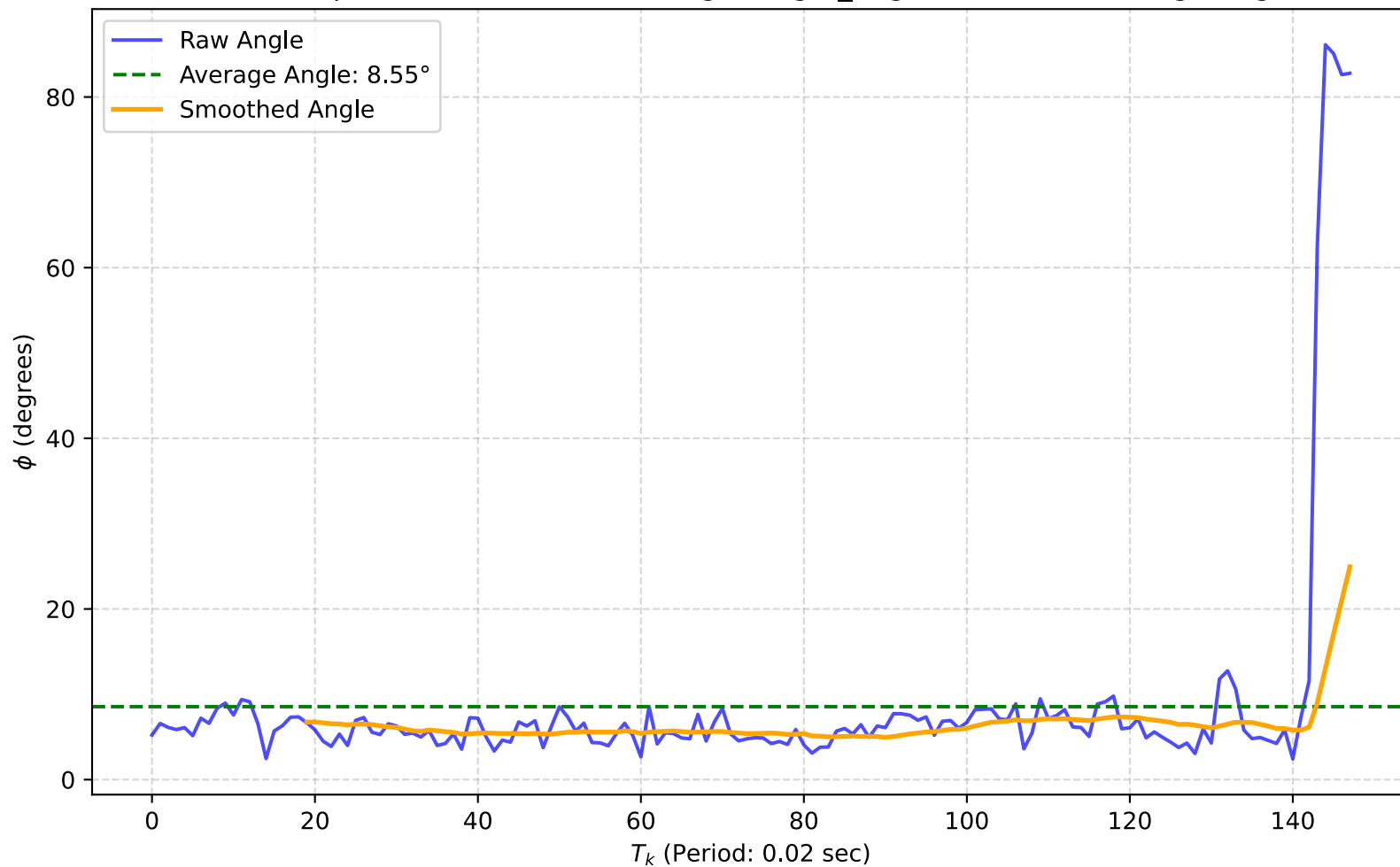
Line Plot of "Exp 4: DDFB without fork angle target_angle=4.9" with Average Angle 8.55°
