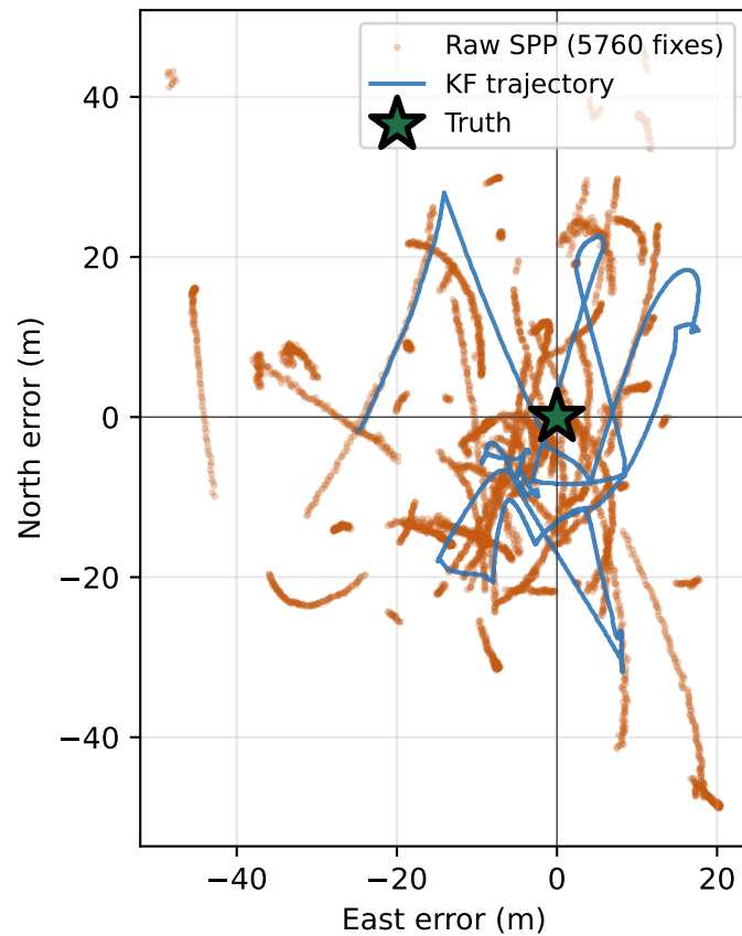
Error Distribution Comparison
