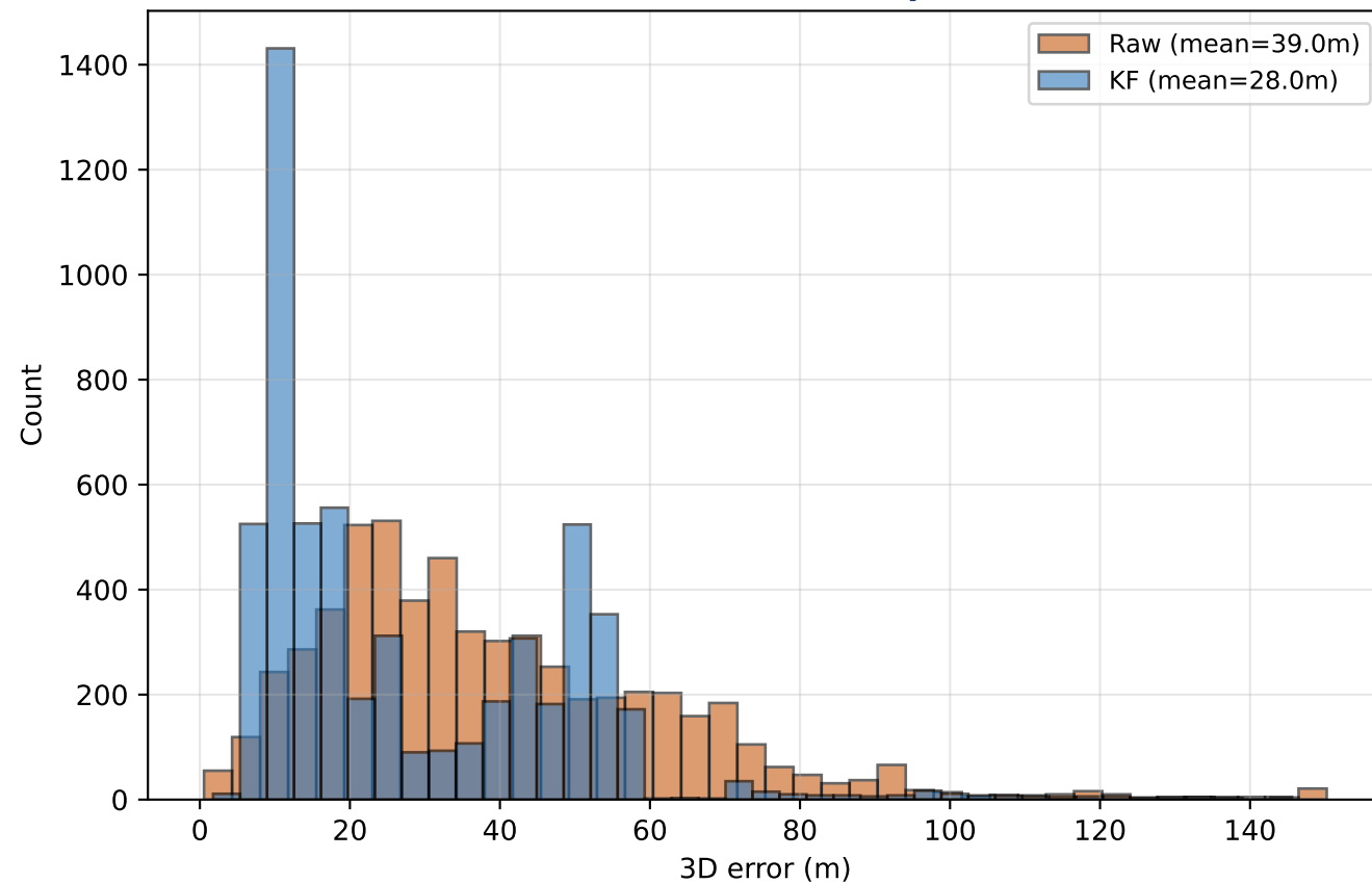
Error Distribution Comparison
