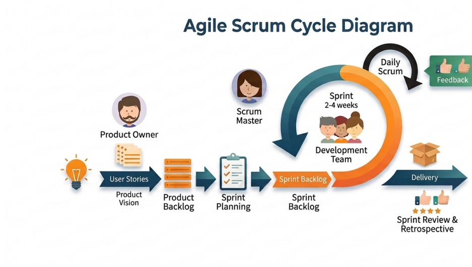
FIGURE 1.6 – processus Scrum.
