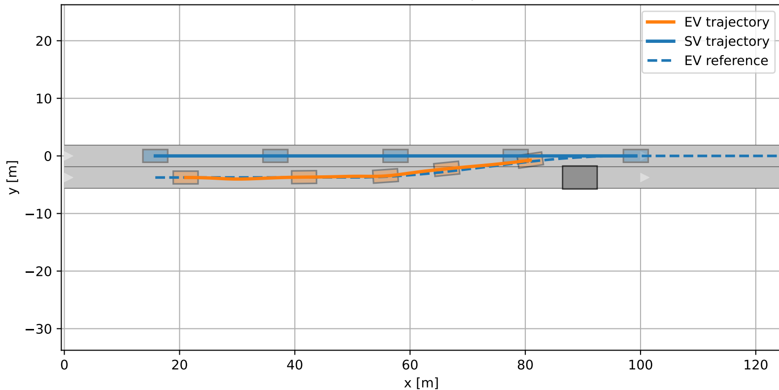
EV-SV Interaction under Non-Cooperative SV Behavior
