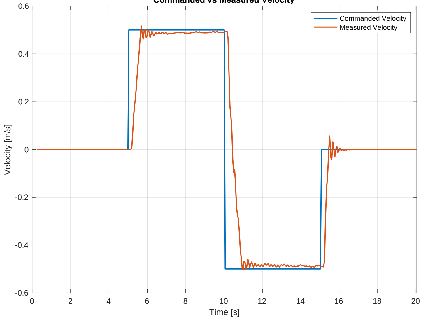
Commanded vs Measured Velocity
