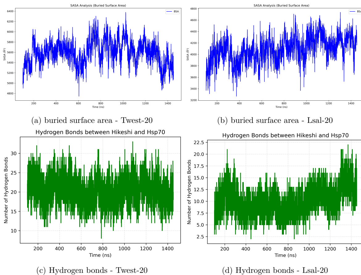
Figure 3: (A) Buried surface area (BSA) of Twist-20 and Lsal-20 at 20 °C , (B) the number of hydrogen bonds between them.
