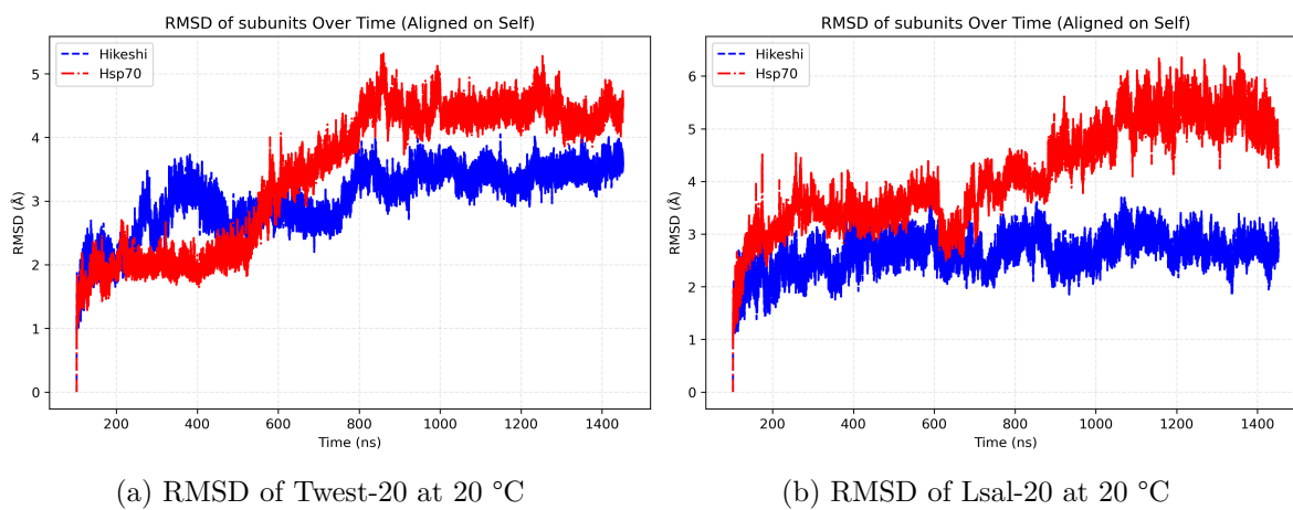
Figure 5: RMSD of CA for Twist-20 and Lsal-20 at 20 °C .
