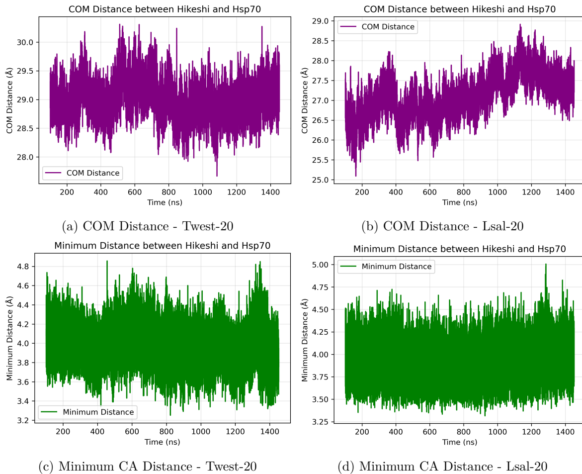
Figure 1: (A) Distance between the center of mass (COM) of Twist-20 and Lsal-20 at 20 °C , (B) and the minimum distance between any two atoms of the complexes.
