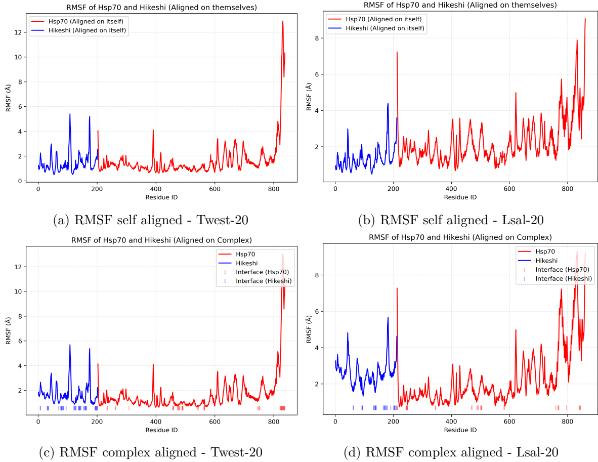
Figure 4: (A) RMSF of CA for Twest-20 and Lsal-20 at 20 °C aligned to their own reference structure, (B) RMSF of CA for Twest-20 and Lsal-20 at 20 °C aligned to the reference structure of the complex.
