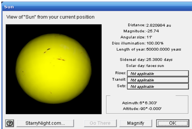
StarryNight Backyard 3.12 – Sun Info Window
