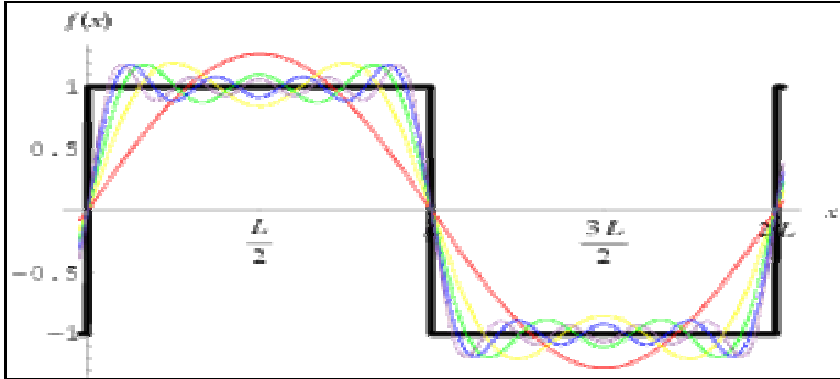
Fourier approximation of a Square into an infinite series of sine waves
