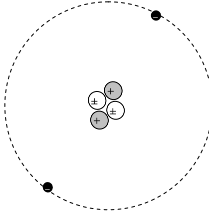
Helium Atom ( {}^2\text{He} - isotope {}_4\text{He} )
