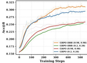
(a) Acc@8
