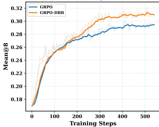
Mean@8
