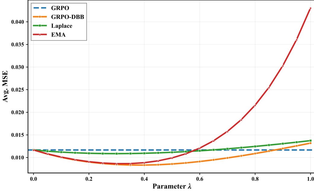
Figure 6. MSE versus \lambda for per-prompt exponential moving average (EMA), per-prompt Laplace smoothing, the GRPO point estimator (horizontal dashed line), and GRPO-DBB. DBB attains the lowest minimum MSE at \lambda = 0.4 and improves on the point estimator over a broader range of \lambda than EMA or Laplace.
