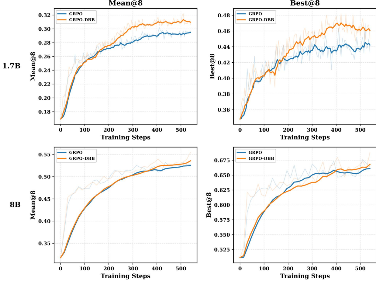
Figure 5. Validation performance of Qwen3-1.7B-Base (top) and Qwen3-8B-Base (bottom) trained with GRPO and GRPO-DBB. The left column shows Mean@8 (= Acc@8) and the right column shows Best@8 on the validation set. Despite producing lower entropy during training, GRPO-DBB matches or exceeds GRPO in Best@8 across both model scales.
