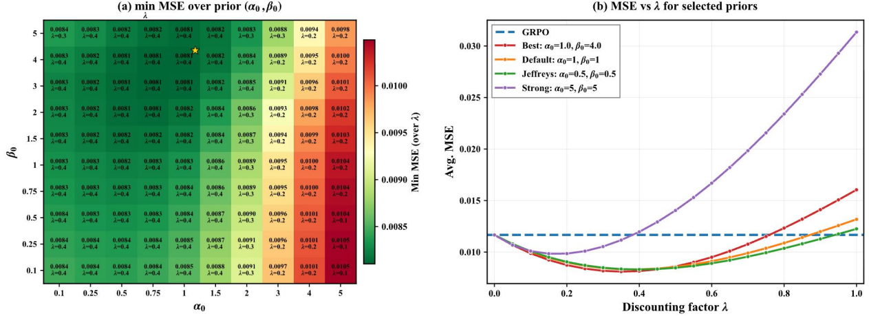
Figure 7. (a) Heatmap of \min_{\lambda} MSE of the DBB estimator over (\alpha_0, \beta_0) . (b) MSE versus \lambda for selected priors. The default symmetric prior (\alpha_0, \beta_0) = (1, 1) is competitive with the best prior and robust over a wide range of \lambda .
