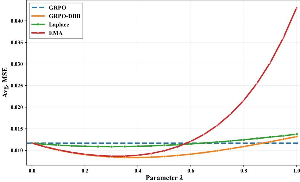
Figure 7. MSE versus \lambda for per-prompt exponential moving average (EMA), Laplace smoothing (Laplace), point estimator (GRPO), and DBB estimator (GRPO-DBB). DBB estimator attains the lowest minimum MSE at \lambda = 0.4 and improves on the point estimator over a broader range of \lambda than EMA or Laplace.
