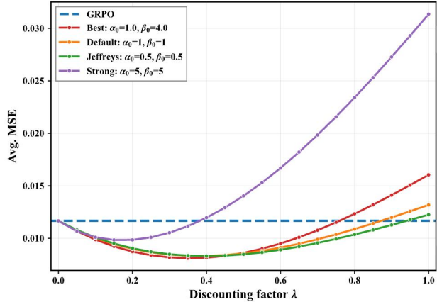
(b) MSE vs \lambda for selected priors
