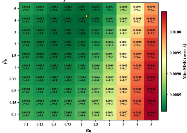
(a) min MSE over prior (\alpha_0, \beta_0)
