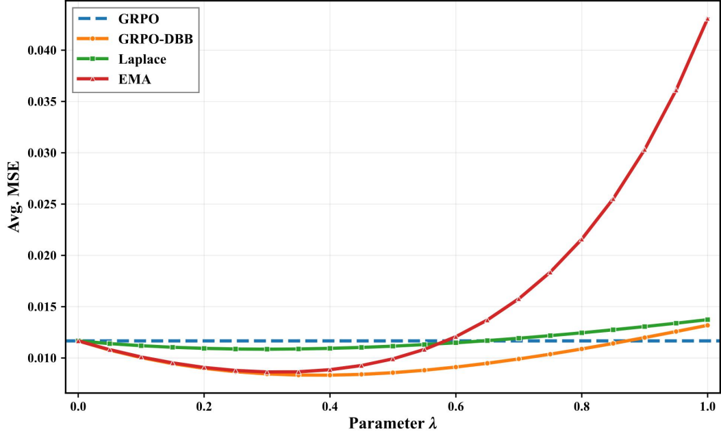
Figure 7. MSE versus \lambda for per-prompt exponential moving average (EMA), per-prompt Laplace smoothing, the GRPO point estimator (horizontal dashed line), and GRPO-DBB. DBB attains the lowest minimum MSE at \lambda = 0.4 and improves on the point estimator over a broader range of \lambda than EMA or Laplace.
