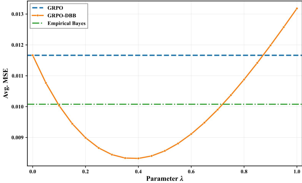
Figure 8. MSE versus \lambda for the empirical Bayes (EB) estimator (online method-of-moments), the GRPO point estimator (dashed), and GRPO-DBB. EB improves over the point estimator without per-prompt tuning, but DBB attains a lower minimum MSE.
