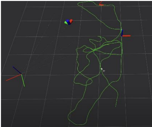
Relocalization failure
