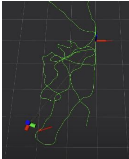
Relocalization success
