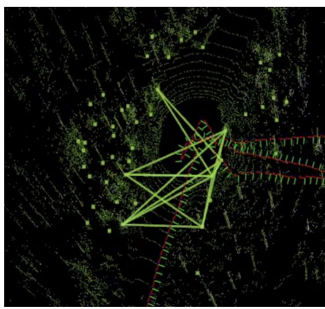
STD
