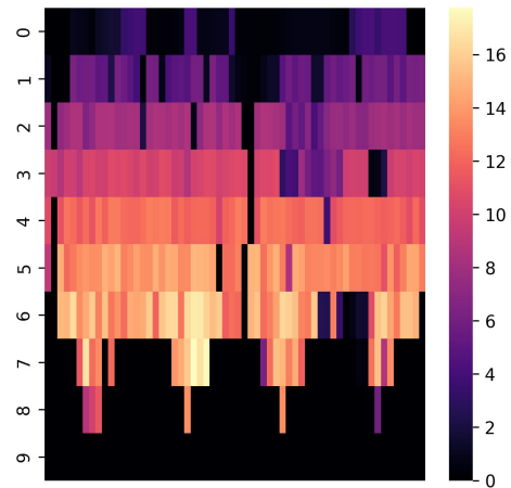
Scan Context
