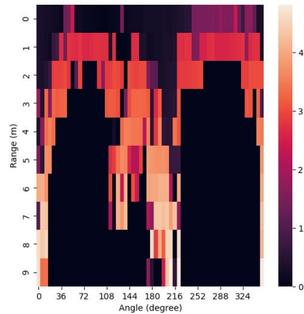
Scan Context
