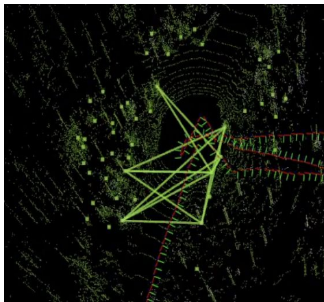
STD
