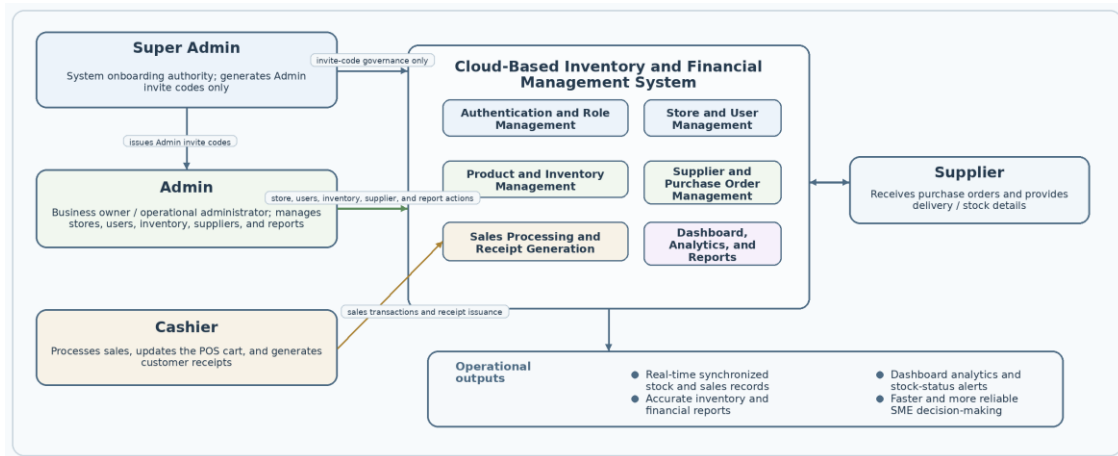
Figure 3.2. Conceptual Framework of the Kodigo System
