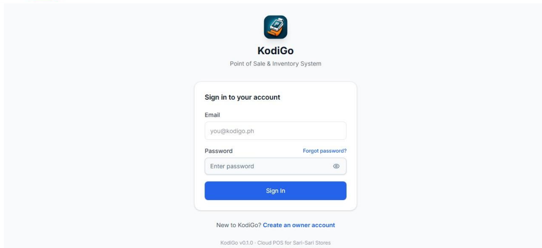
Figure 3.7. Login Page
