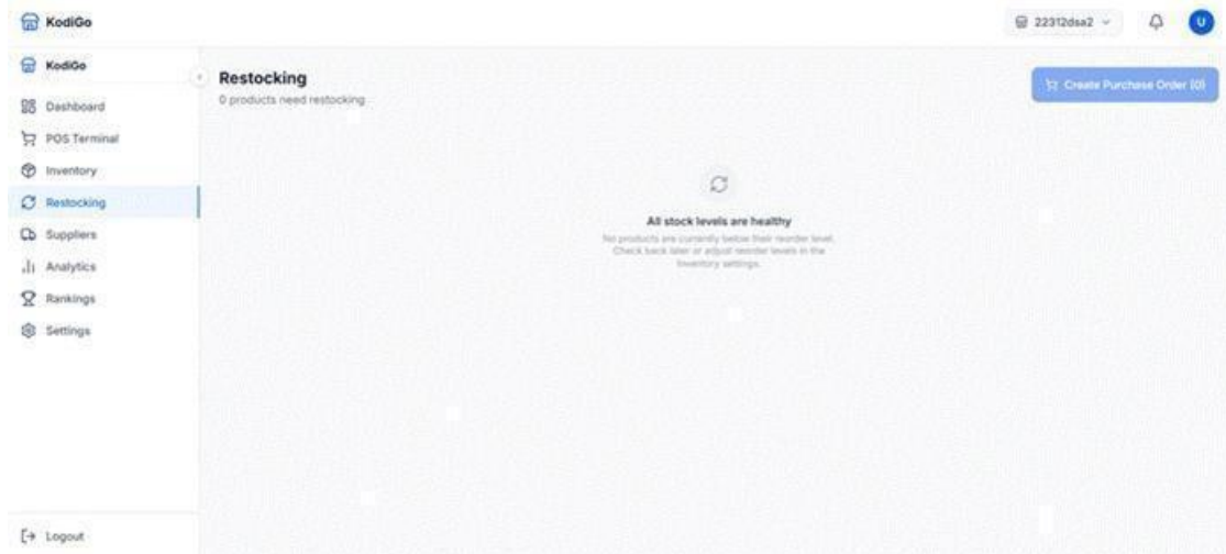
Figure 3.18. Restocking Page
