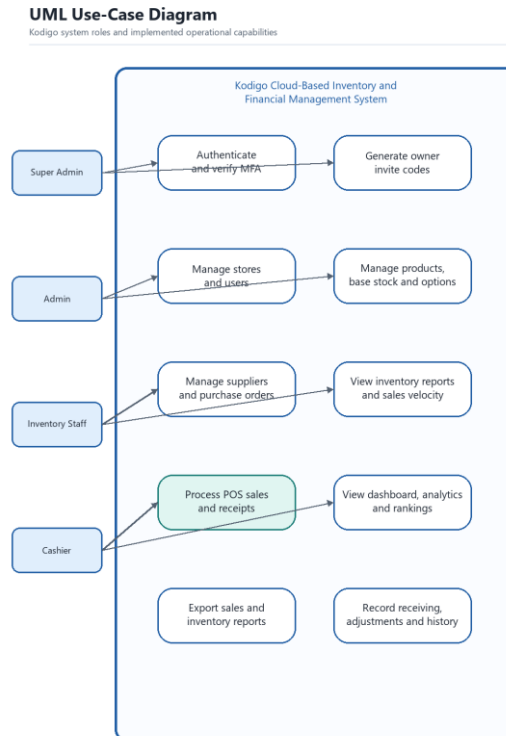
Figure 3.3. UML Use-Case Diagram of the Kodigo System
