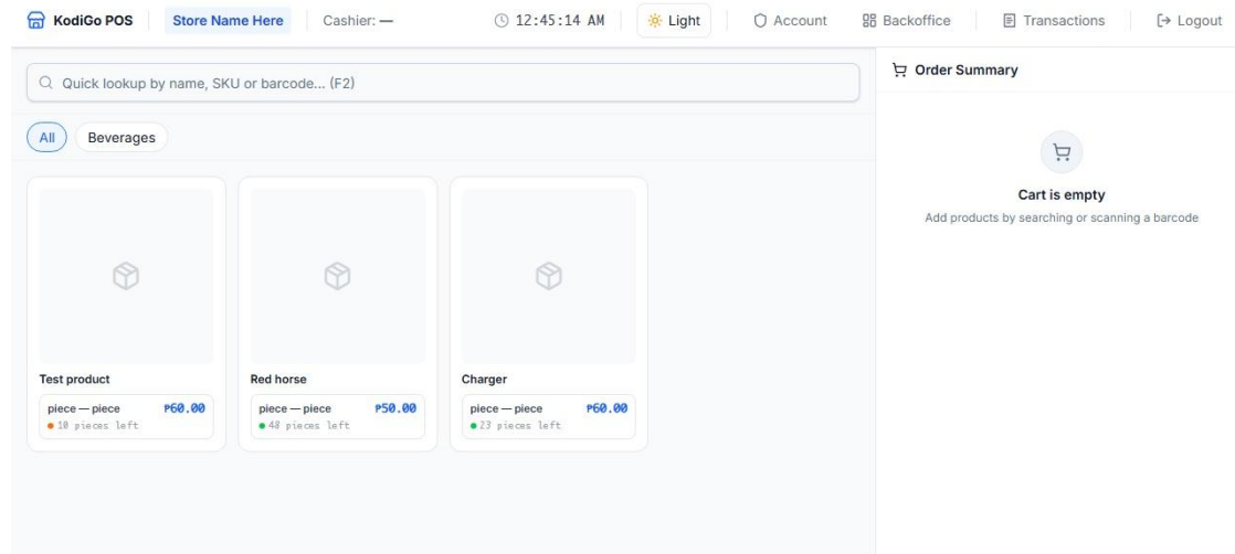
Figure 3.19. Point-of-Sale Page
