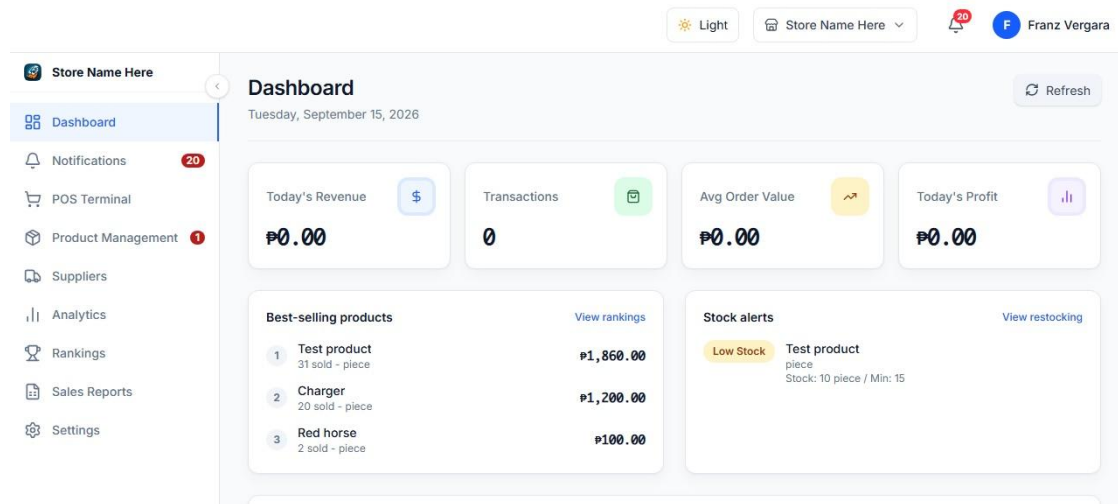
Figure 3.13. Dashboard Page
