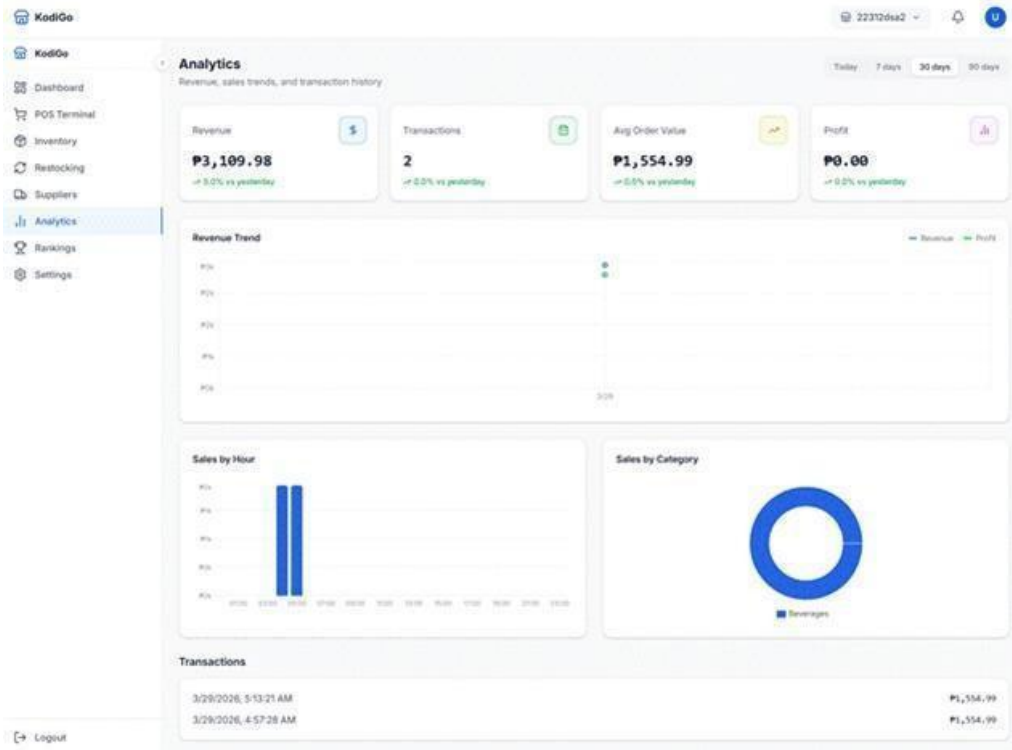
Figure 3.20. Analytics Page
