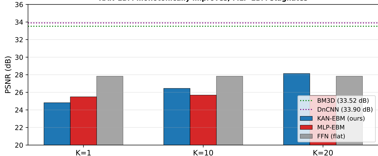
CBSD68 denoising ( \sigma=15/255 , in-distribution training) KAN-EBM monotonically improves; MLP-EBM stagnates
