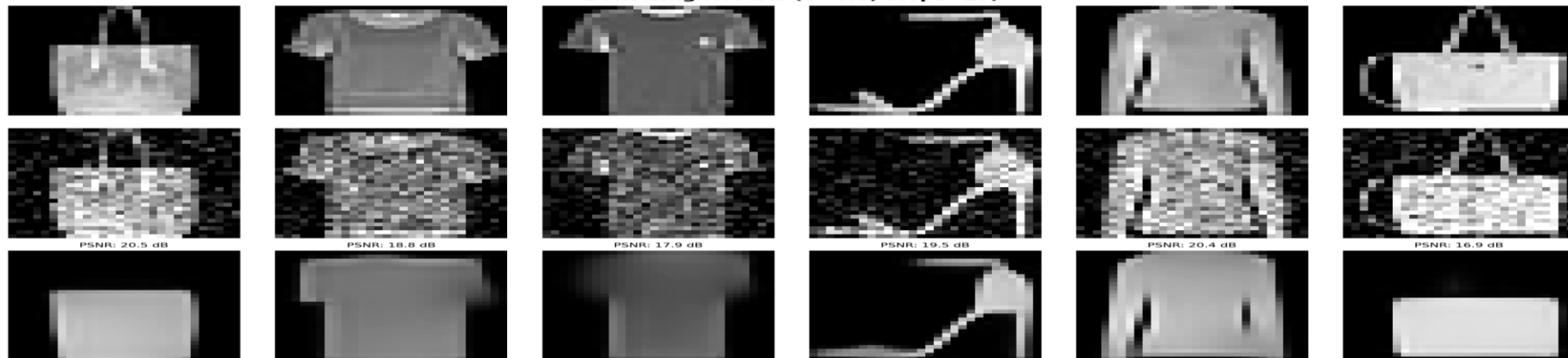
Denoising Results ( \sigma=0.3 , steps=10)
