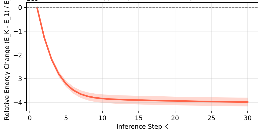
Relative Energy Drop (shows convergence rate)
