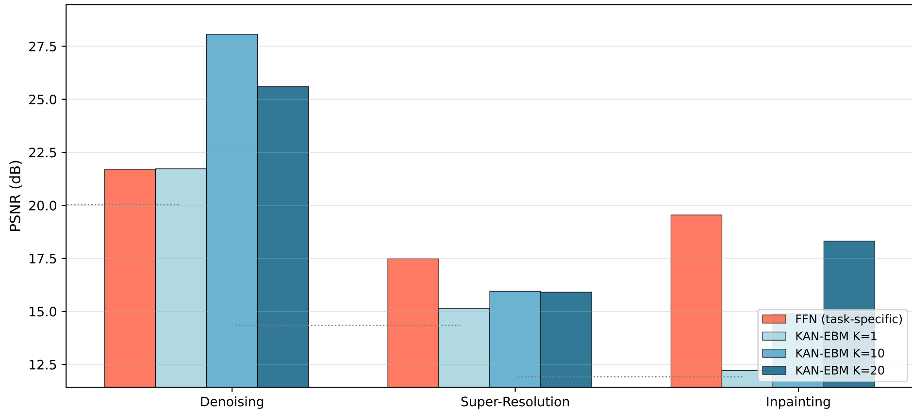
Multi-Task Restoration: FFN (task-specific) vs KAN-EBM (single model) KAN-EBM matches or exceeds FFN at K=10+ without task-specific training
