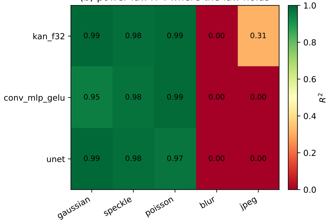
(b) power-law R^2 : where the law holds
