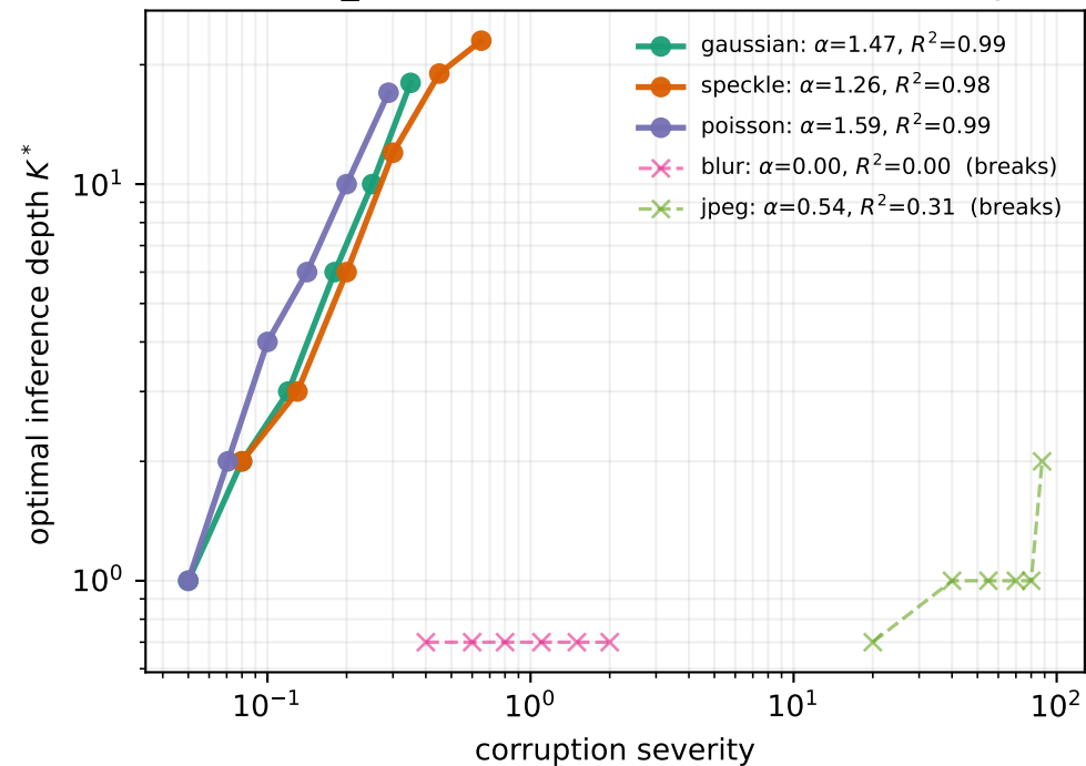
(a) kan_f32: law holds for additive noise only
