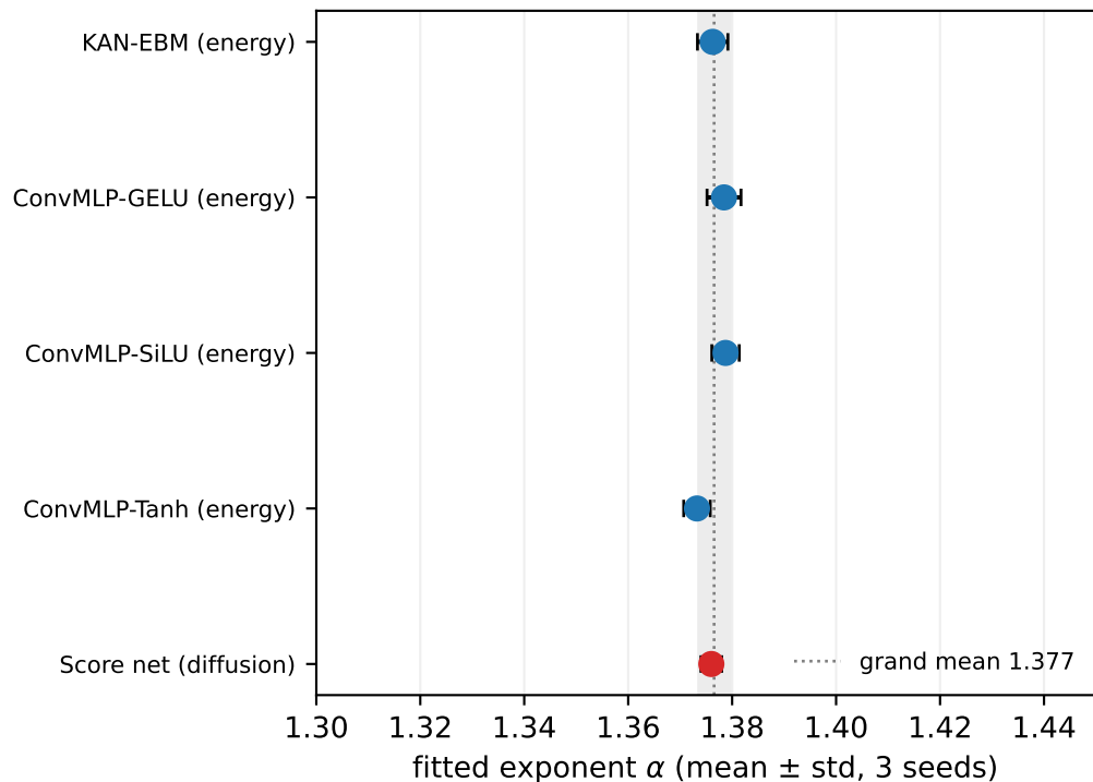
(b) \alpha indistinguishable across models ( F = 0.79 )
