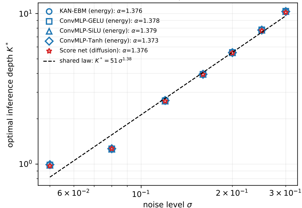
(a) All denoisers collapse onto one law
