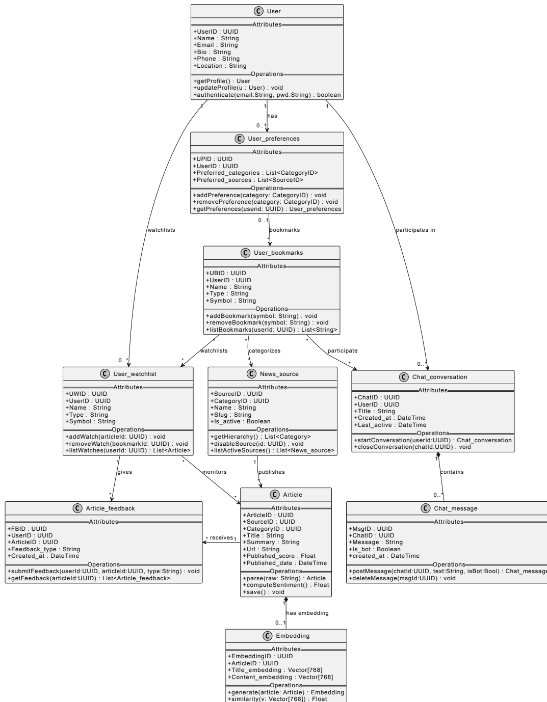
Figure 6.6: Class Diagram
