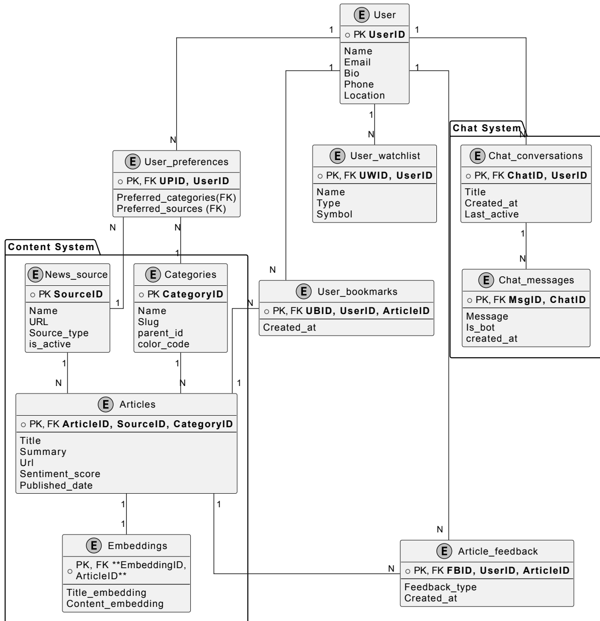
Figure 4.9: Entity Relationship Diagram for Quantum Entity Relationship model showing database structure and table connections
