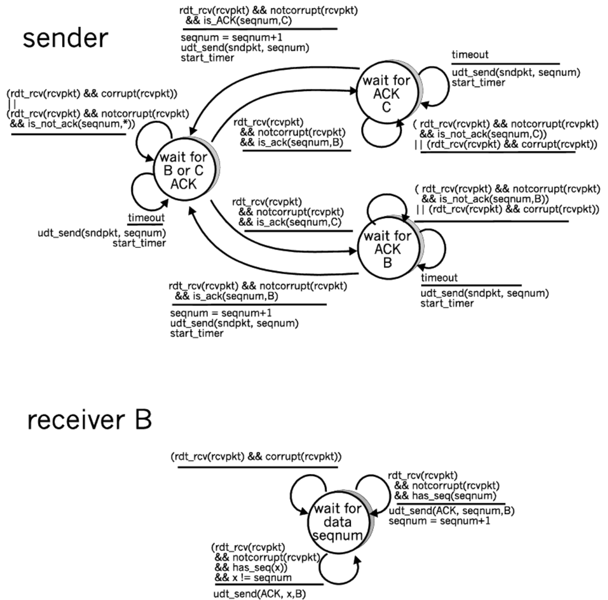
Figure 3. Sender and receiver for Problem 3.19(Problem 19)
