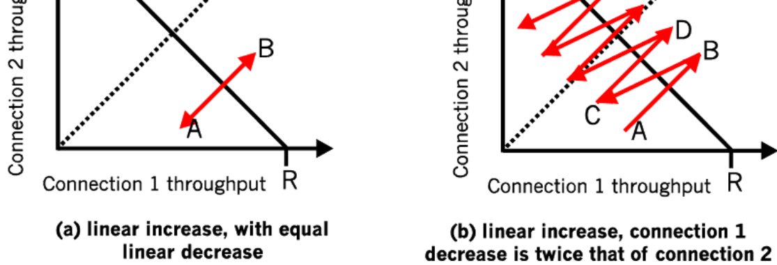
Figure 5: Lack of TCP convergence with linear increase, linear decrease
