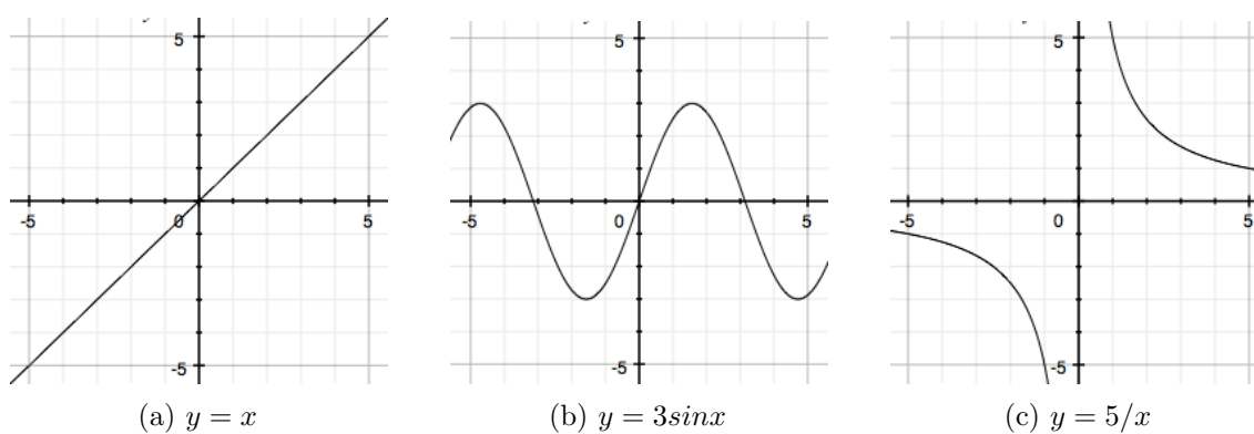
Figure 3.1: Three simple graphs
