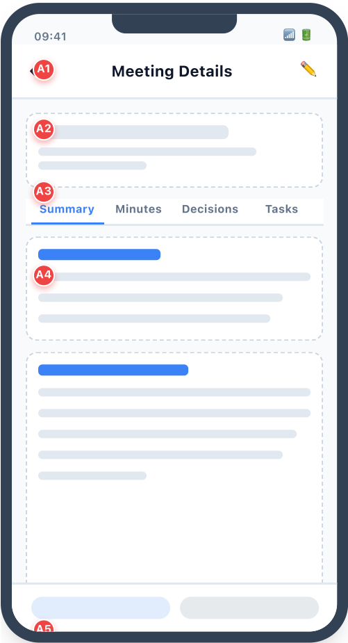
Figure 5.3: Schematic Wireframe and Layout Annotations for the Meeting Details Screen.
