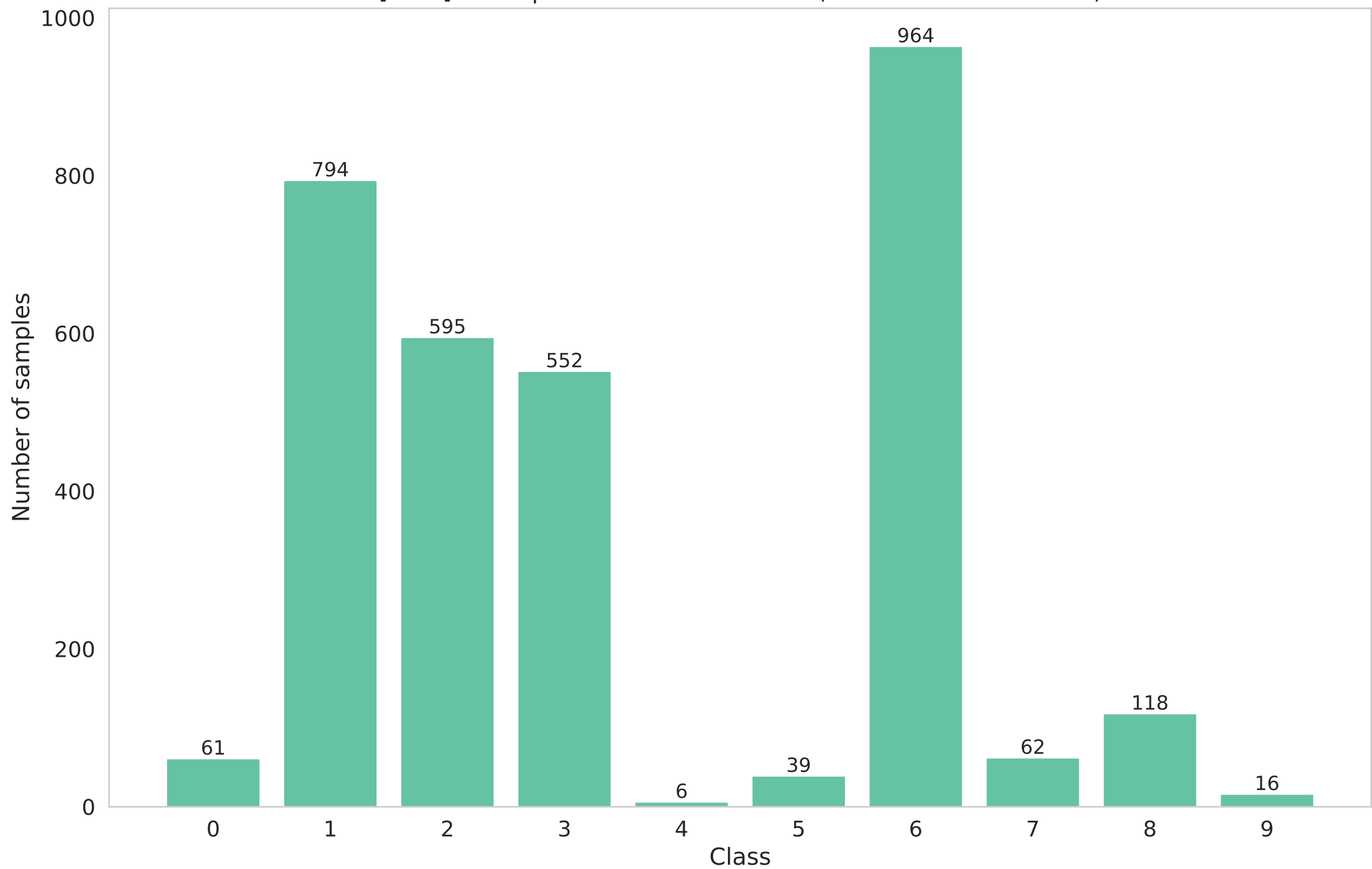
[train] Participant 5 data distribution (Non-IID - dirichlet - 0.5)
