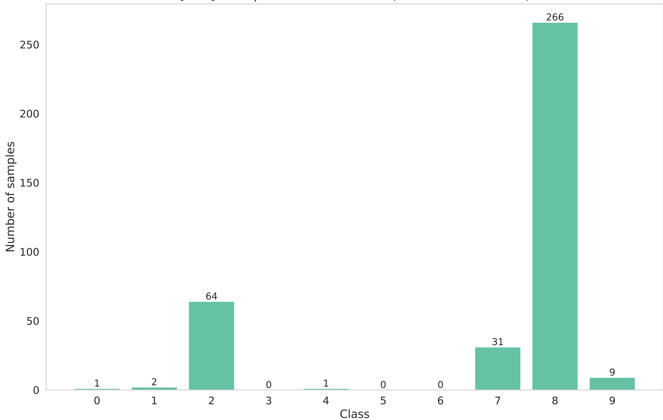
[train] Participant 4 data distribution (Non-IID - dirichlet - 0.1)
