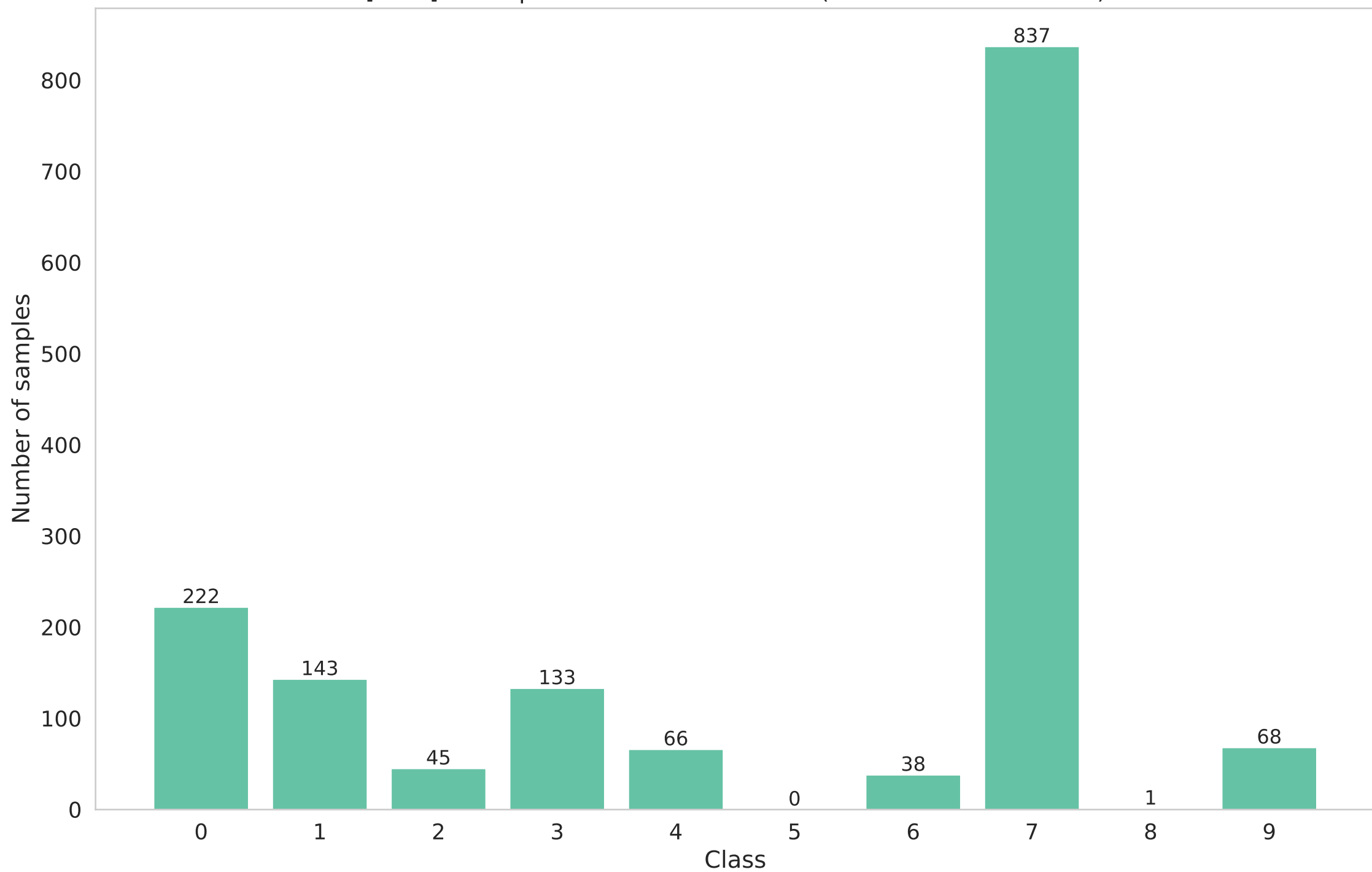
[train] Participant 12 data distribution (Non-IID - dirichlet - 0.3)
