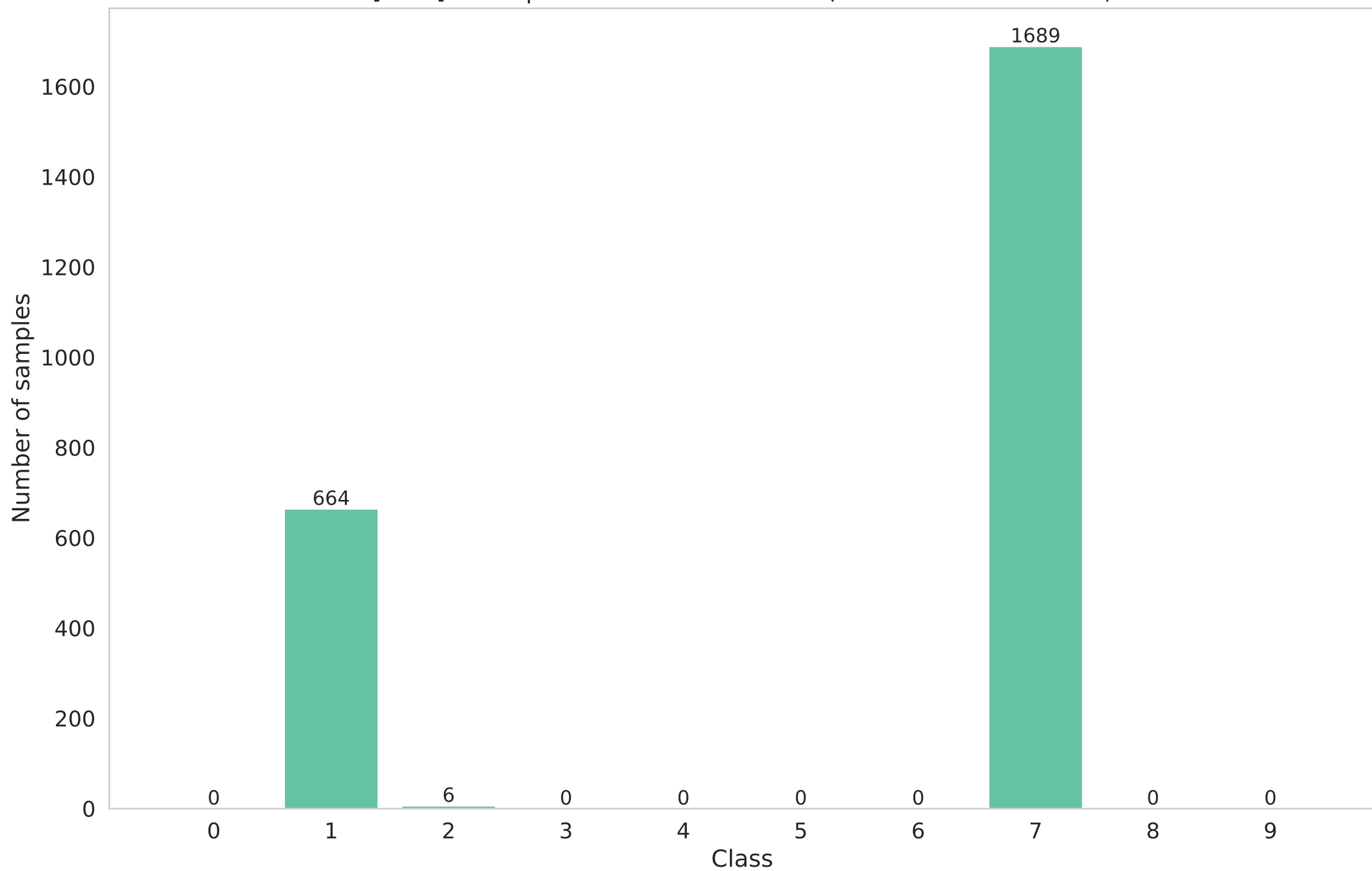
[train] Participant 14 data distribution (Non-IID - dirichlet - 0.1)
