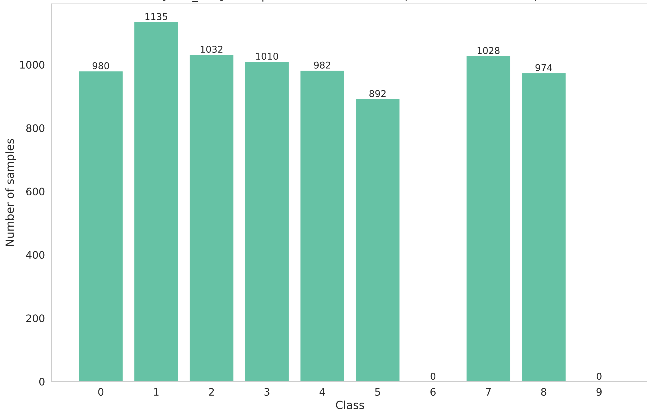
[local_test] Participant 10 data distribution (Non-IID - dirichlet - 0.1)
