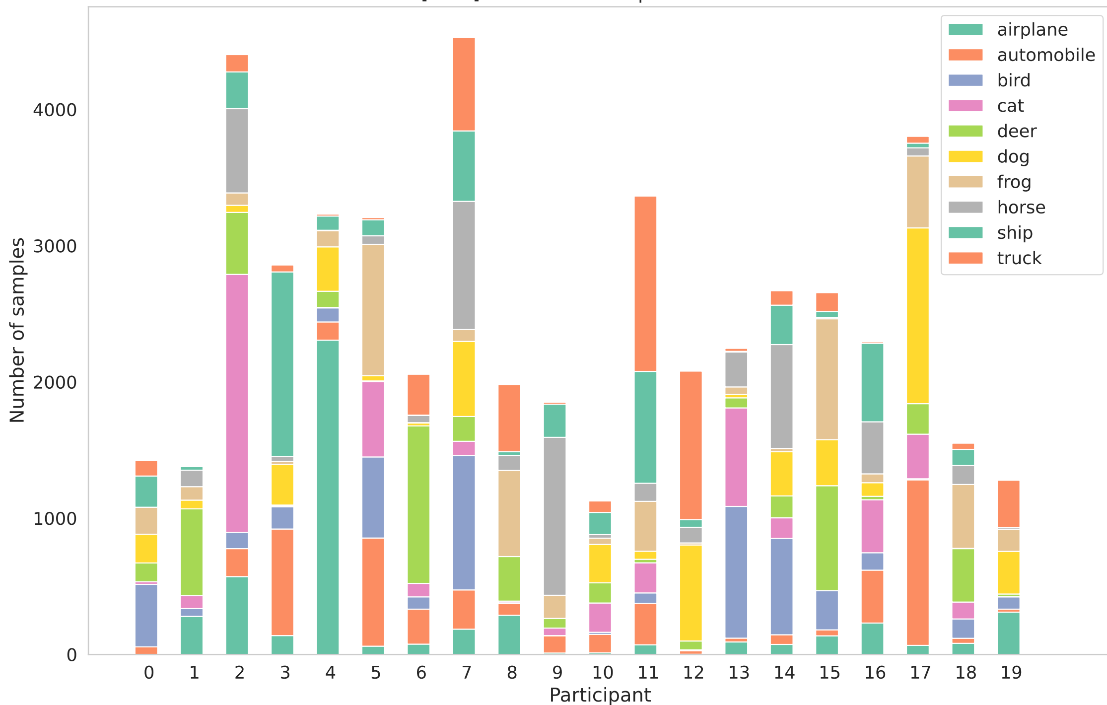
[train] Distribution of splitted datasets
