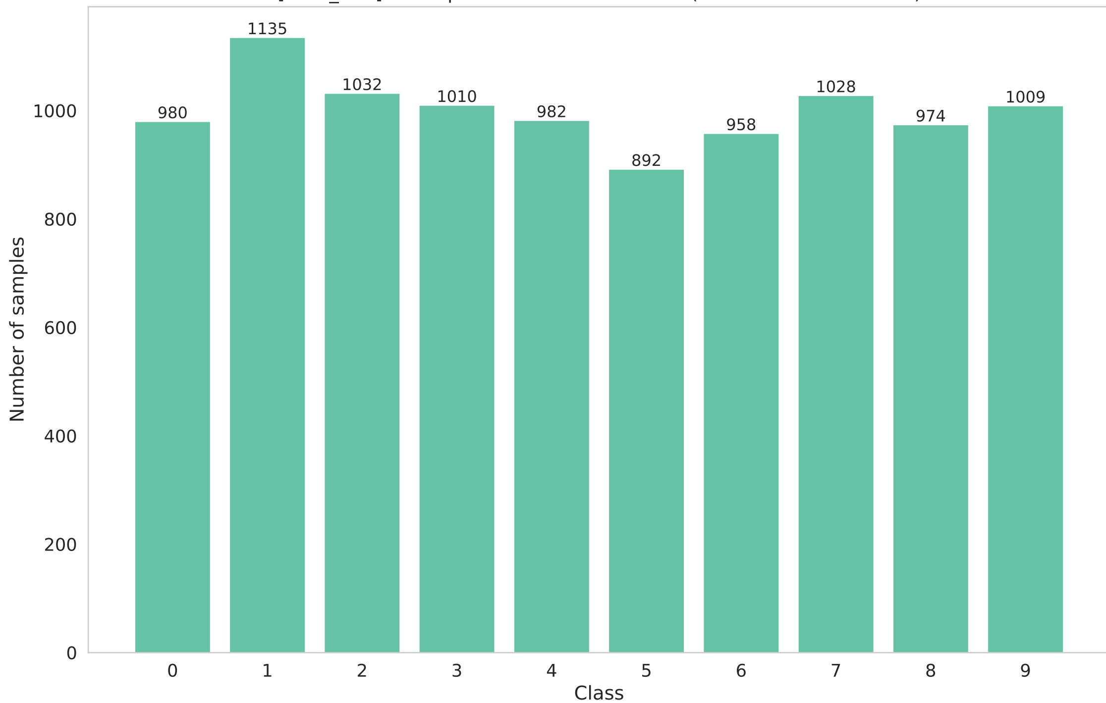
[local_test] Participant 19 data distribution (Non-IID - dirichlet - 0.1)
