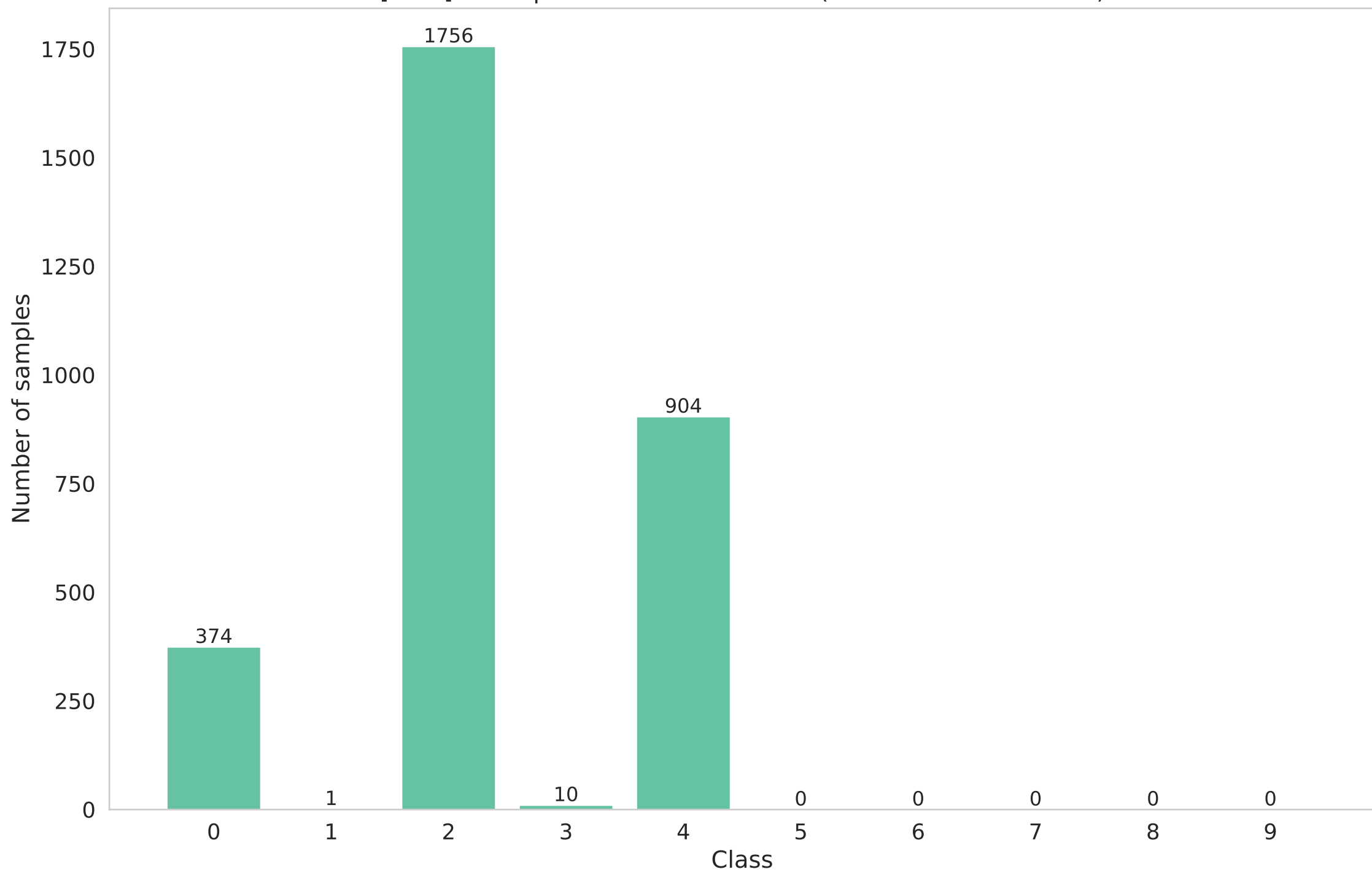
[train] Participant 3 data distribution (Non-IID - dirichlet - 0.1)
