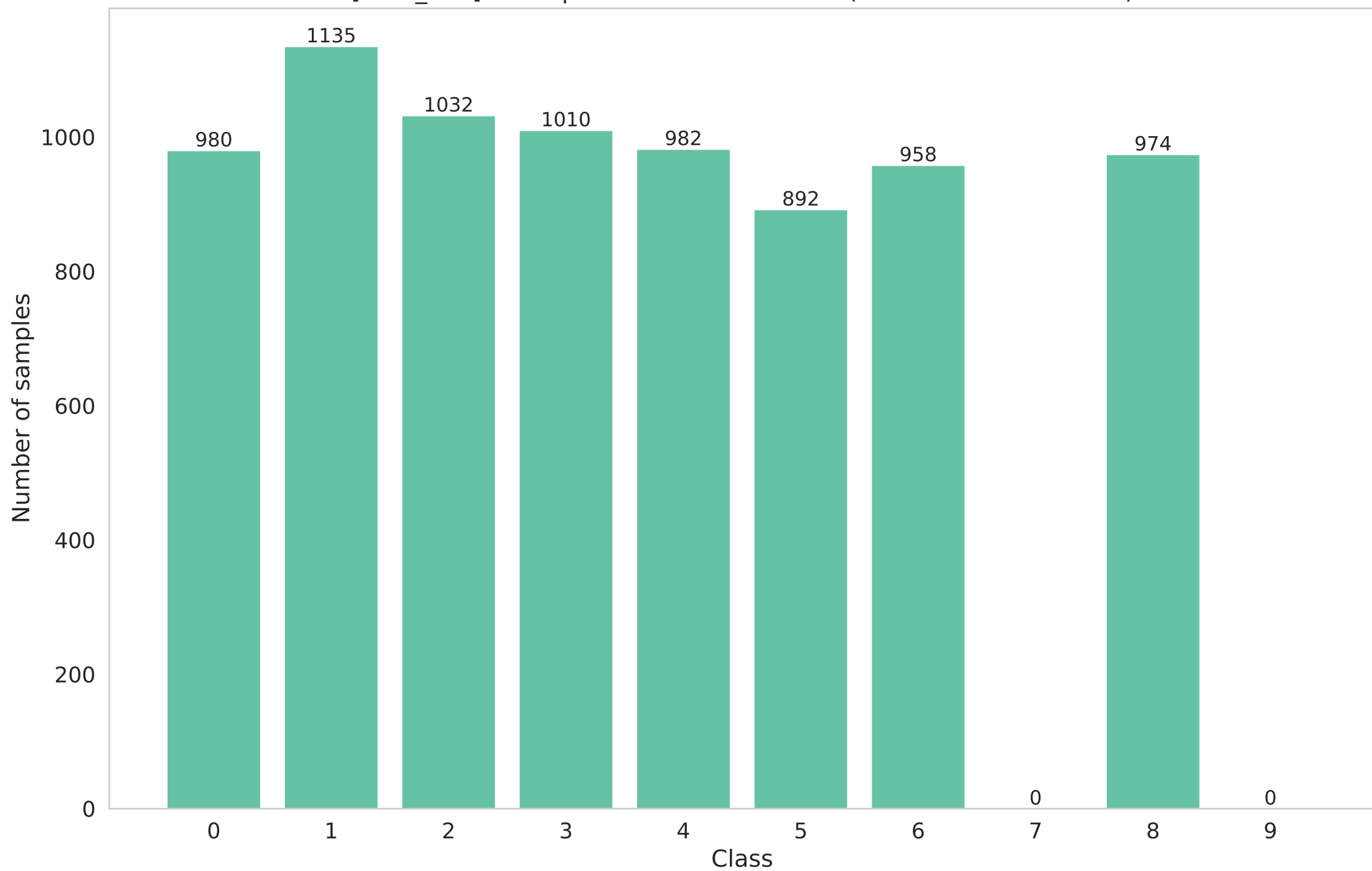
[local_test] Participant 9 data distribution (Non-IID - dirichlet - 0.1)
