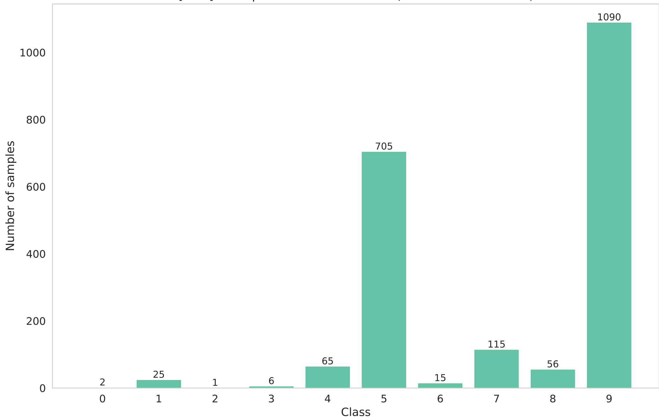
[train] Participant 12 data distribution (Non-IID - dirichlet - 0.5)
