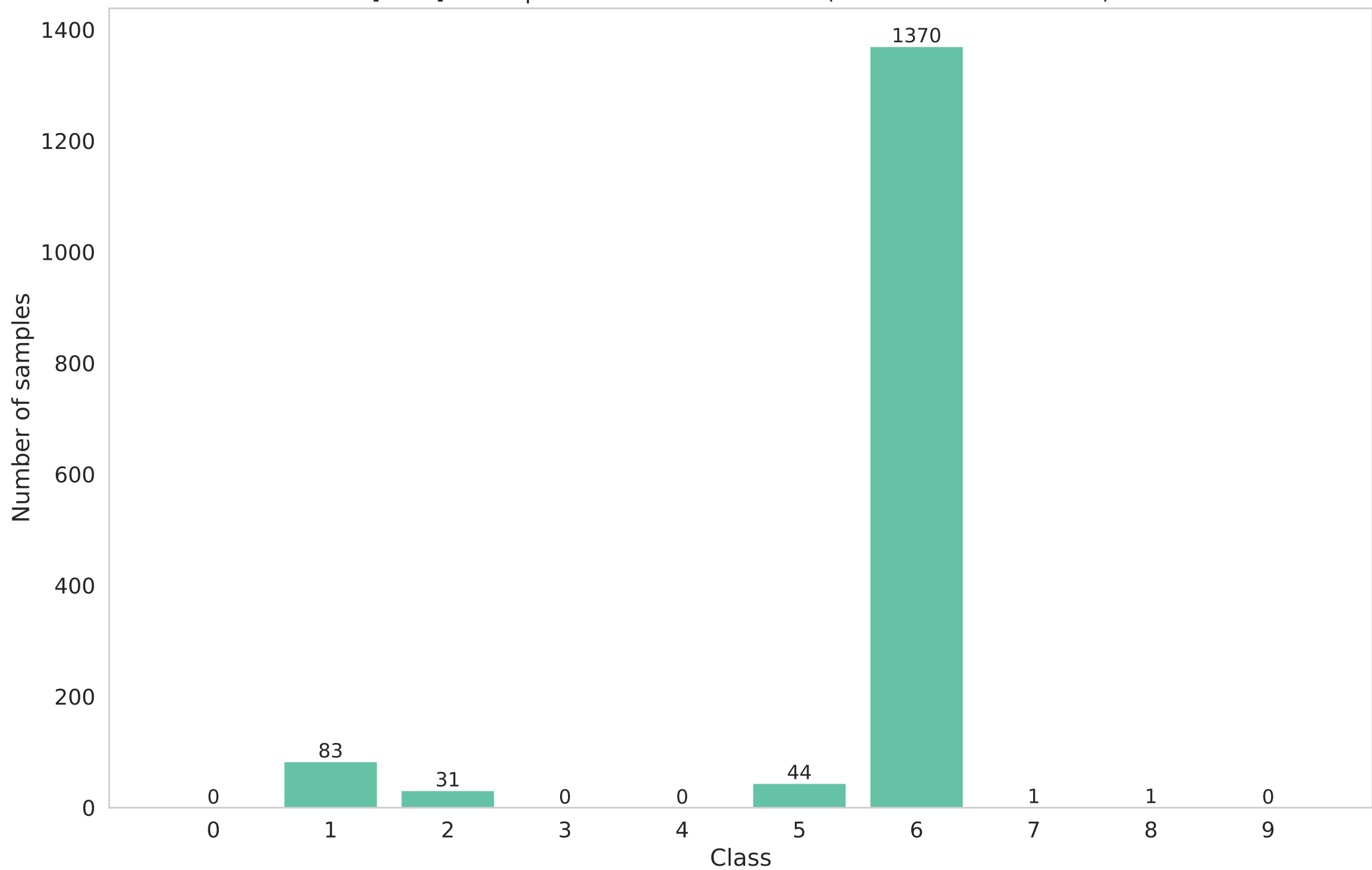
[train] Participant 13 data distribution (Non-IID - dirichlet - 0.1)
