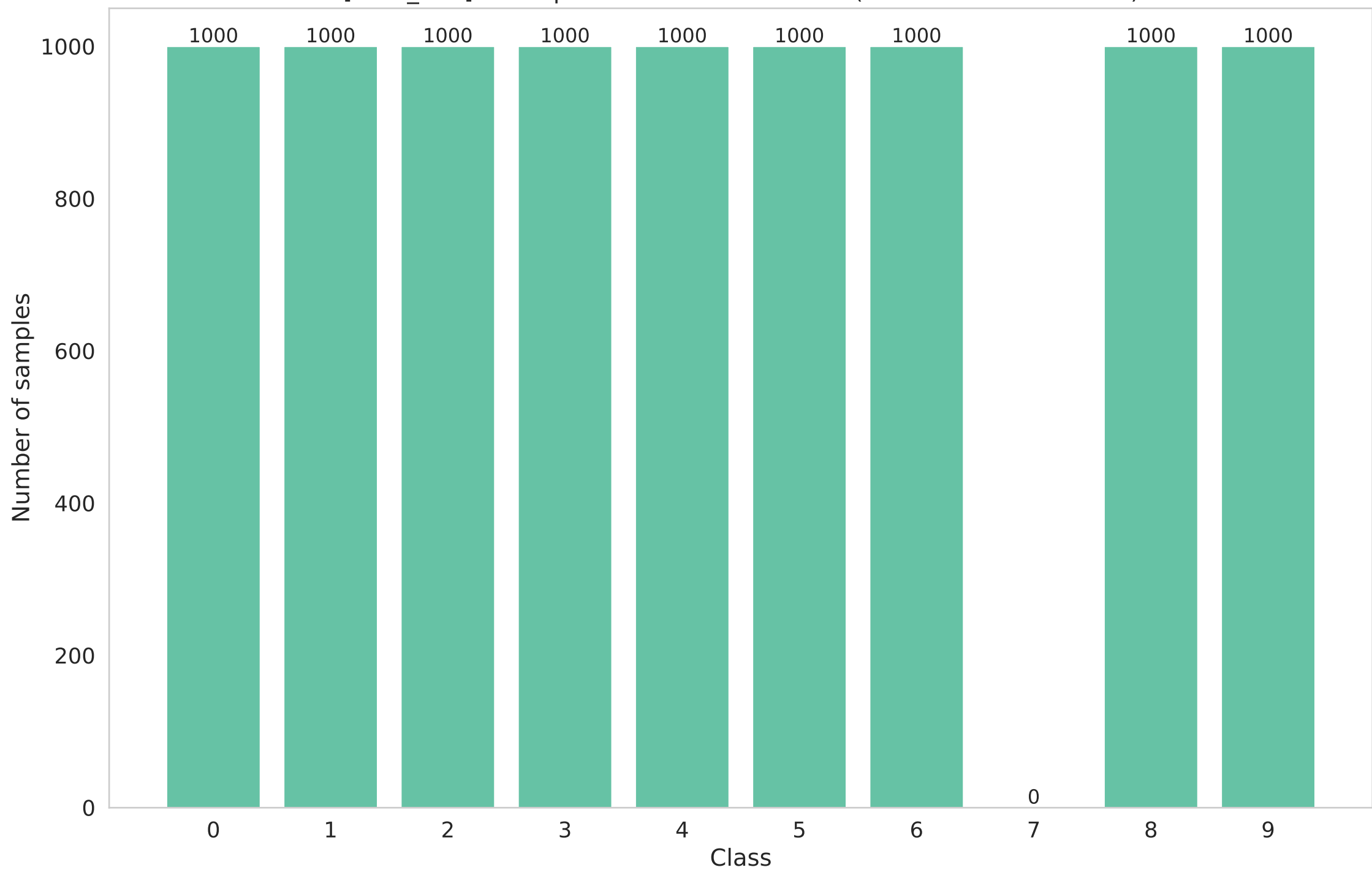
[local_test] Participant 10 data distribution (Non-IID - dirichlet - 0.3)
