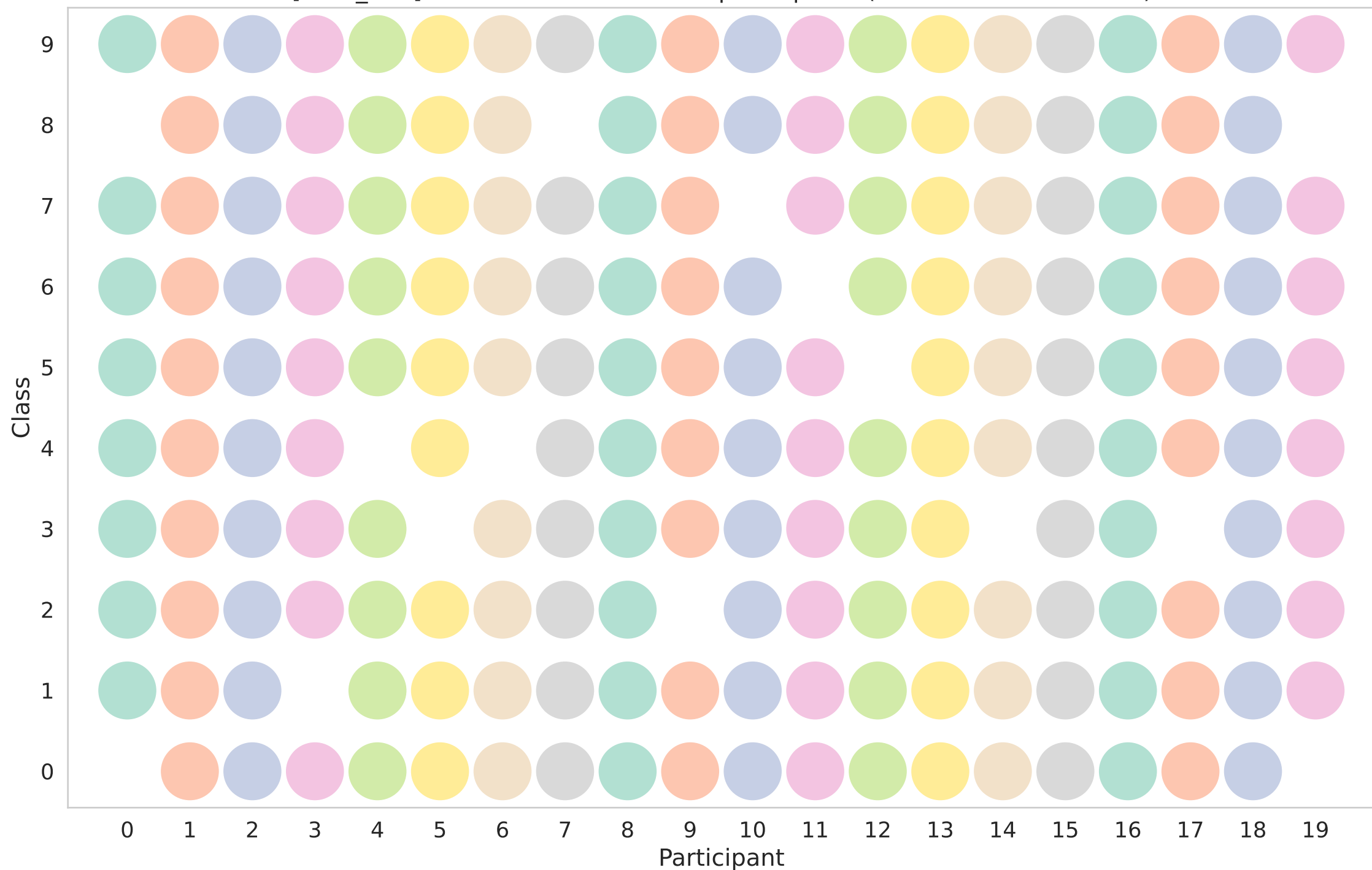
[local test] Data distribution across participants (Non-IID - dirichlet - 0.3)
