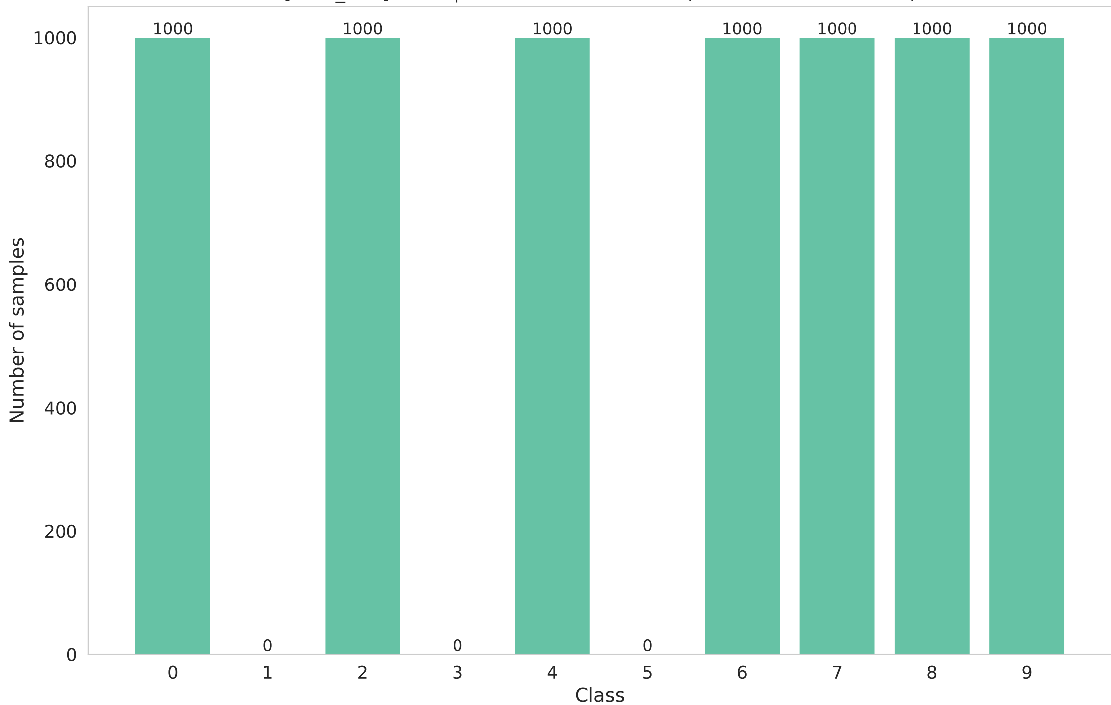
[local_test] Participant 1 data distribution (Non-IID - dirichlet - 0.1)
