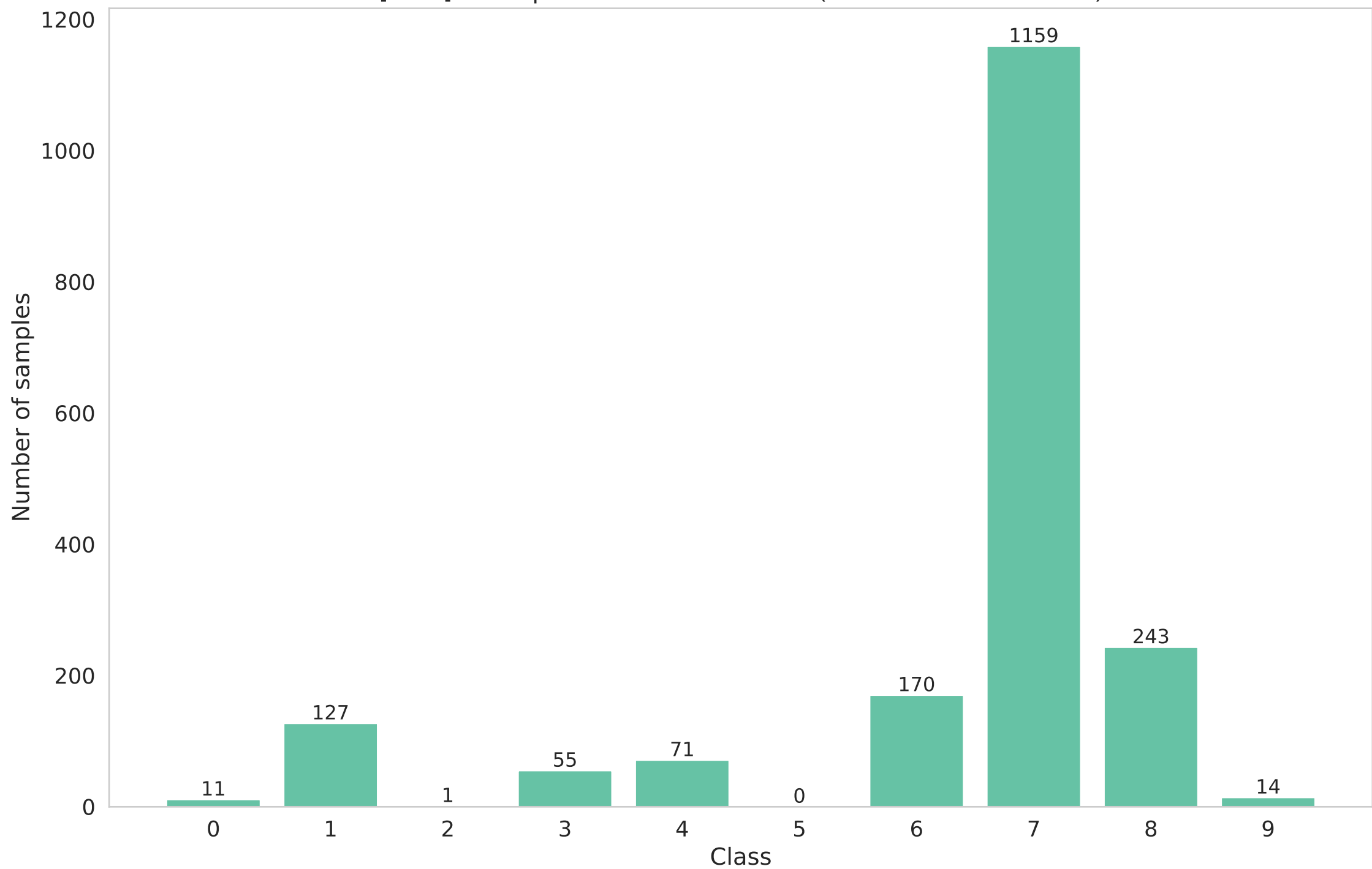
[train] Participant 9 data distribution (Non-IID - dirichlet - 0.5)
