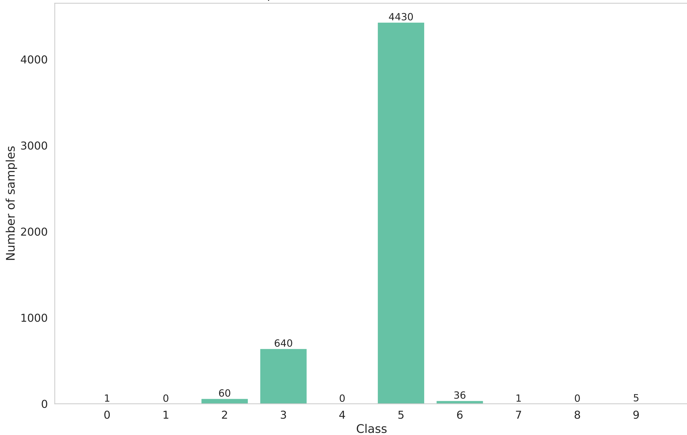
[train] Participant 1 data distribution (Non-IID - dirichlet - 0.1)
