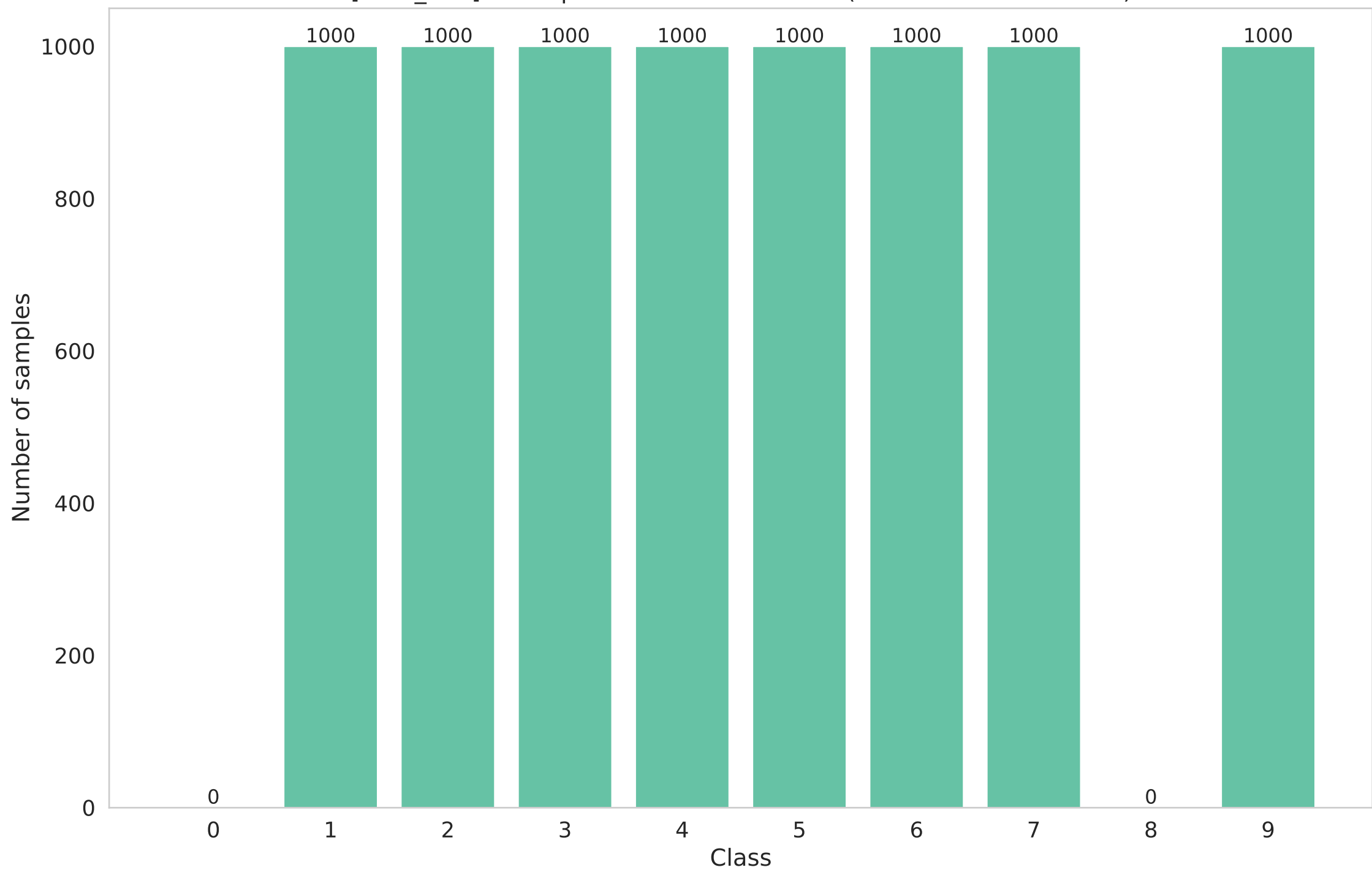
[local_test] Participant 0 data distribution (Non-IID - dirichlet - 0.3)
