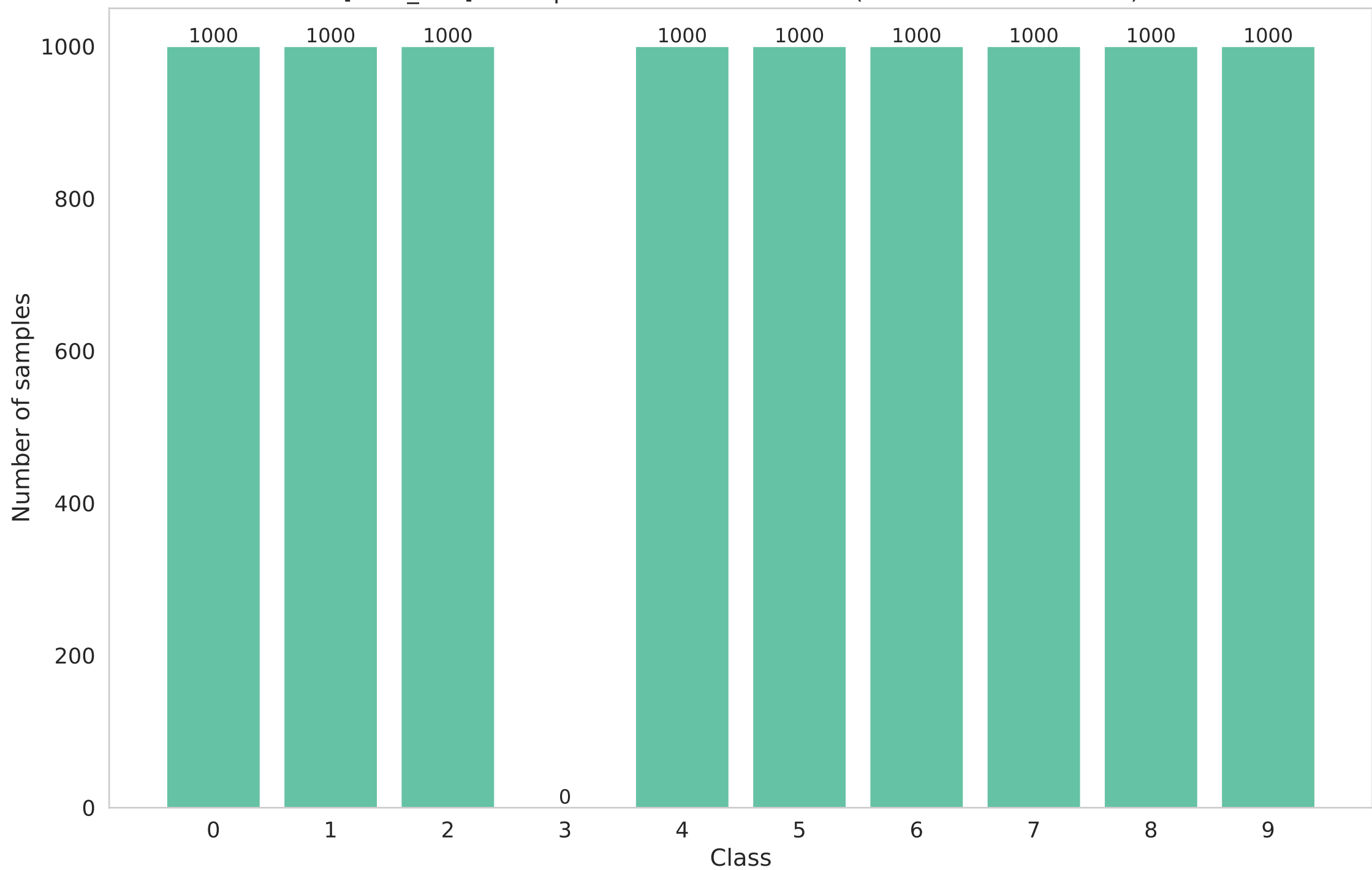
[local_test] Participant 14 data distribution (Non-IID - dirichlet - 0.3)
