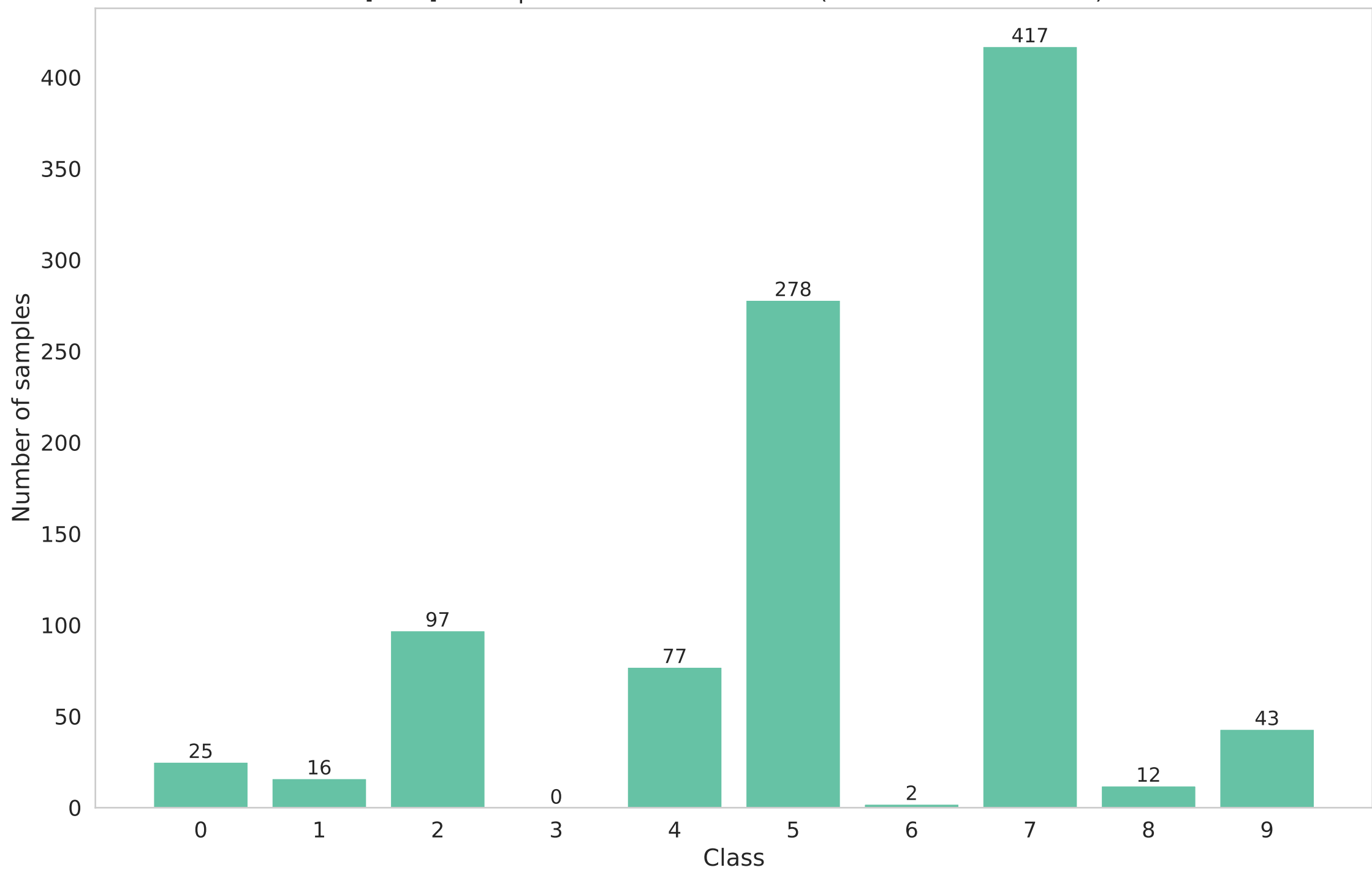
[train] Participant 17 data distribution (Non-IID - dirichlet - 0.3)
