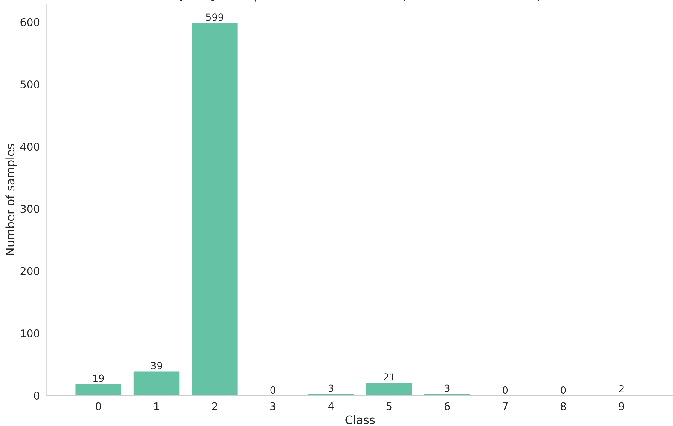
[train] Participant 15 data distribution (Non-IID - dirichlet - 0.1)
