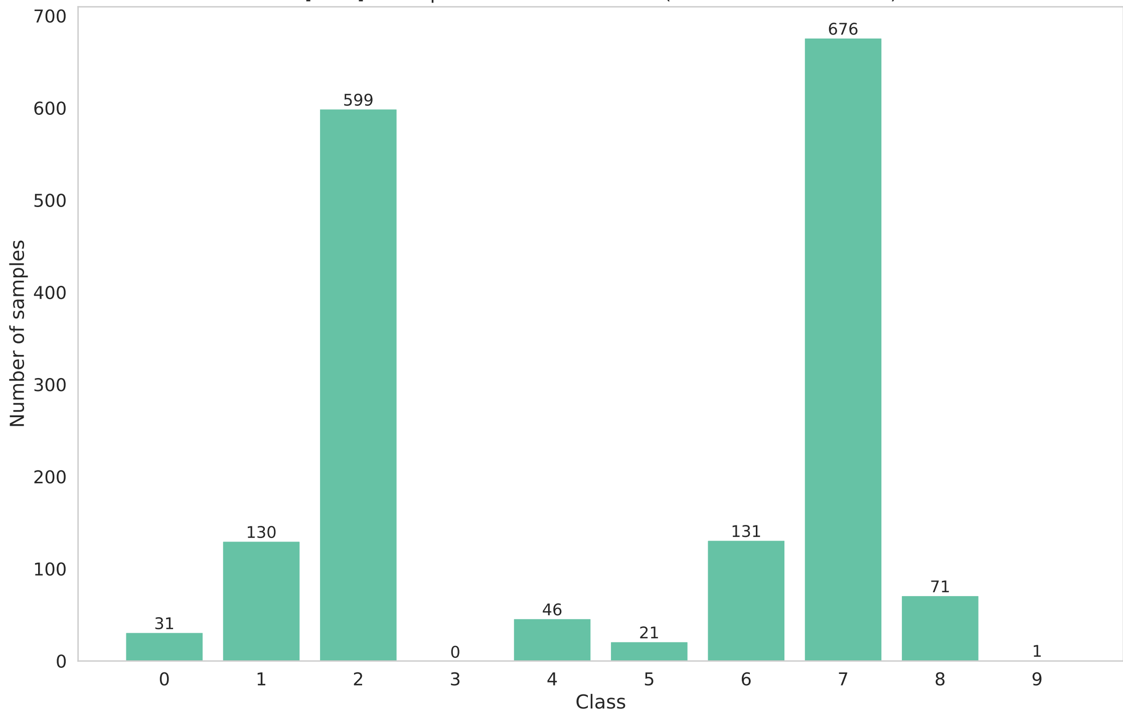
[train] Participant 5 data distribution (Non-IID - dirichlet - 0.3)
