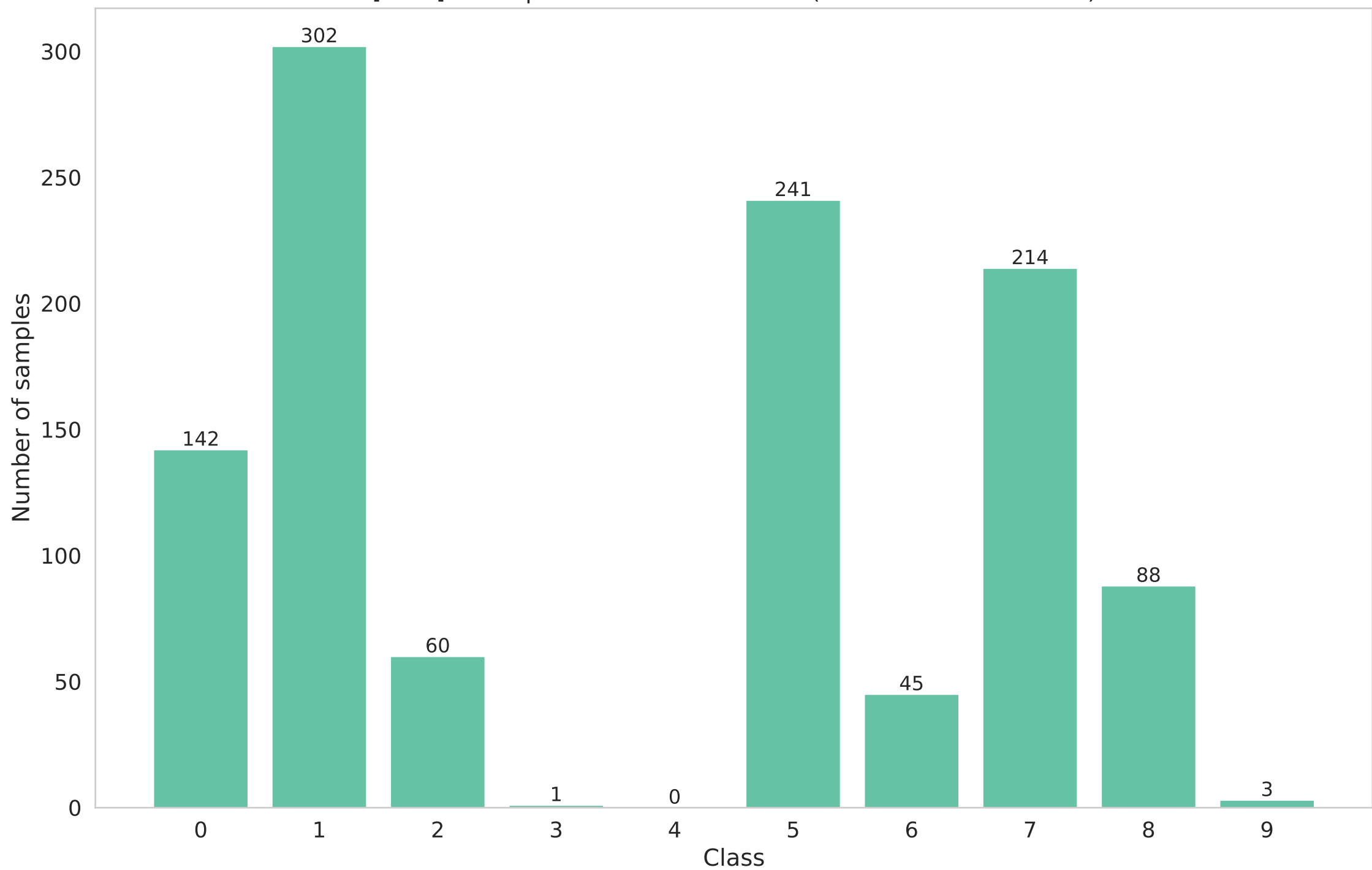
[train] Participant 6 data distribution (Non-IID - dirichlet - 0.3)
