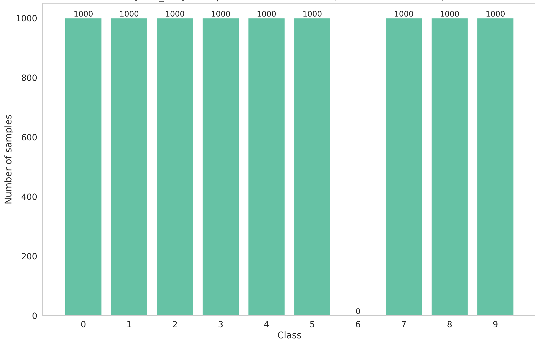
[local_test] Participant 11 data distribution (Non-IID - dirichlet - 0.3)
