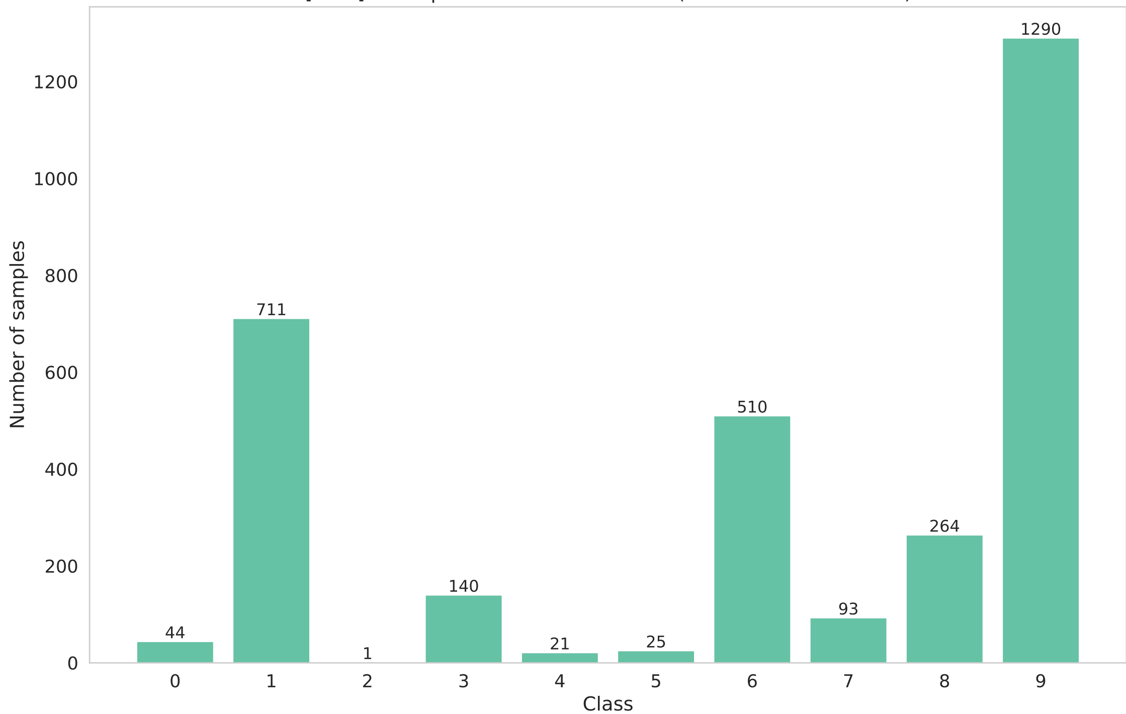
[train] Participant 13 data distribution (Non-IID - dirichlet - 0.3)
