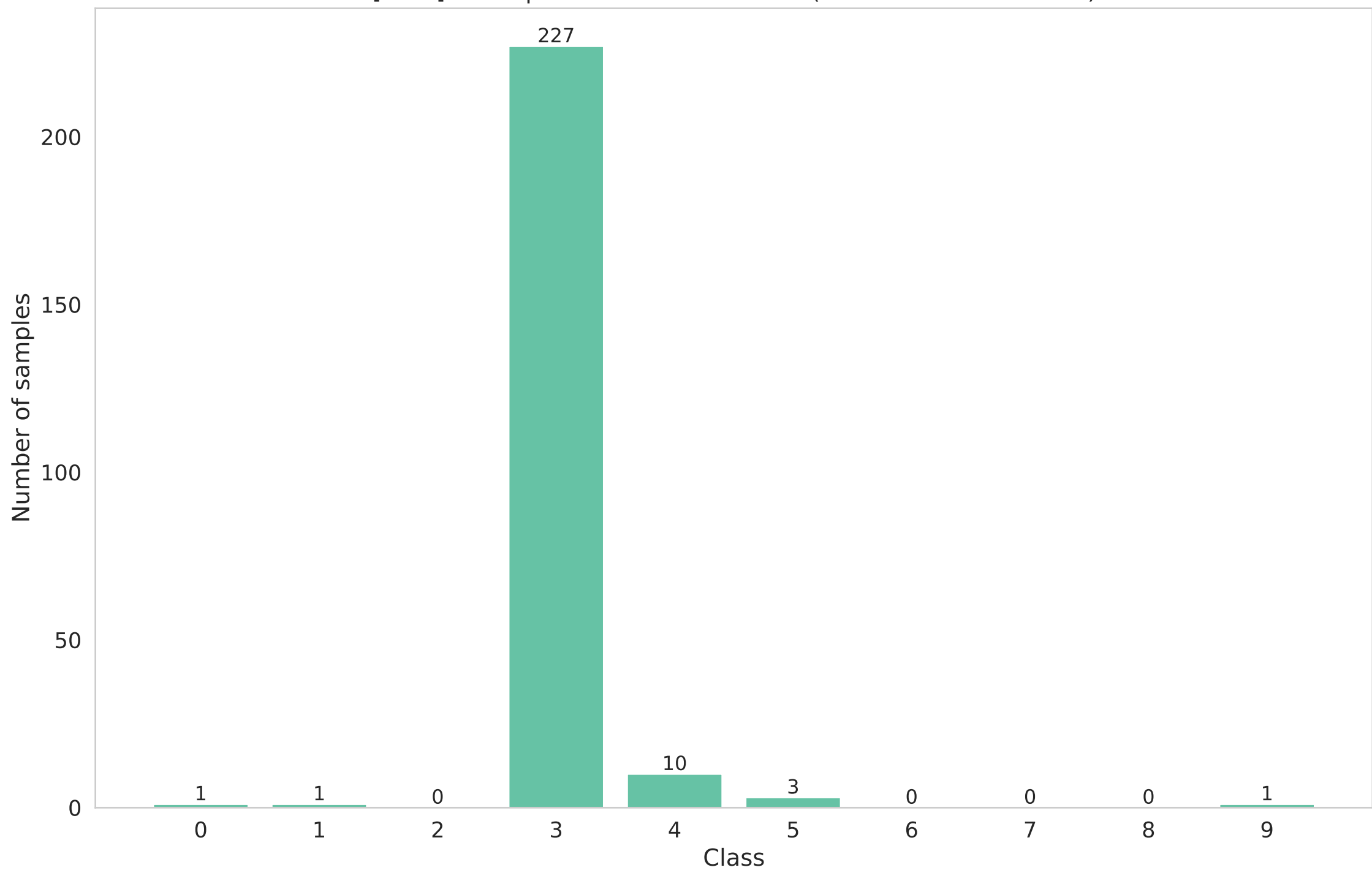
[train] Participant 7 data distribution (Non-IID - dirichlet - 0.1)
