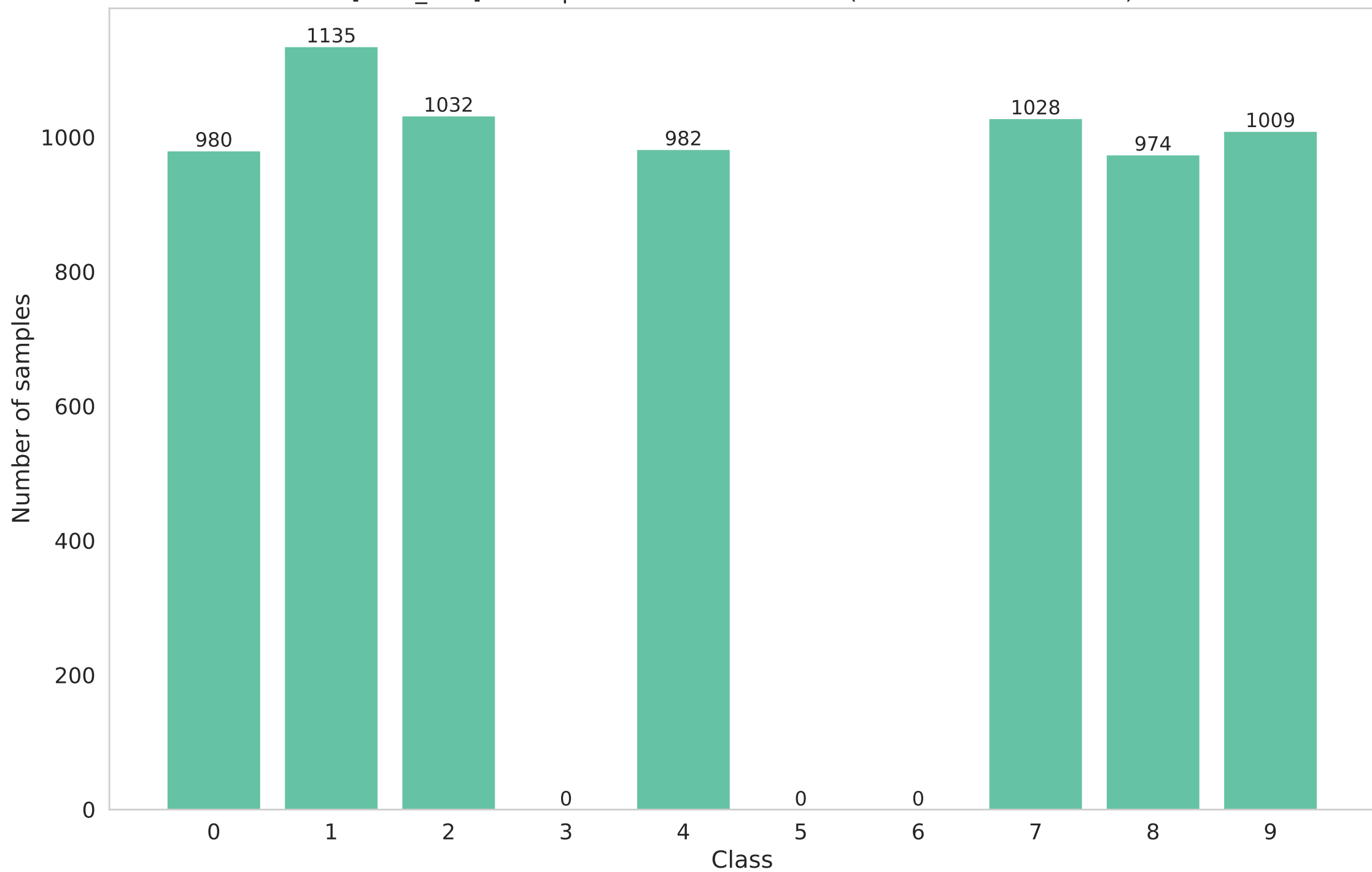
[local_test] Participant 4 data distribution (Non-IID - dirichlet - 0.1)
