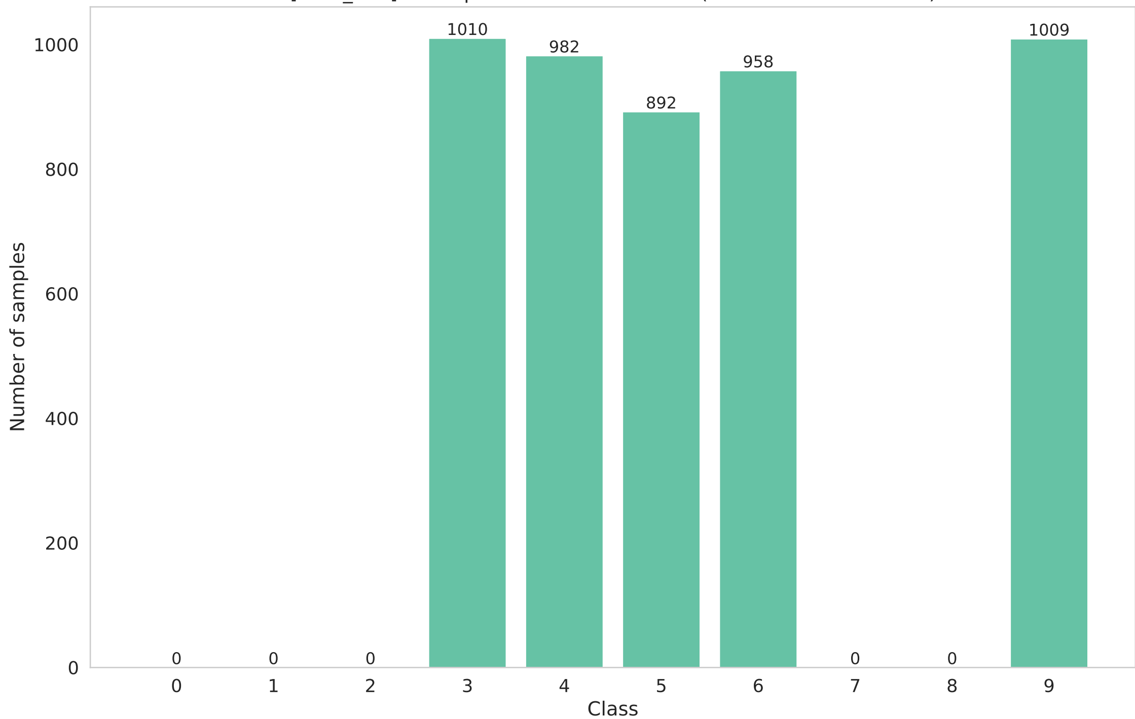
[local_test] Participant 8 data distribution (Non-IID - dirichlet - 0.1)
