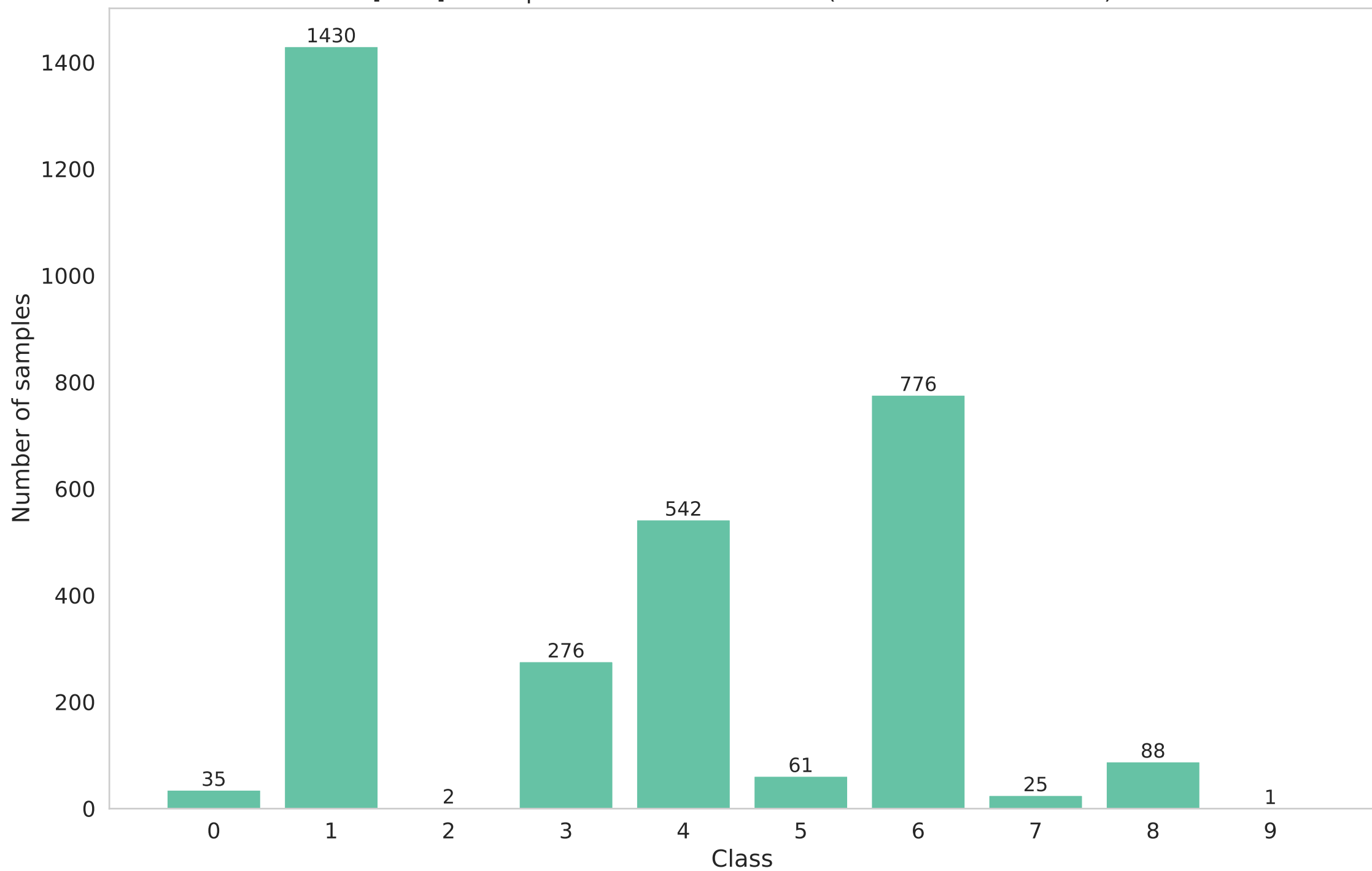
[train] Participant 18 data distribution (Non-IID - dirichlet - 0.3)
