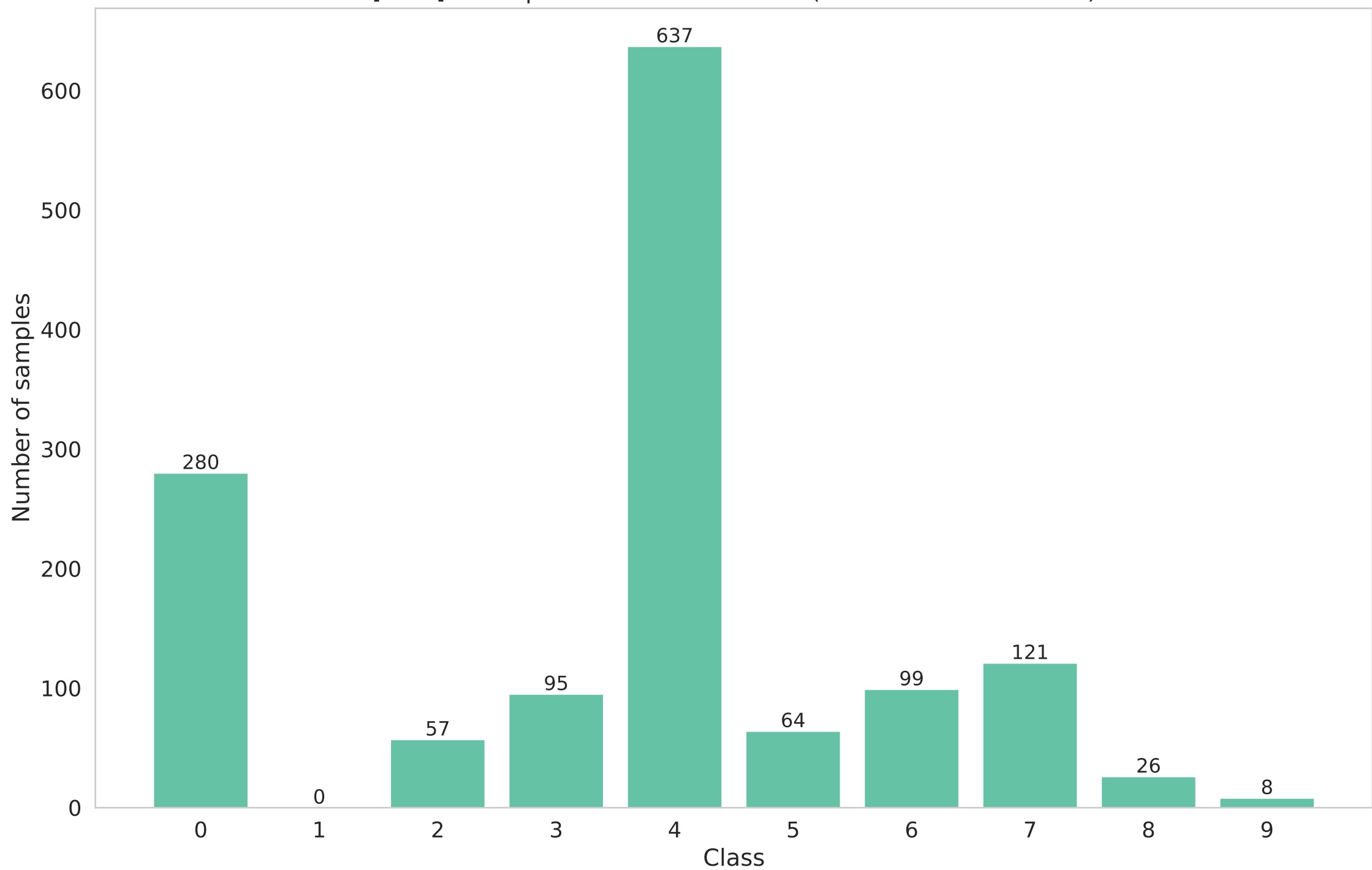
[train] Participant 1 data distribution (Non-IID - dirichlet - 0.5)
