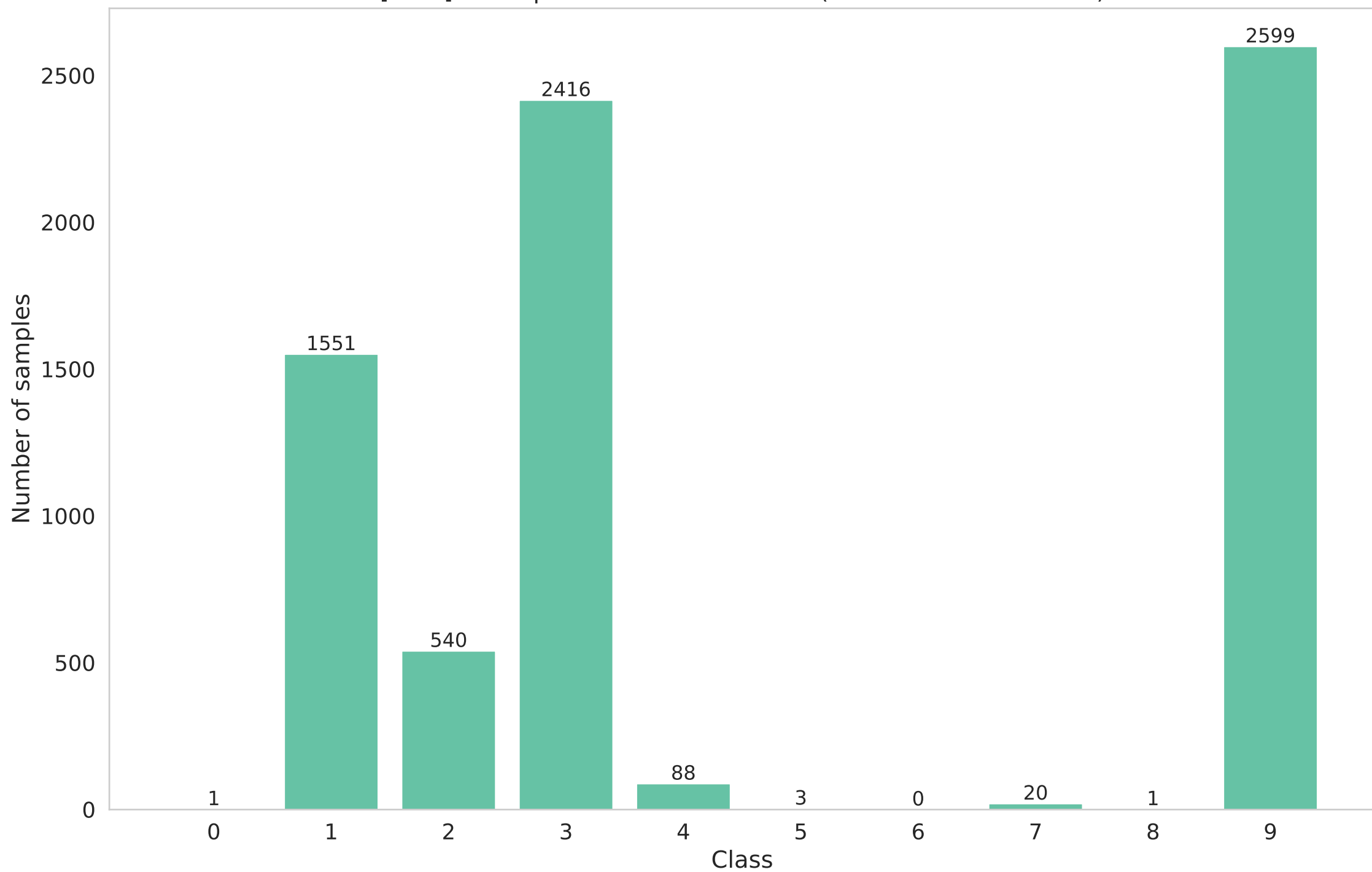
[train] Participant 8 data distribution (Non-IID - dirichlet - 0.1)
