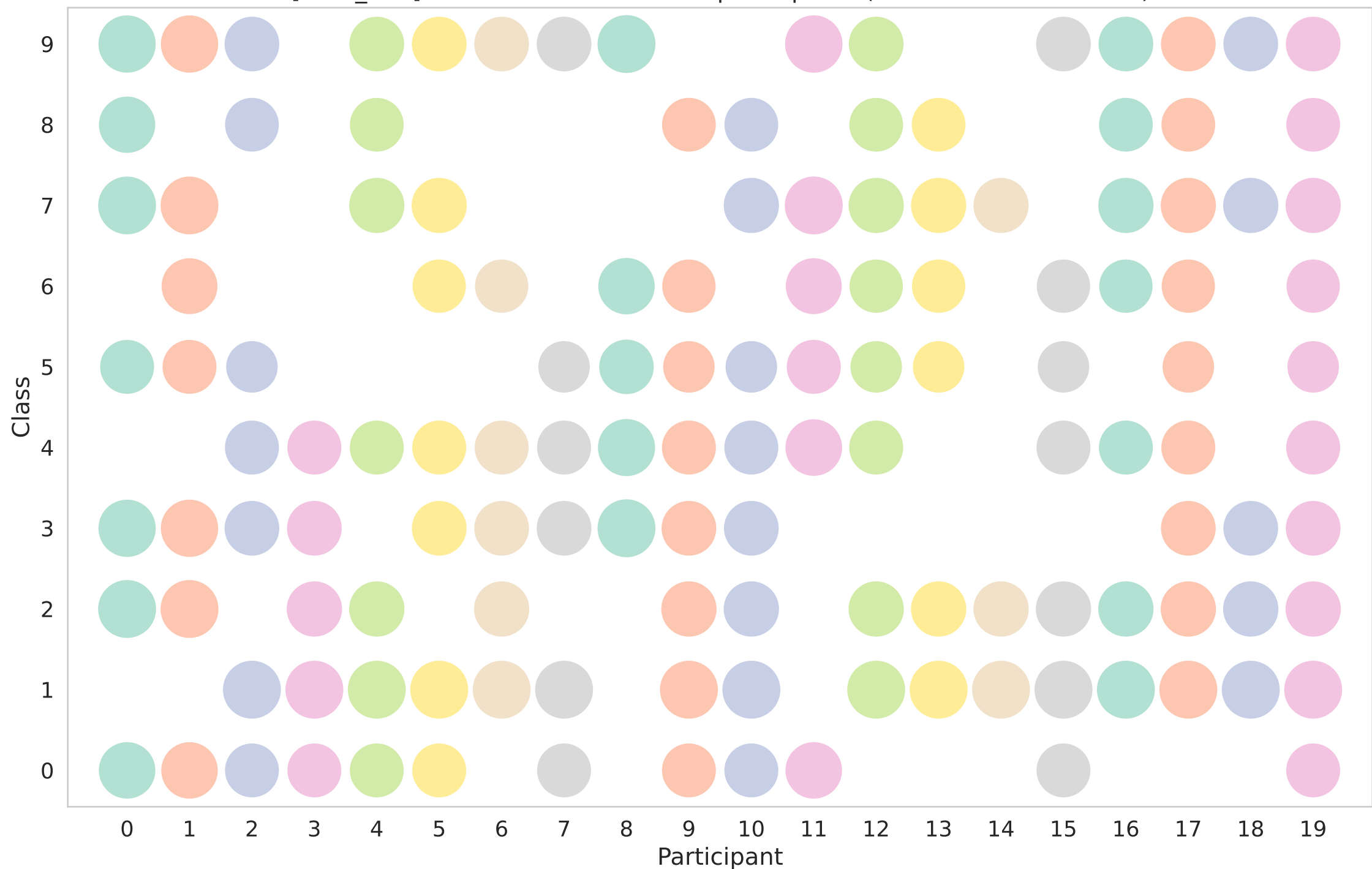
[local test] Data distribution across participants (Non-IID - dirichlet - 0.1)
