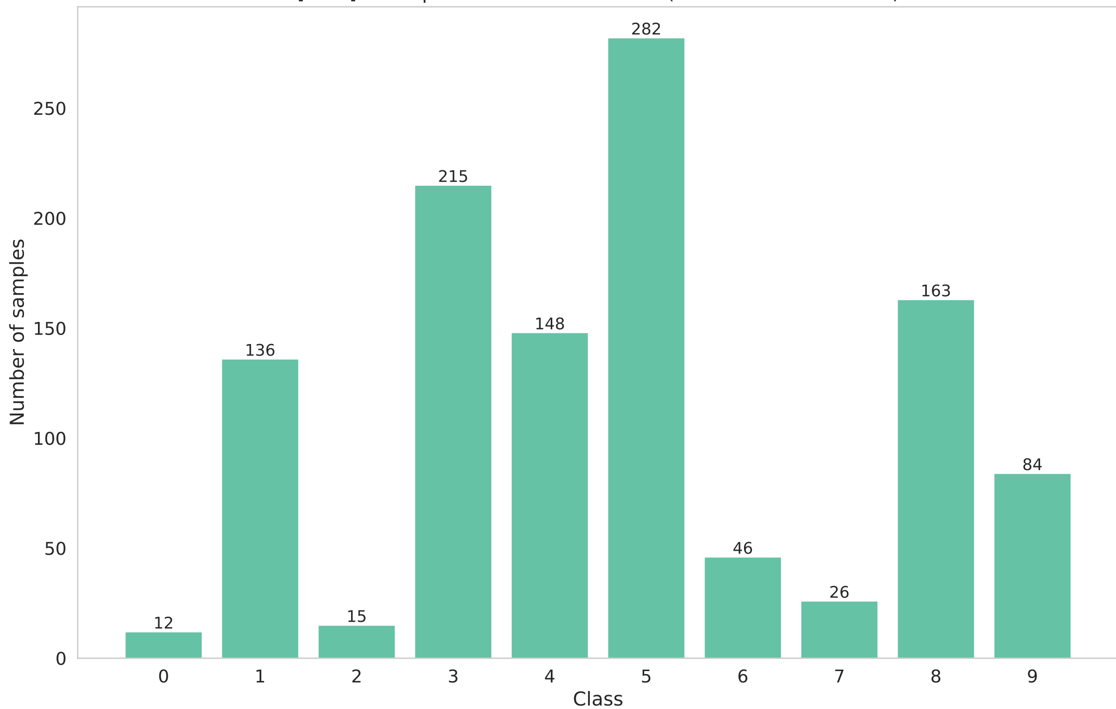
[train] Participant 10 data distribution (Non-IID - dirichlet - 0.5)
