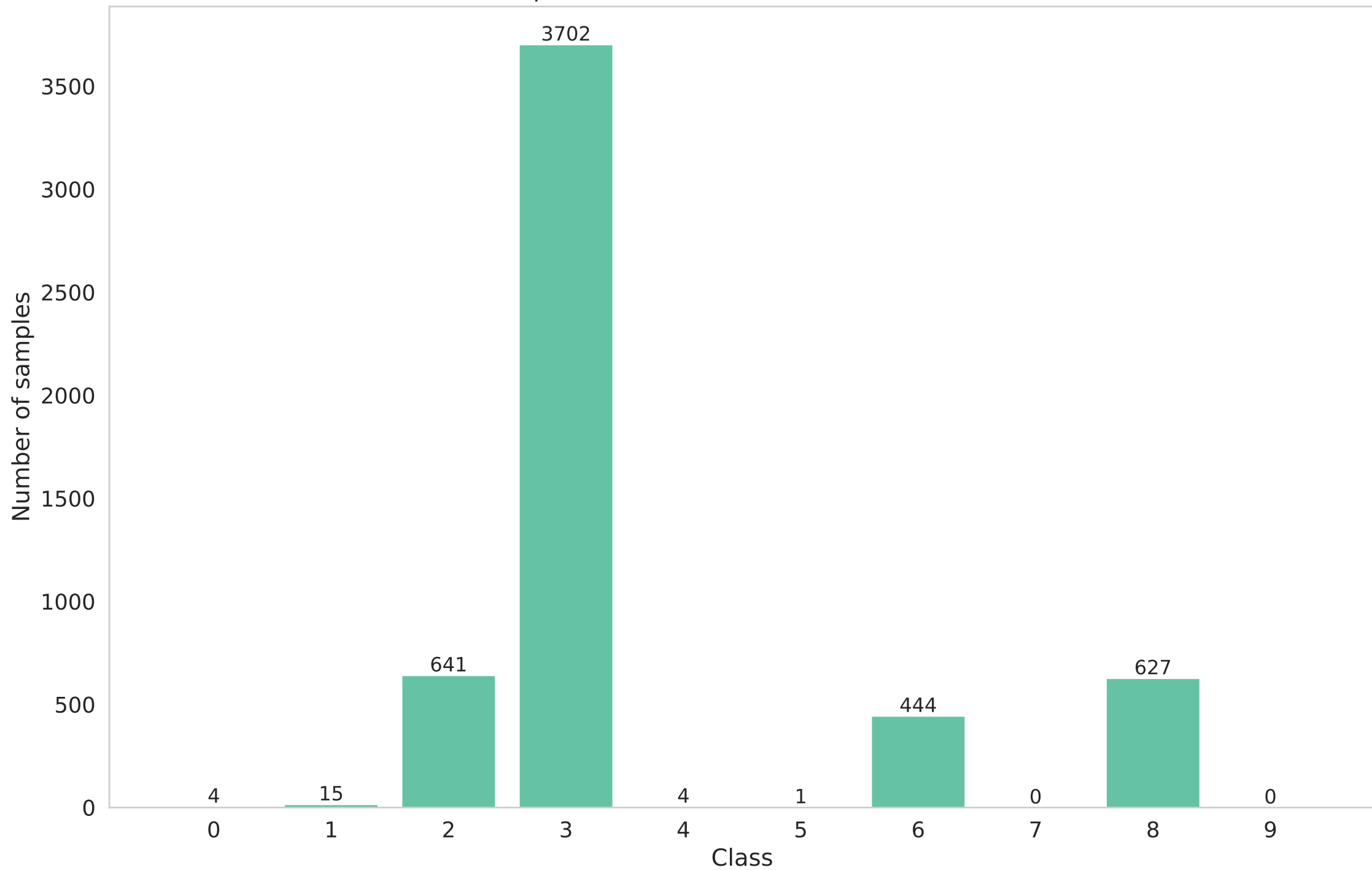
[train] Participant 9 data distribution (Non-IID - dirichlet - 0.1)
