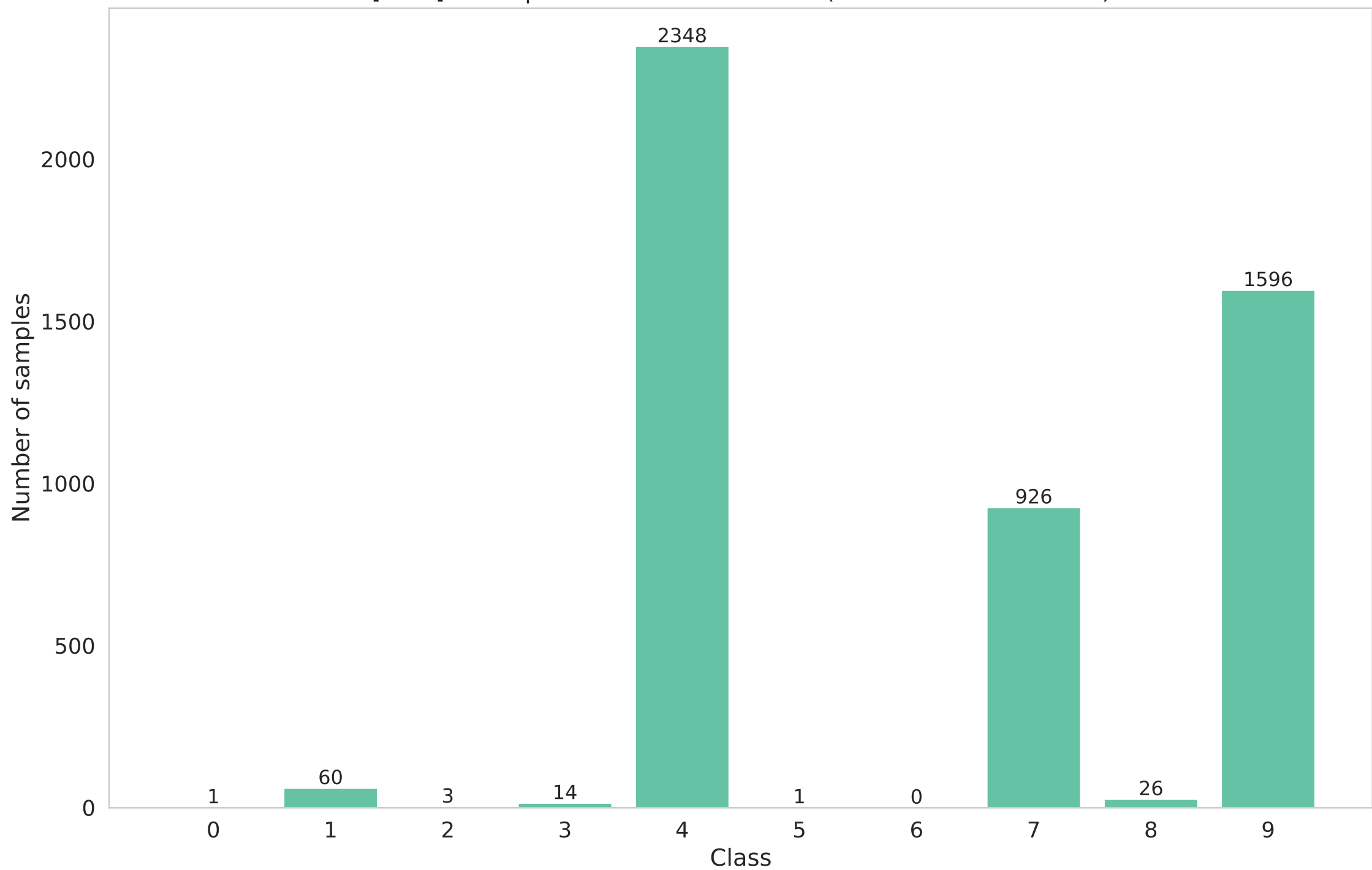
[train] Participant 11 data distribution (Non-IID - dirichlet - 0.3)
