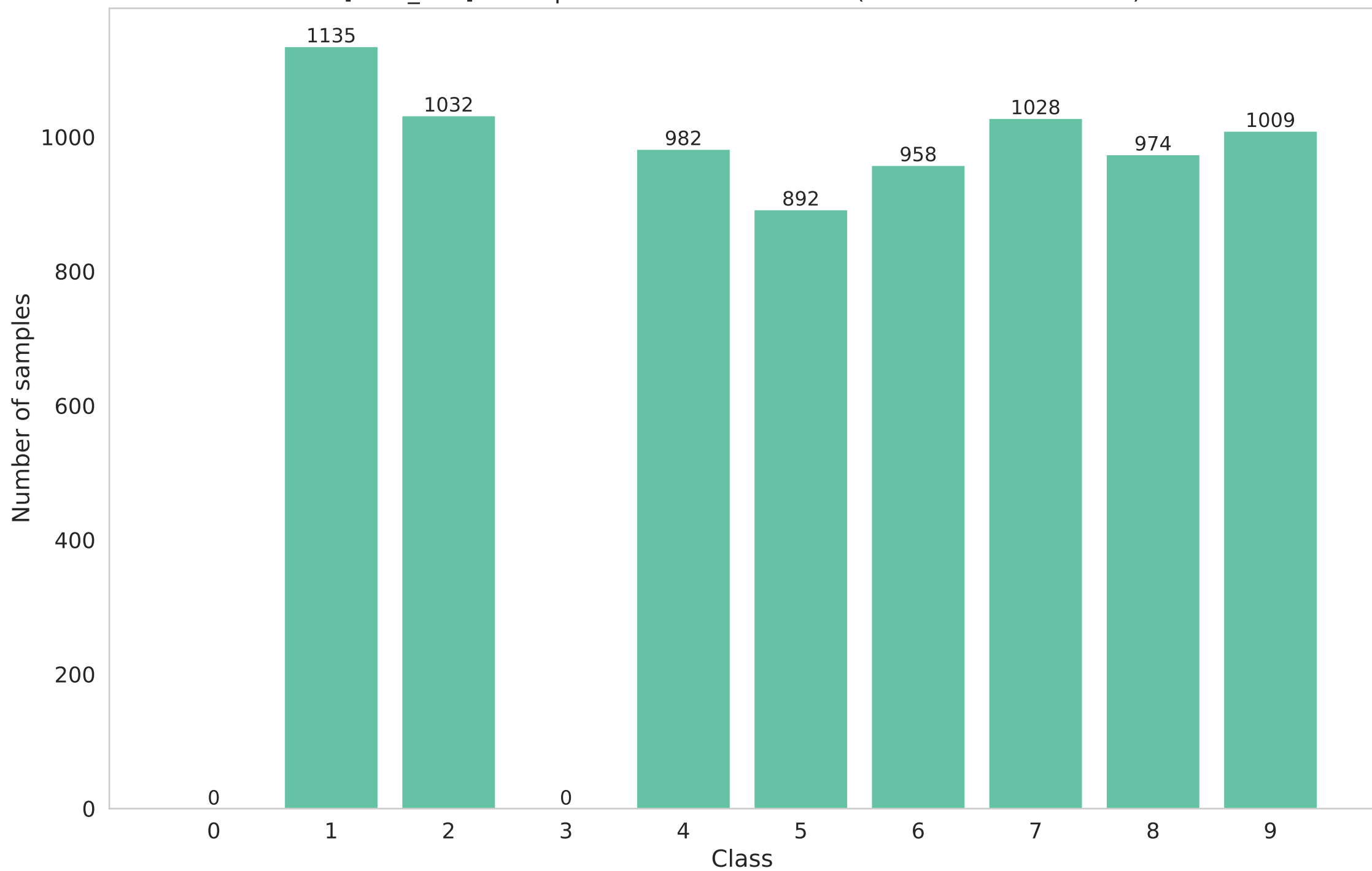
[local_test] Participant 12 data distribution (Non-IID - dirichlet - 0.1)
