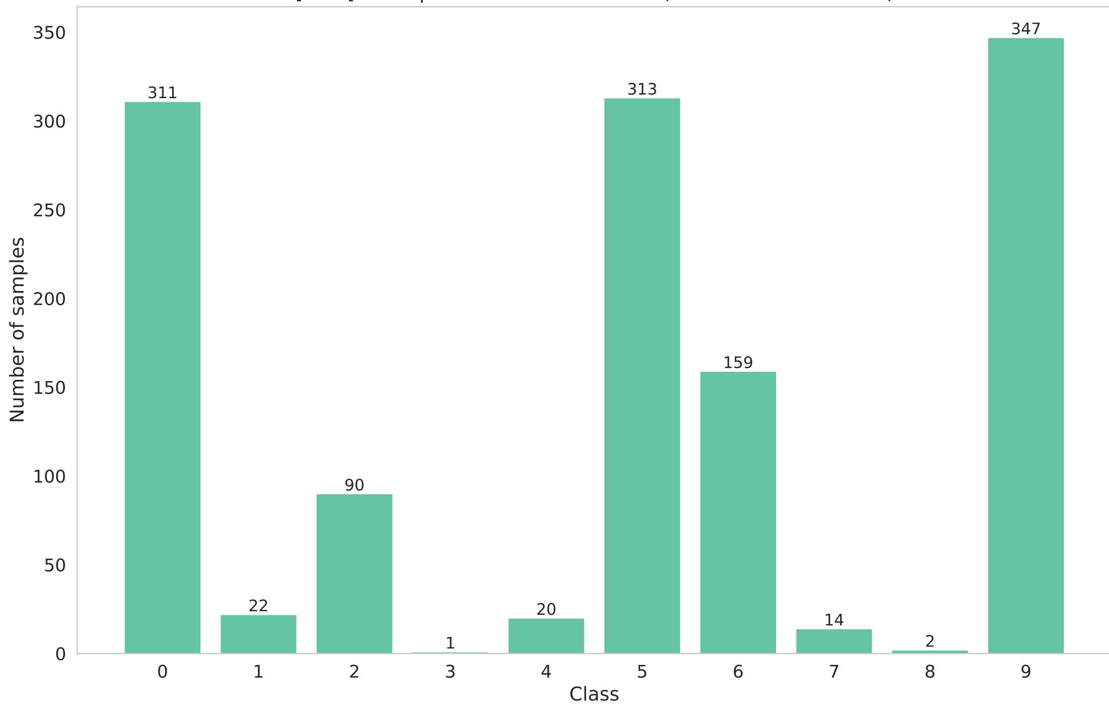
[train] Participant 19 data distribution (Non-IID - dirichlet - 0.5)
