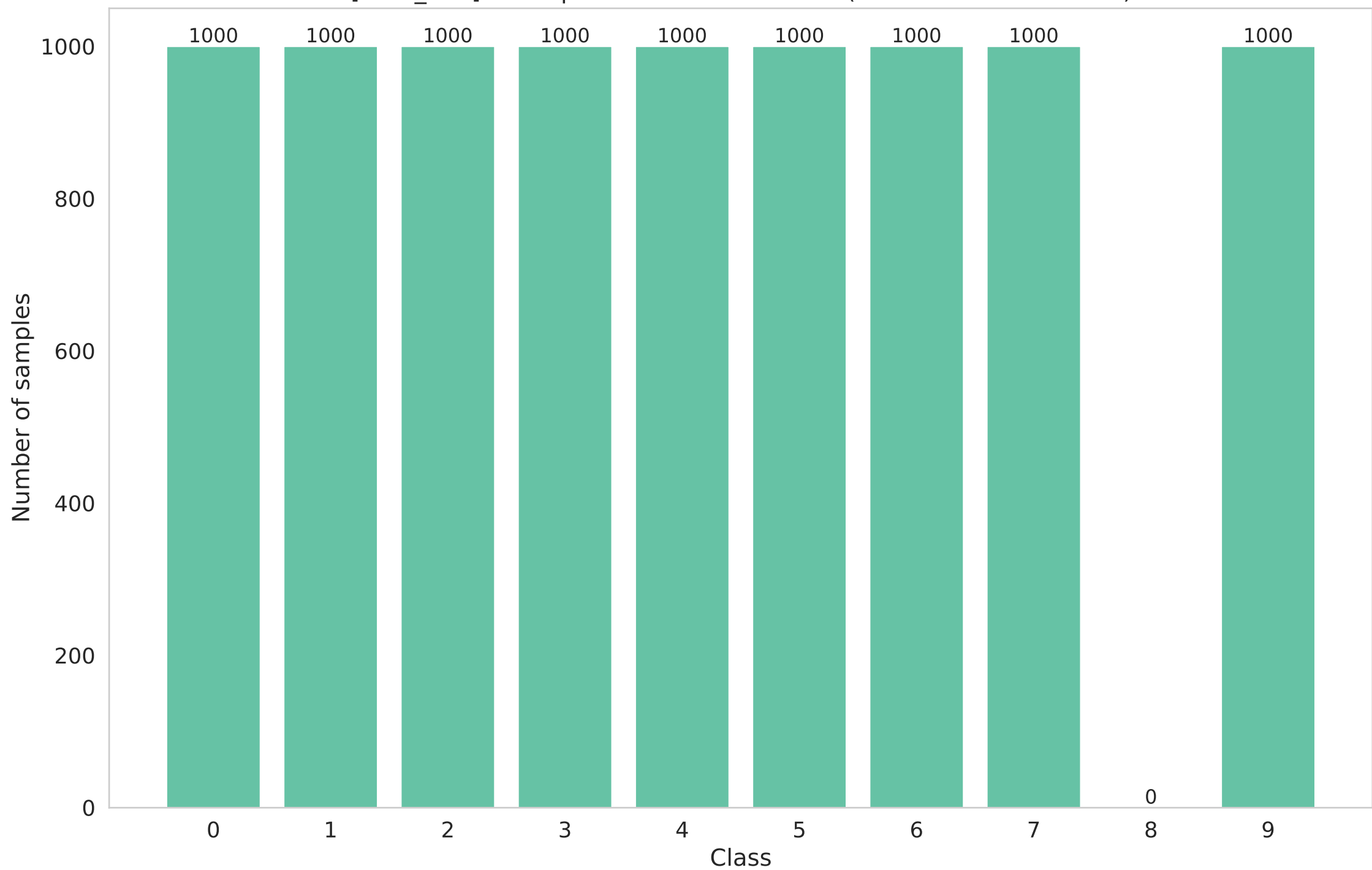
[local_test] Participant 7 data distribution (Non-IID - dirichlet - 0.3)
