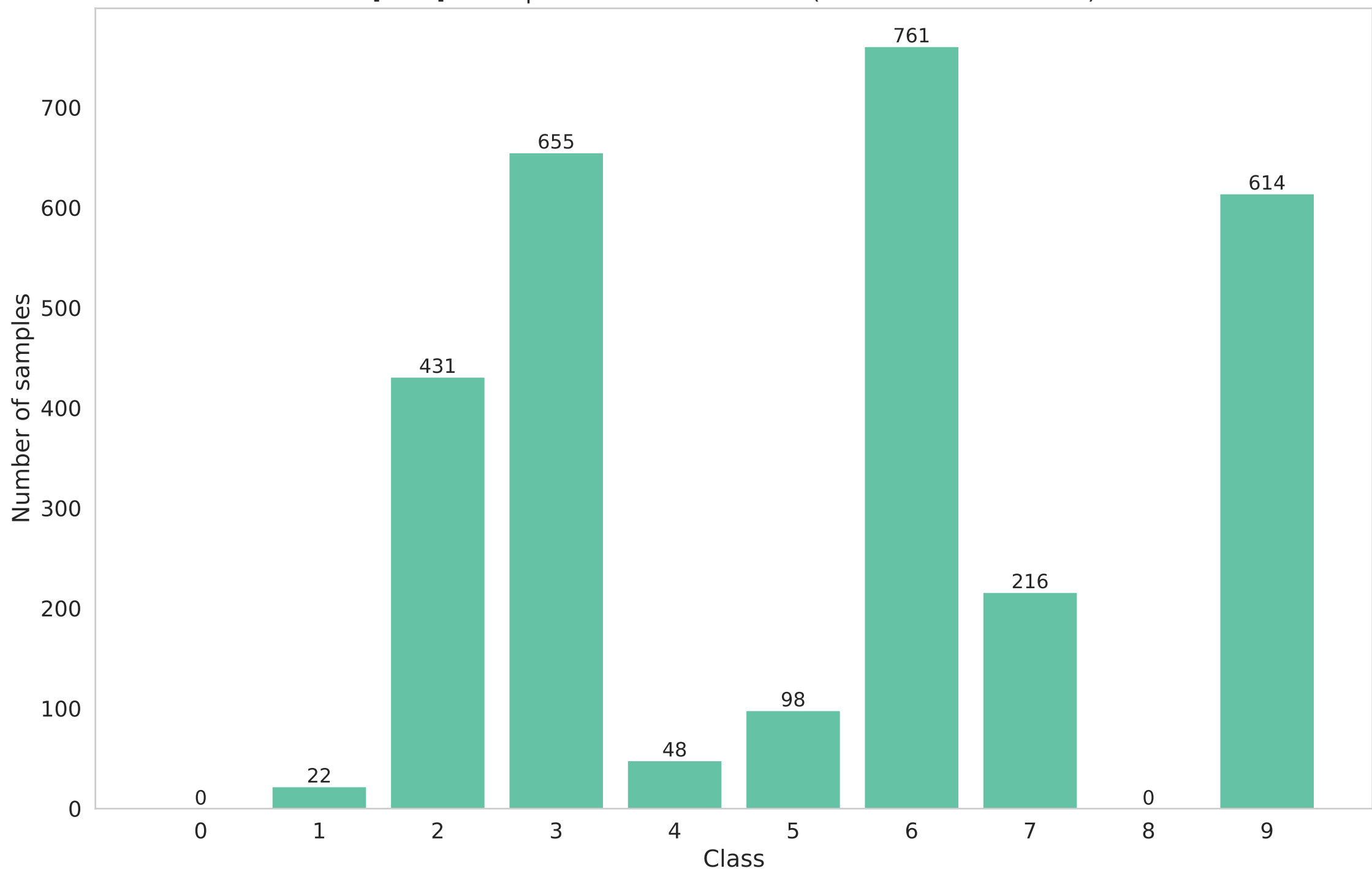
[train] Participant 0 data distribution (Non-IID - dirichlet - 0.3)
