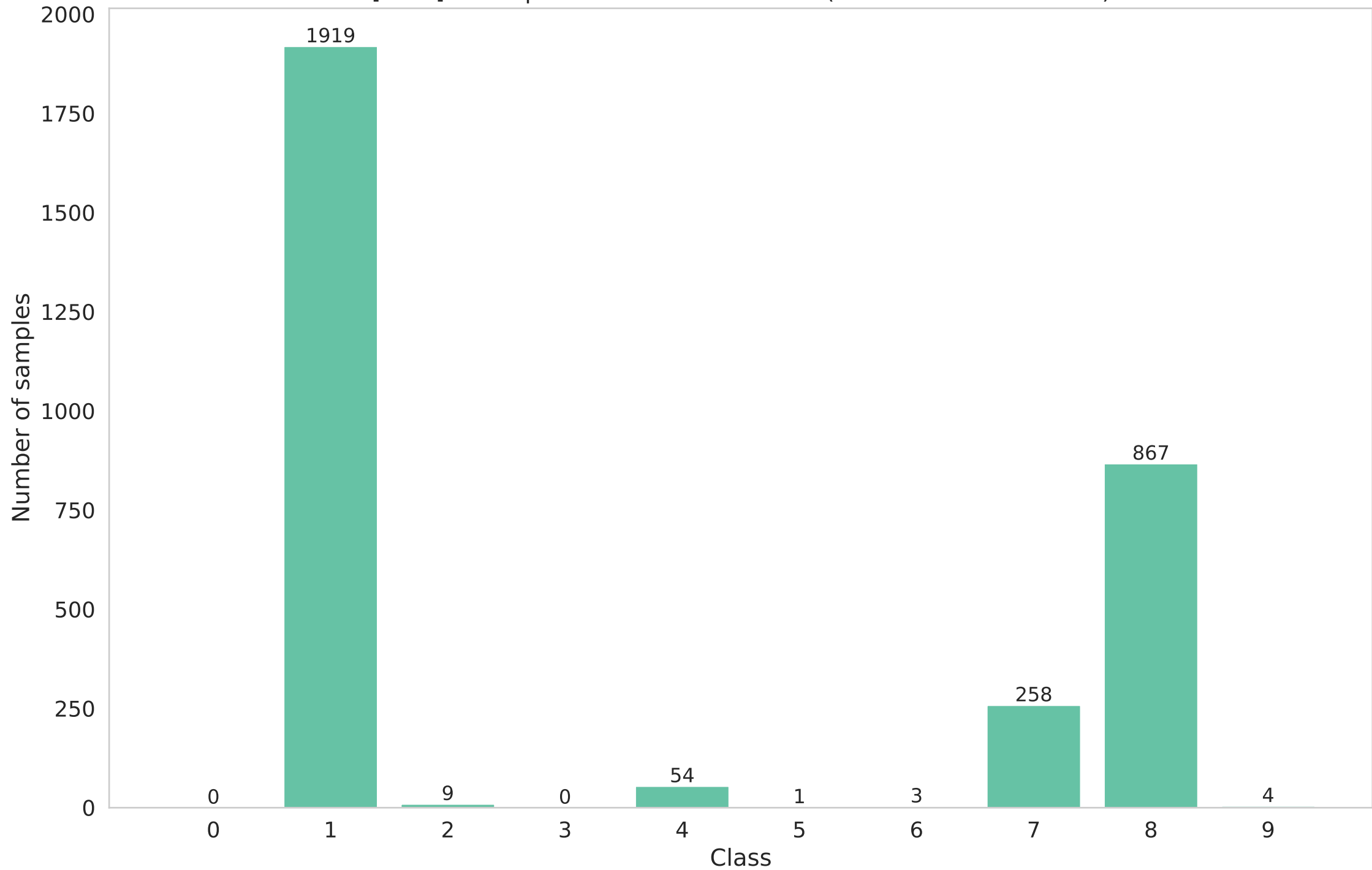
[train] Participant 12 data distribution (Non-IID - dirichlet - 0.1)
