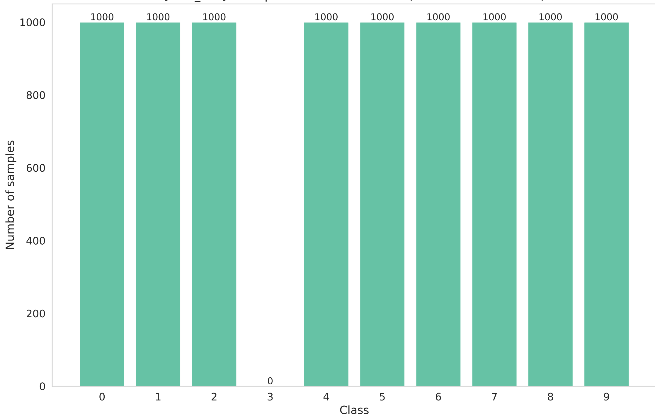
[local_test] Participant 17 data distribution (Non-IID - dirichlet - 0.3)
