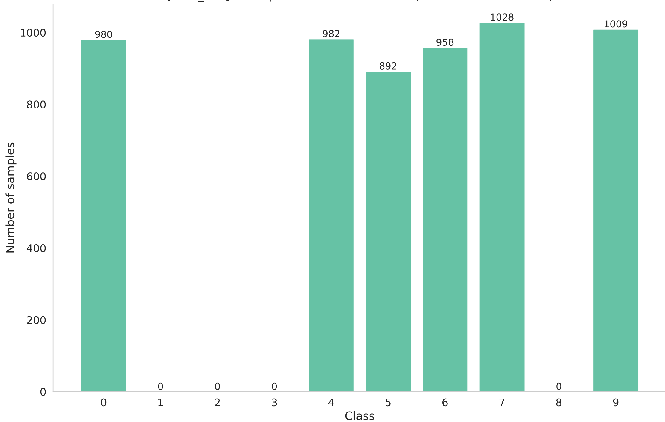
[local_test] Participant 11 data distribution (Non-IID - dirichlet - 0.1)
