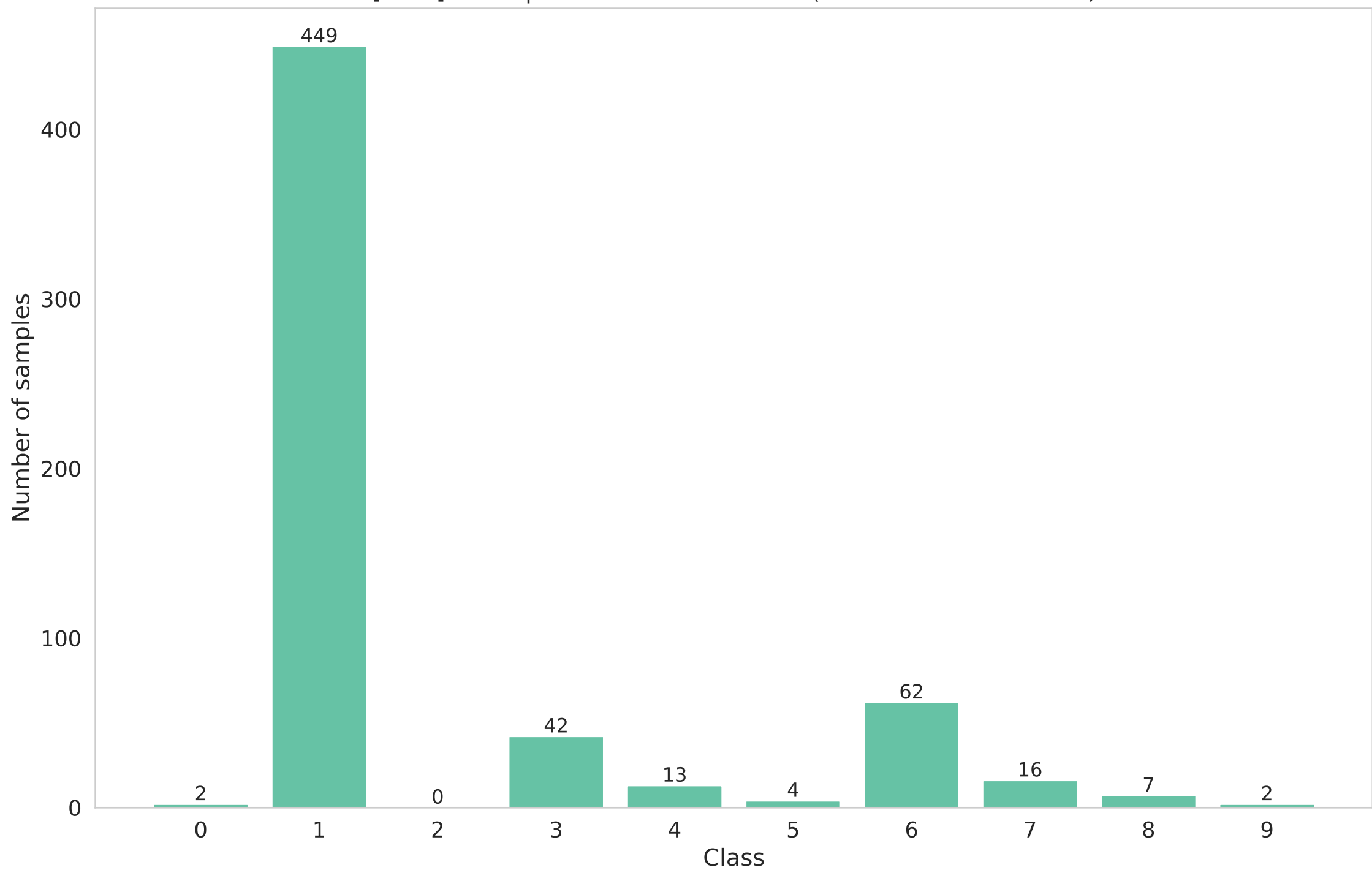
[train] Participant 9 data distribution (Non-IID - dirichlet - 0.3)
