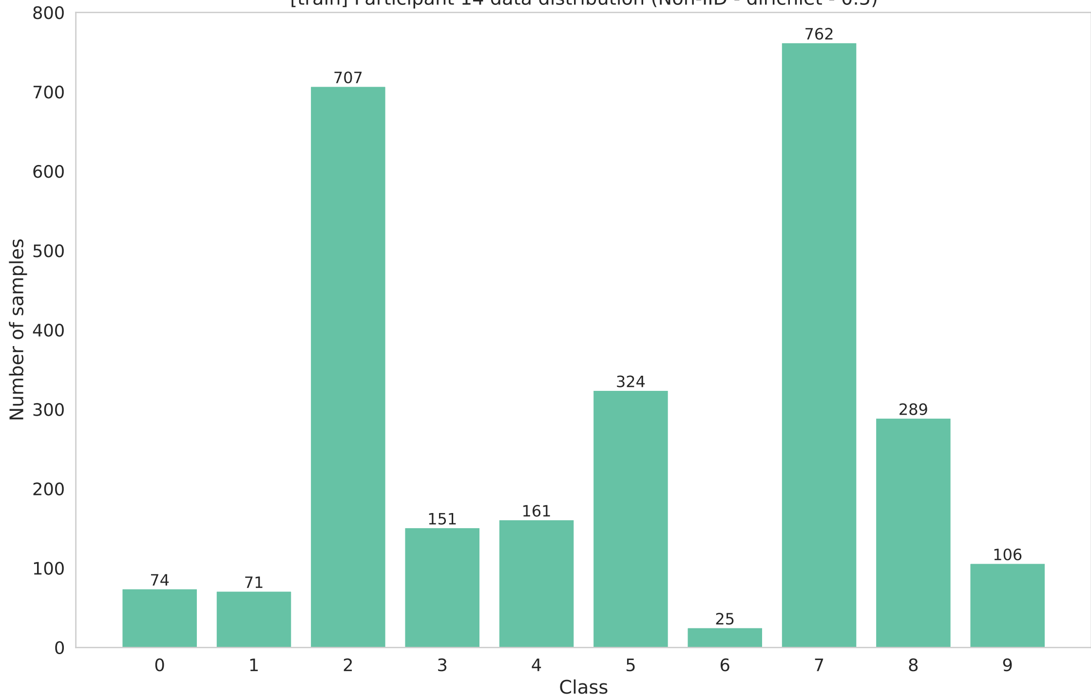
[train] Participant 14 data distribution (Non-IID - dirichlet - 0.5)
