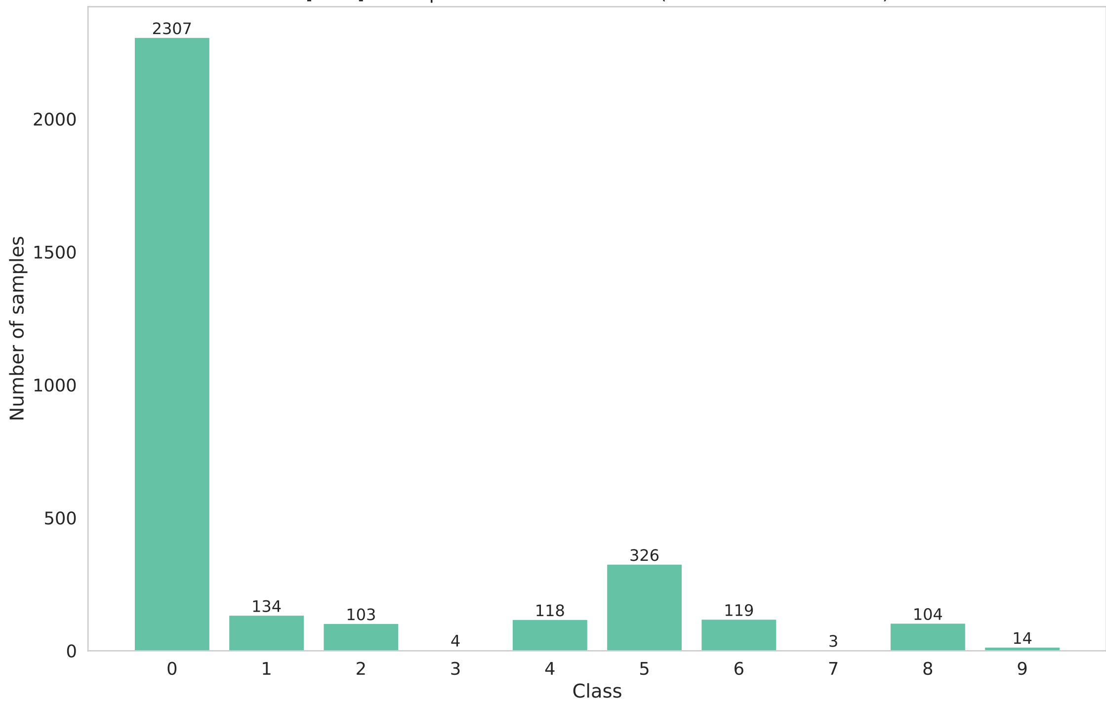
[train] Participant 4 data distribution (Non-IID - dirichlet - 0.5)
