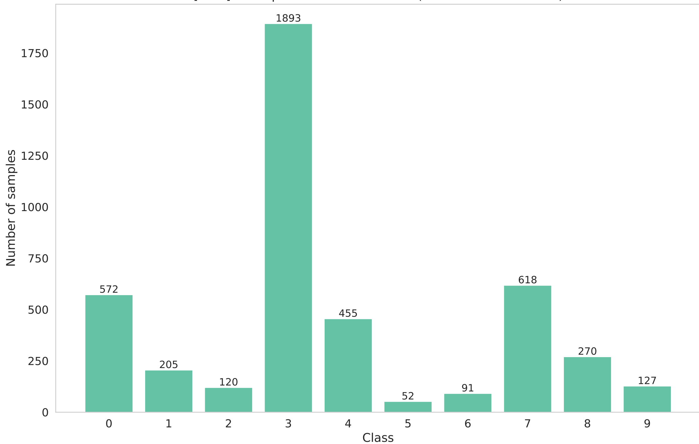
[train] Participant 2 data distribution (Non-IID - dirichlet - 0.5)
