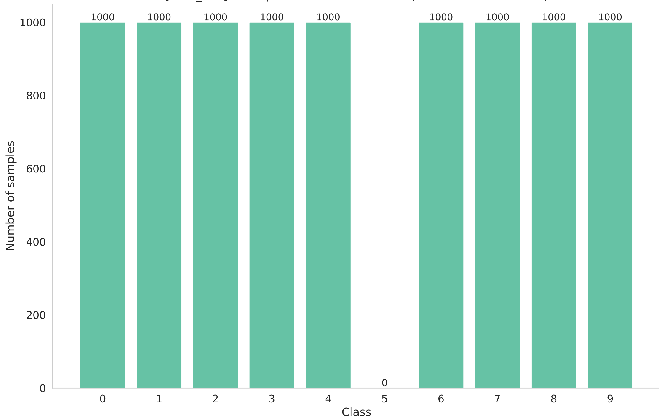
[local_test] Participant 12 data distribution (Non-IID - dirichlet - 0.3)
