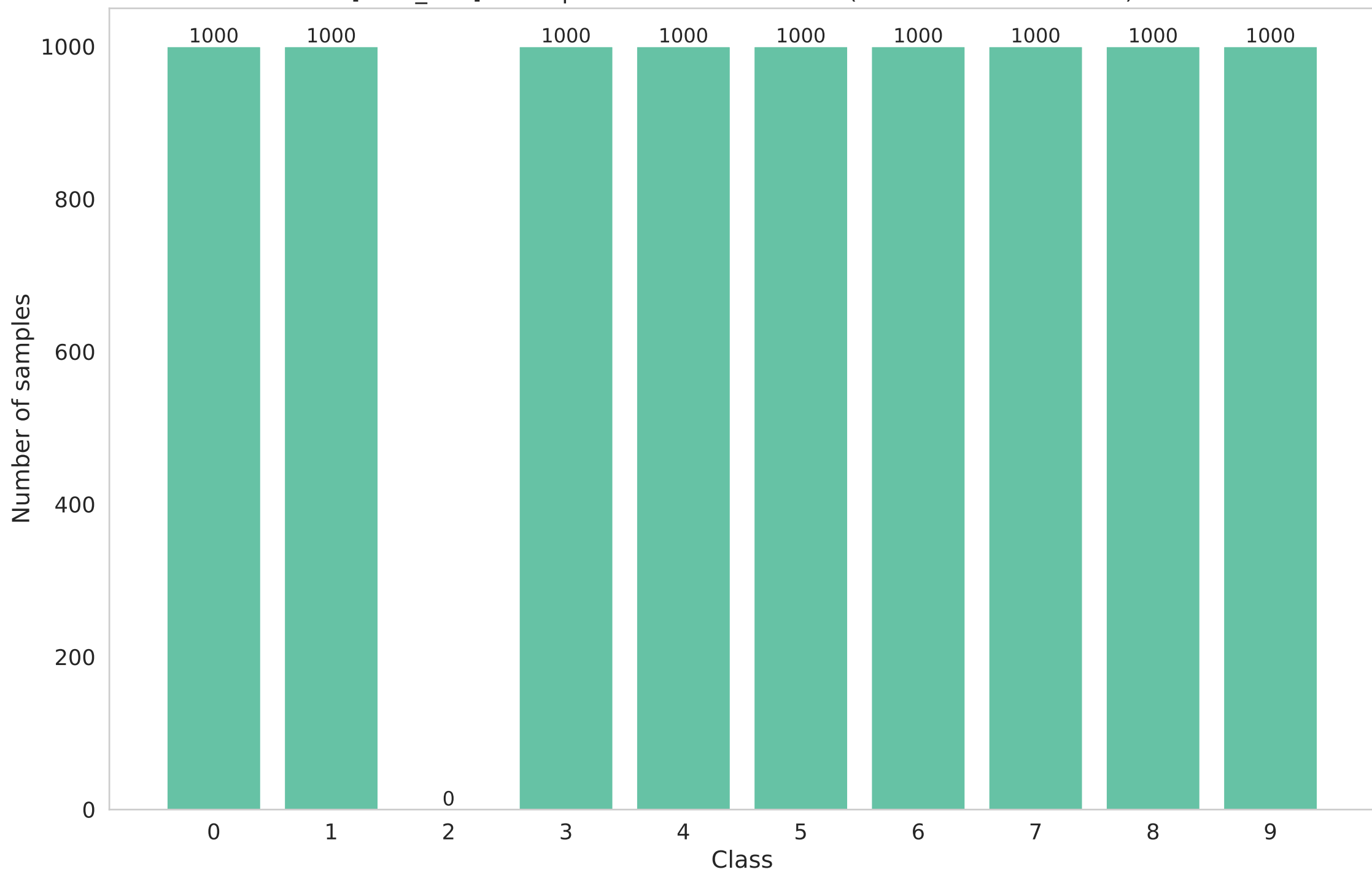
[local_test] Participant 9 data distribution (Non-IID - dirichlet - 0.3)
