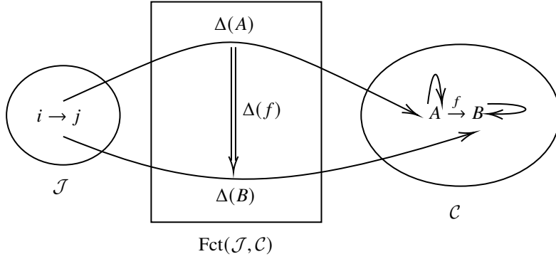
Figure 8.2: 对角函子图释
