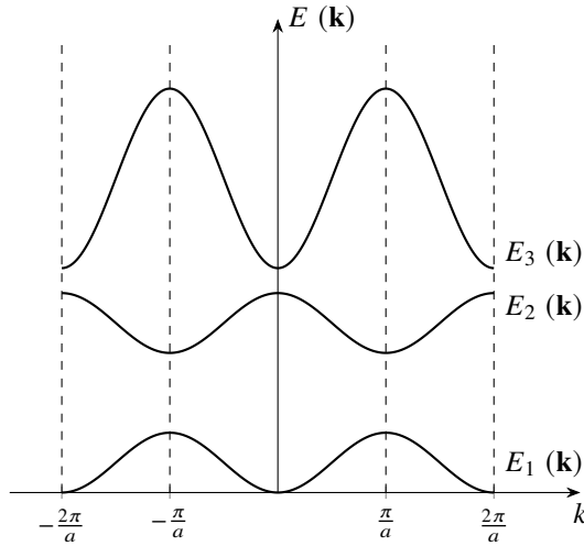
Figure C.1: 一维晶体能带示意图
