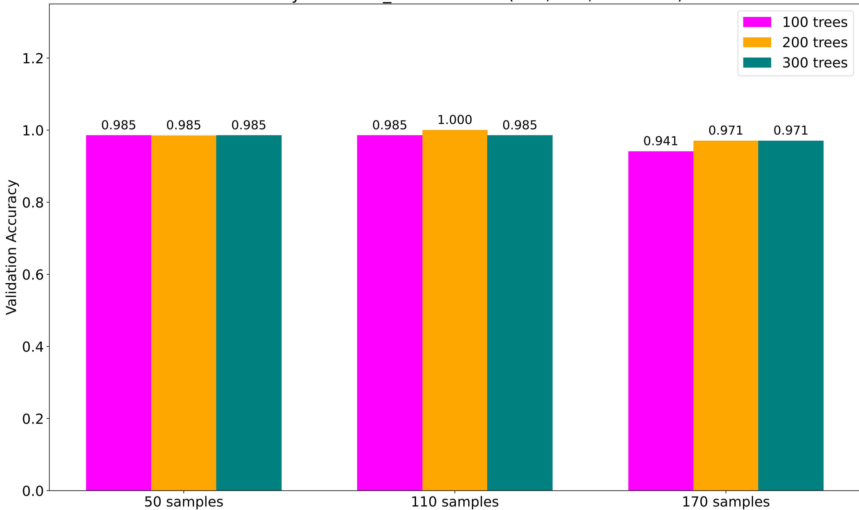
Accuracy with max_features='all' (100, 200, 300 trees)
