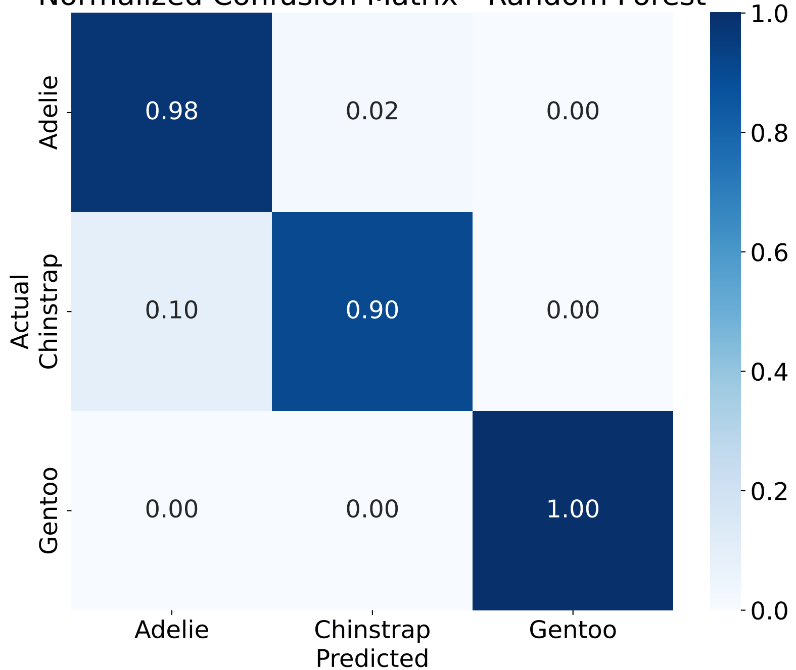
Normalized Confusion Matrix - Random Forest
