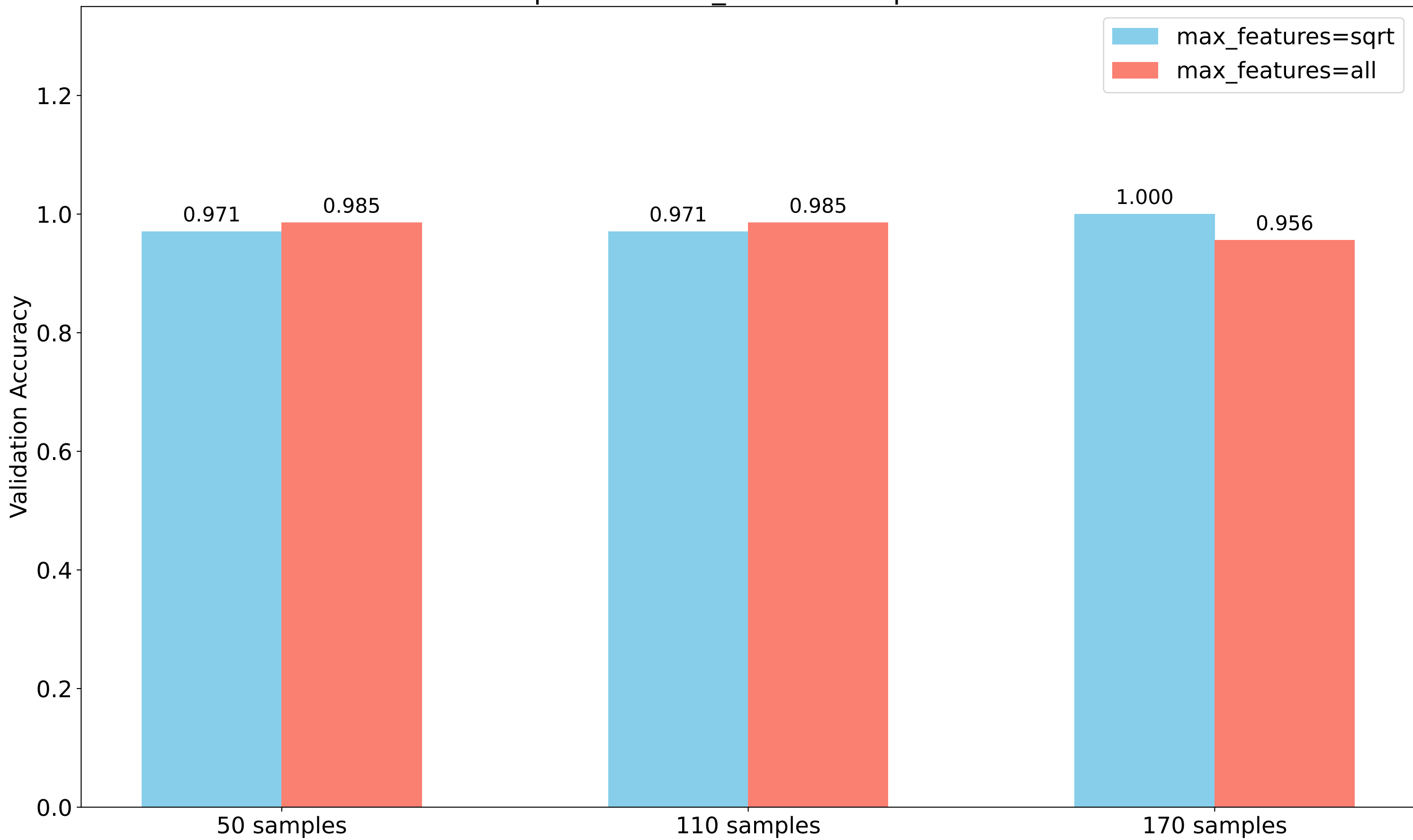
Comparison: max_features='sqrt' vs 'all'
