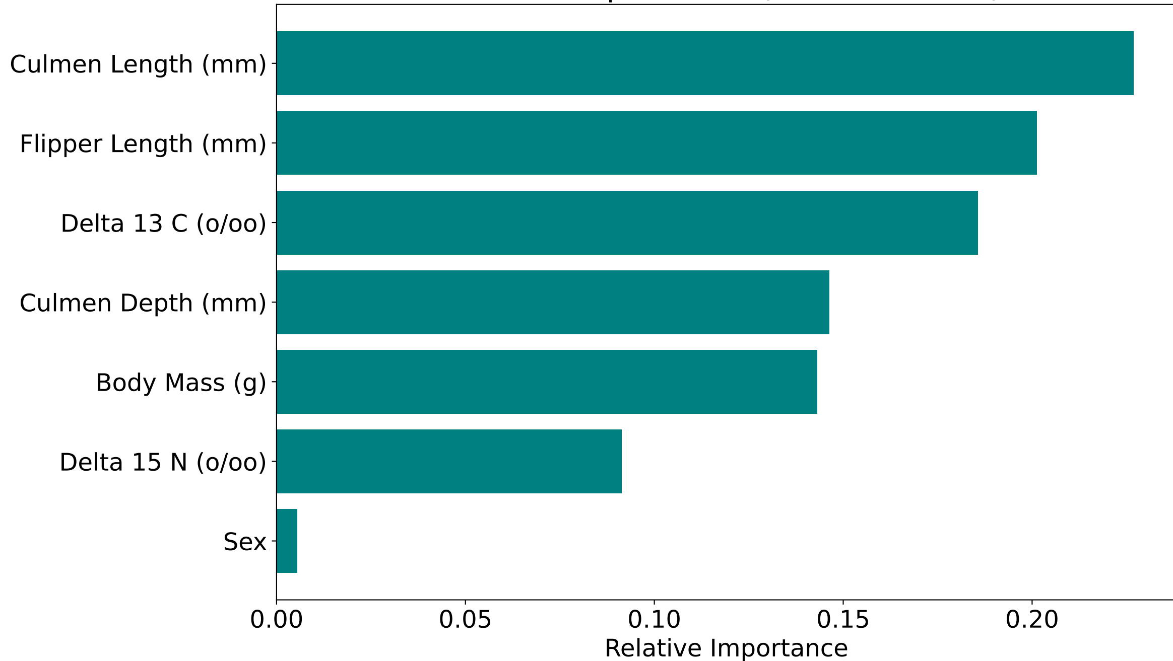
Feature Importances (Random Forest)
