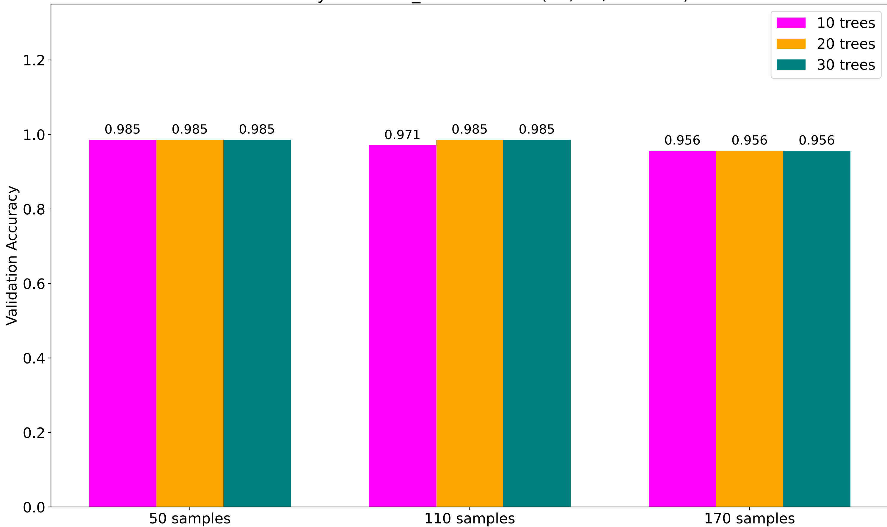
Accuracy with max_features='all' (10, 20, 30 trees)
