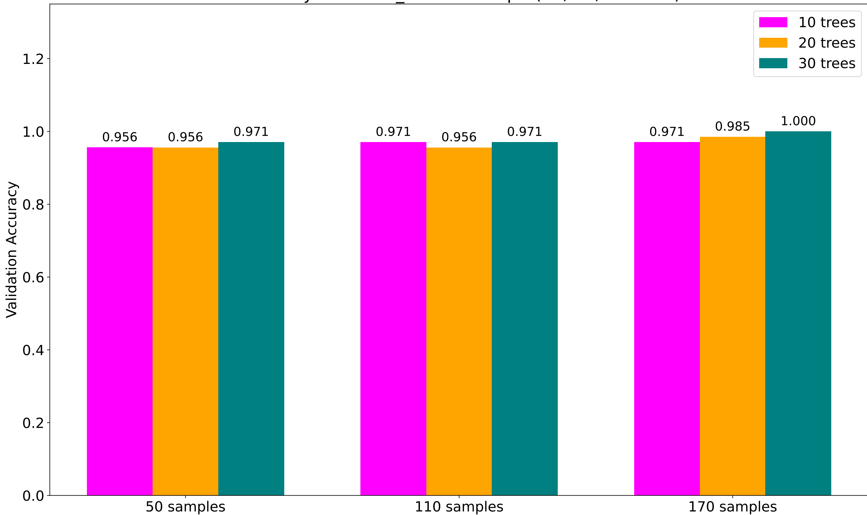
Accuracy with max_features='sqrt' (10, 20, 30 trees)
