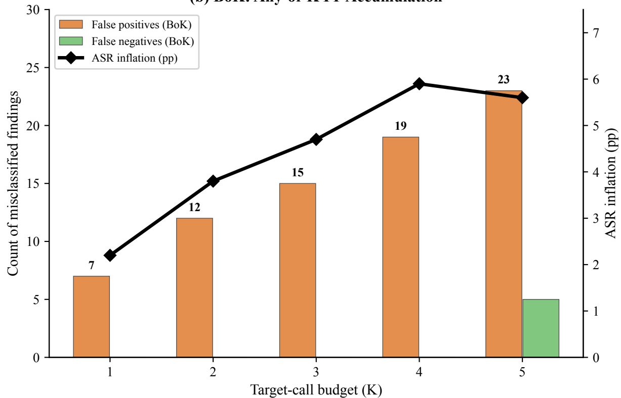
(b) BoK: Any-of-K FP Accumulation
