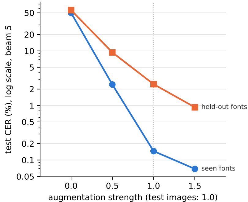
RQ3: augmentation strength
