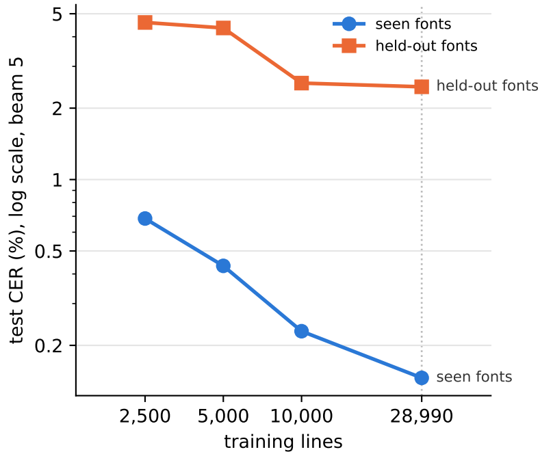
RQ3: amount of training data
