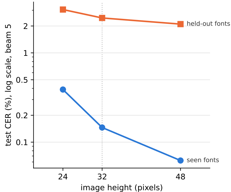
RQ4: image height
