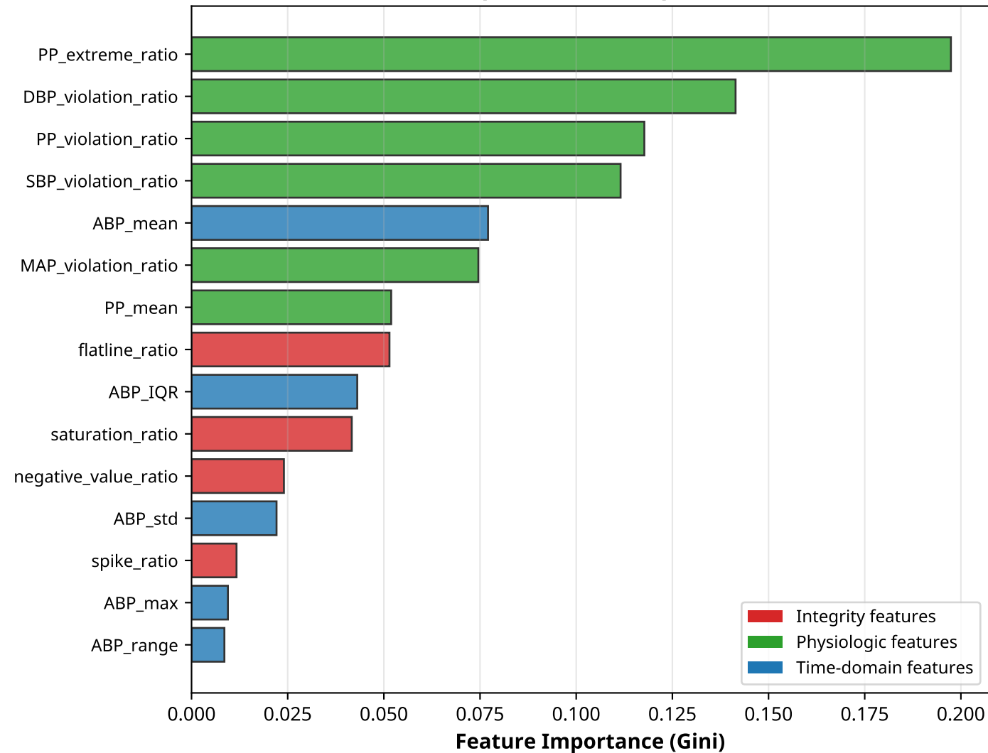
(A) Top-15 Feature Importance
