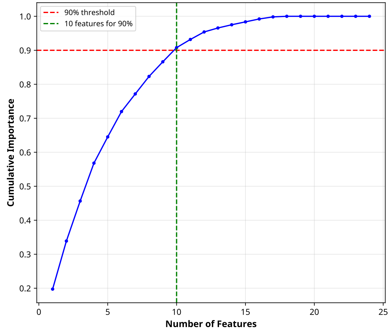
(B) Cumulative Feature Importance
