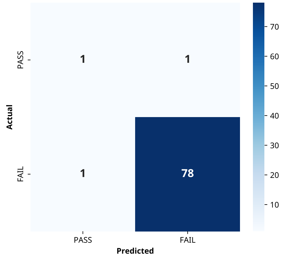
(C) RF Confusion Matrix
