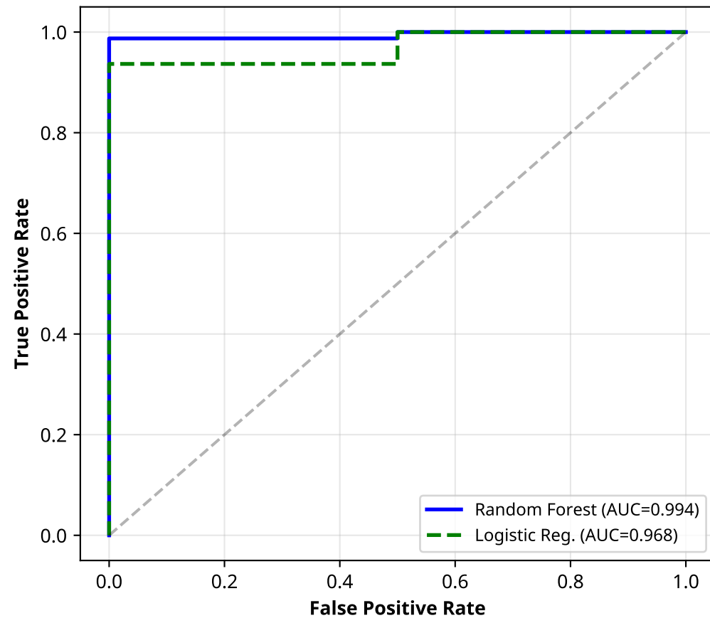
(A) ROC Curves
