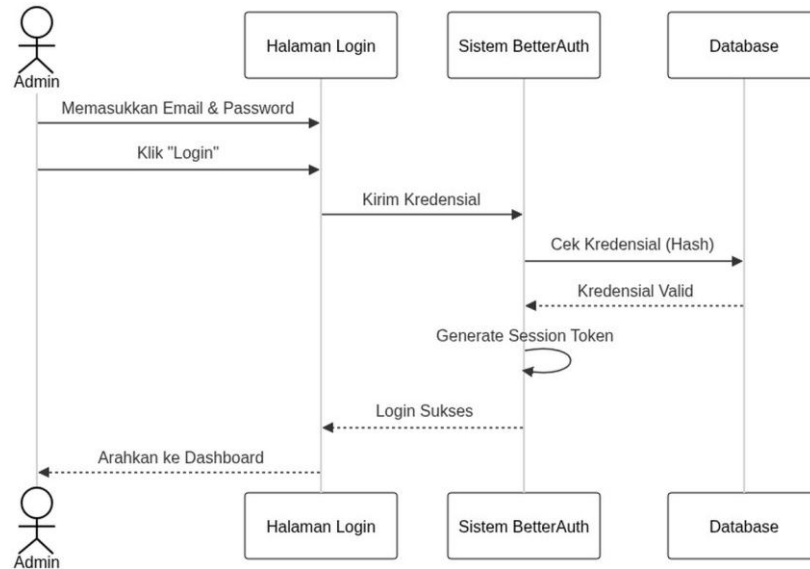
Gambar 3.9 Sequence Diagram Login (Admin)
