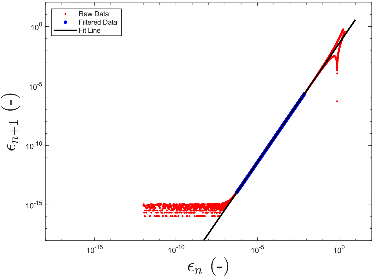
Netwon's Method - Error Data with Fit
