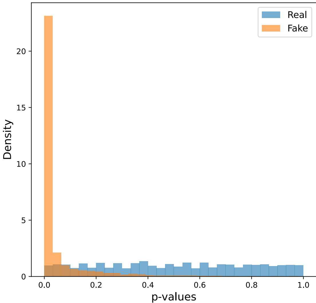
P-values on GAUGAN (after)
