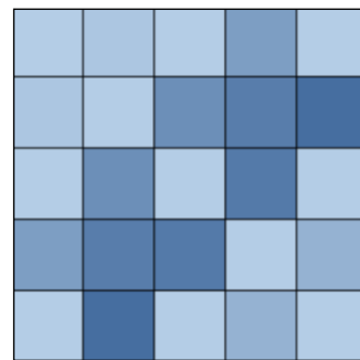
c) Independence Graph Construction
