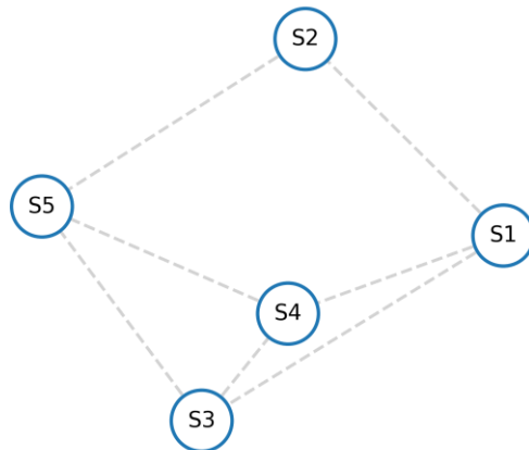
c) Independence Graph Construction
