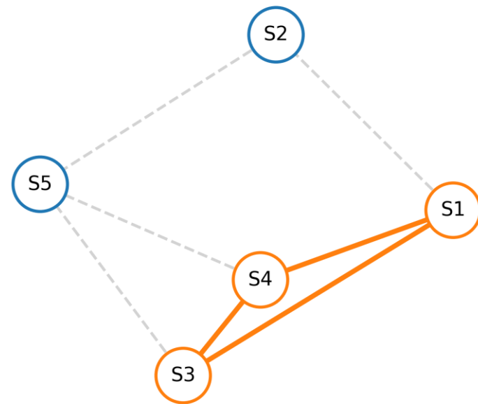
d) Maximum Independent Clique
