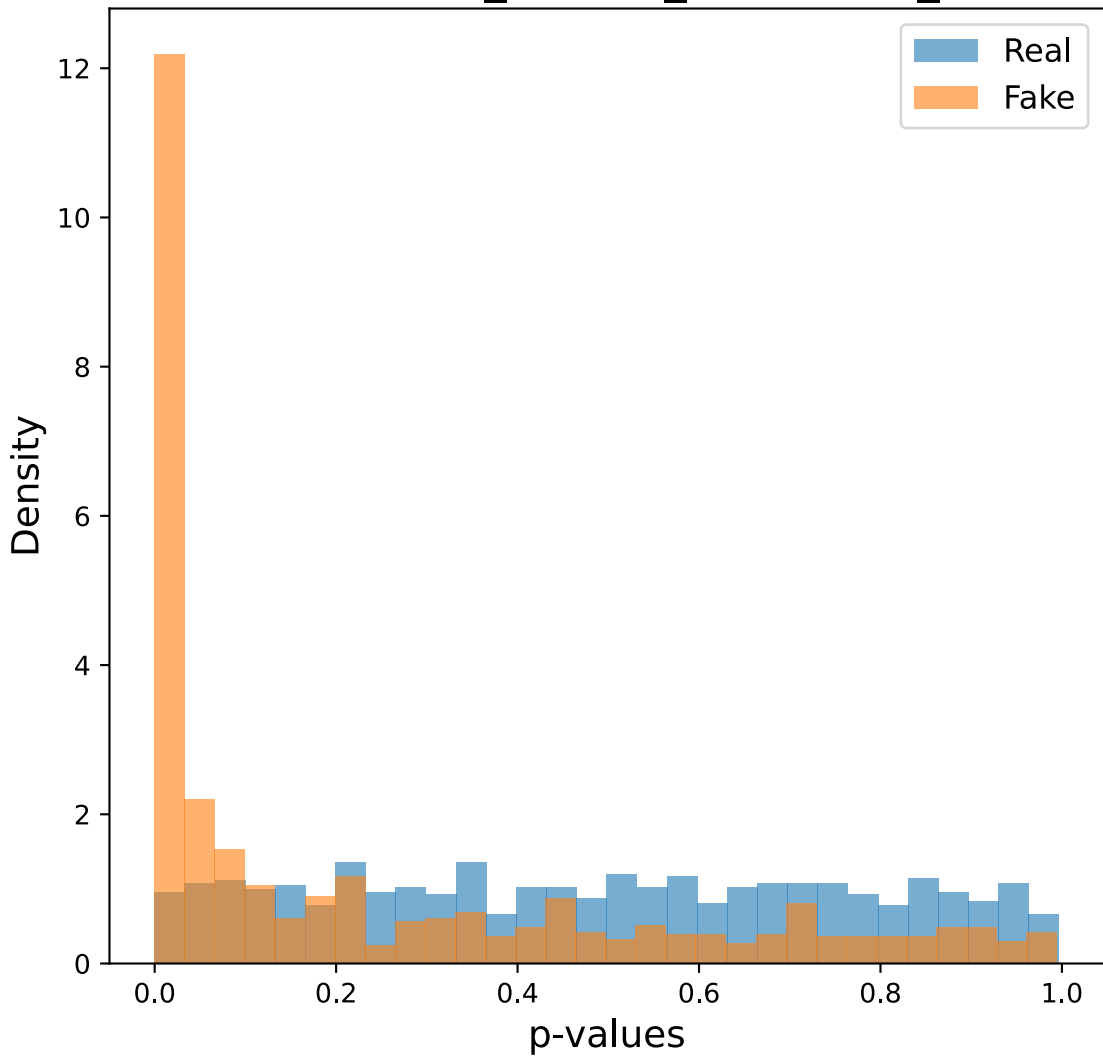
P-values on COCO_STABLE_DIFFUSION_2 (after)
