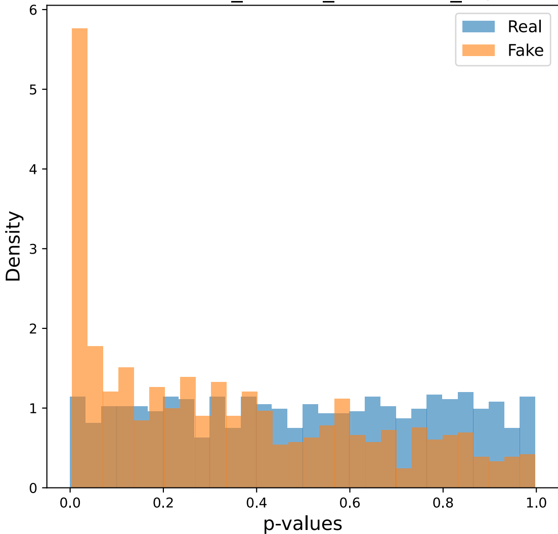
P-values on COCO_STABLE_DIFFUSION_2 (before)
