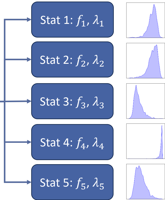
a) Real Empirical Distribution
